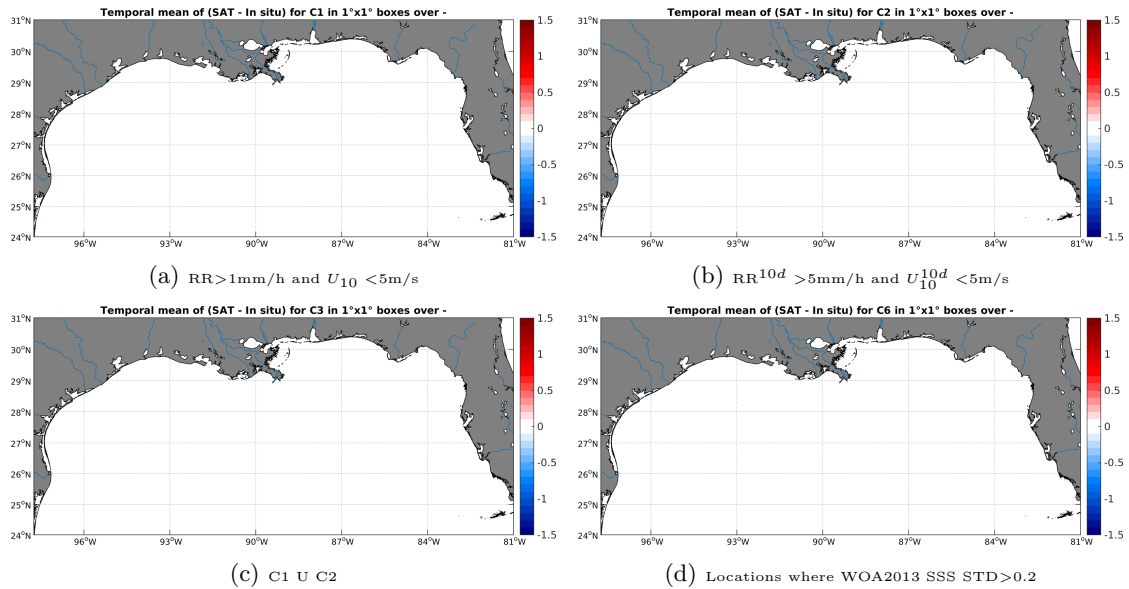
Figure 11: Temporal mean gridded over spatial boxes of size 1^\circ \times 1^\circ of \Delta SSS (SMAP-L2-JPL-V4 - Surface drifters) for 4 different subdatasets corresponding to: RR > 1 mm/h and U_{10} < 5 m/s (a), RR 10d > 5 mm/h and U_{10}^{10d} < 5 m/s (b), C1 U C2 (c), Locations where WOA2013 SSS STD > 0.2 (d).
