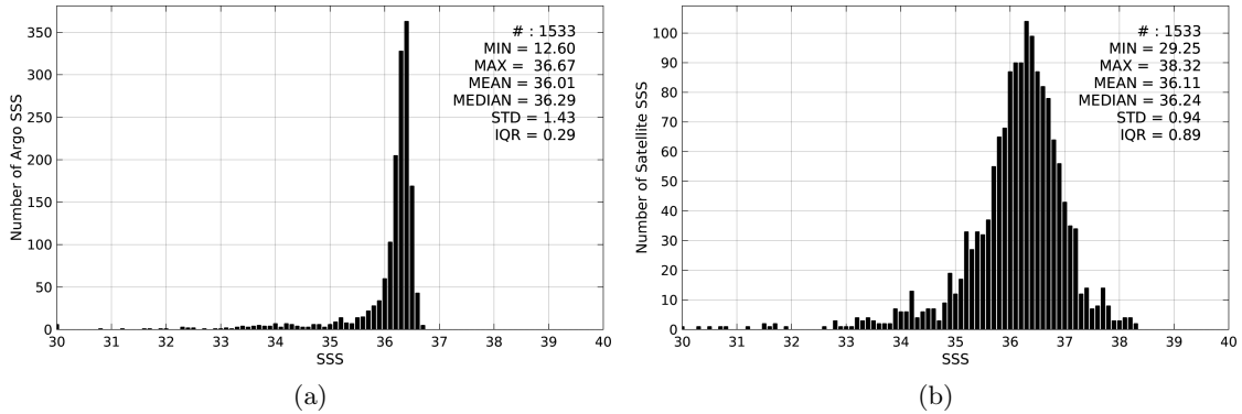
Figure 2: Histograms of SSS from Argo (a) and SMAP-L2-JPL-V4 (b) considering all match-up pairs per bins of 0.1 over the Mississippi river plume Pi-MEP region and for the full satellite product period.
