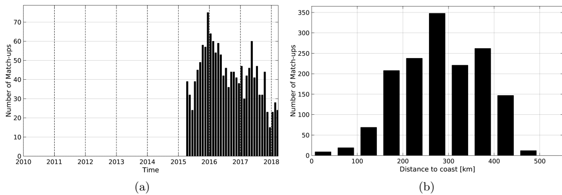
Figure 1: Number of match-ups between Argo and SMAP-L2-JPL-V4 SSS as a function of time (a) and as function of the distance to coast (b) over the Mississippi river plume Pi-MEP region and for the full satellite product period.
