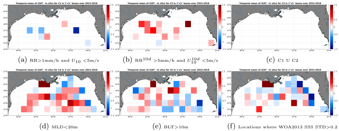
Figure 12: Temporal mean gridded over spatial boxes of size 1^\circ \times 1^\circ of \Delta\text{SSS} (SMAP-L2-JPL-V4 - Argo) for 6 different subdatasets corresponding to: RR > 1\text{mm/h} and U_{10} < 5\text{m/s} (a), RR^{10d} > 5\text{mm/h} and U_{10}^{10d} < 5\text{m/s} (b), C1 U C2 (c), MLD < 20\text{m} (d), BLT > 10\text{m} (e), Locations where WOA2013 SSS STD > 0.2 (f).
