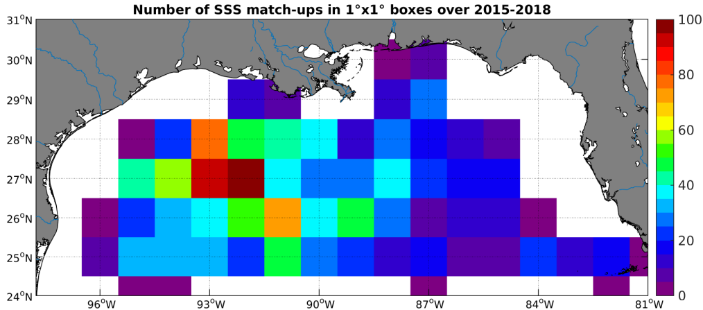
Figure 4: Number of SSS match-ups between Argo SSS and the SMAP-L2-JPL-V4 SSS product for the Mississippi river plume Pi-MEP region over 1^\circ \times 1^\circ boxes and for the full satellite product period.
