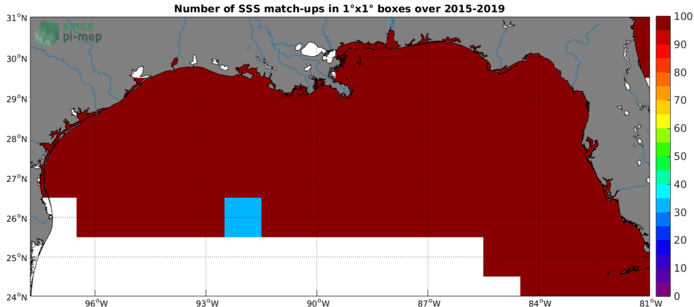
Figure 4: Number of SSS match-ups between TSG-SAMOS SSS and the SMAP-L2-JPL-V4.3 SSS product for the Mississippi river plume Pi-MEP region over 1^\circ \times 1^\circ boxes and for the full satellite product period.
