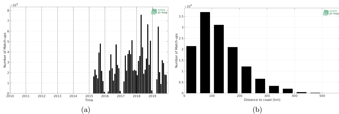
Figure 1: Number of match-ups between TSG-SAMOS and SMAP-L2-JPL-V4.3 SSS as a function of time (a) and as function of the distance to coast (b) over the Mississippi river plume Pi-MEP region and for the full satellite product period.
