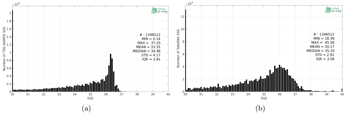
Figure 2: Histograms of SSS from TSG-SAMOS (a) and SMAP-L2-JPL-V4.3 (b) considering all match-up pairs per bins of 0.1 over the Mississippi river plume Pi-MEP region and for the full satellite product period.
