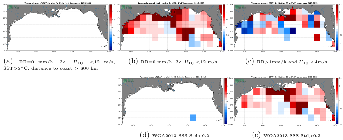
Figure 12: Temporal mean gridded over spatial boxes of size 1^{\circ}\times 1^{\circ} of \Delta\text{SSS} (SMAP-L2-JPL-V4.3 - TSG-SAMOS) for 5 different subdatasets corresponding to:RR=0 mm/h, 3 < U_{10} < 12 m/s, SST > 5^{\circ}\text{C} , distance to coast > 800 km (a), RR=0 mm/h, 3 < U_{10} < 12 m/s (b), RR > 1 mm/h and U_{10} < 4 m/s (c), WOA2013 SSS Std < 0.2 (d), WOA2013 SSS Std > 0.2 (e).
