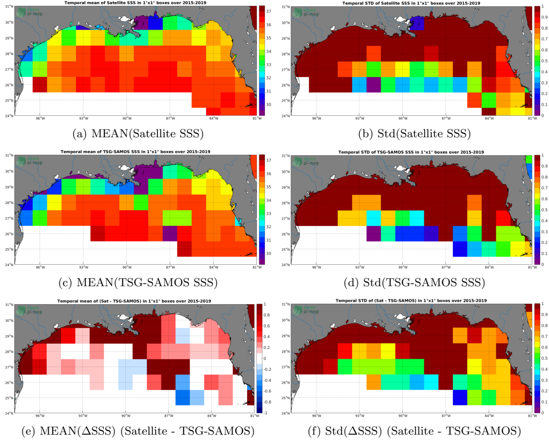
Figure 6: Temporal mean (left) and Std (right) of SSS from SMAP-L2-JPL-V4.3 (top), TSG-SAMOS (middle), and of \Delta SSS (Satellite - TSG-SAMOS). Only match-up pairs are used to generate these maps.
