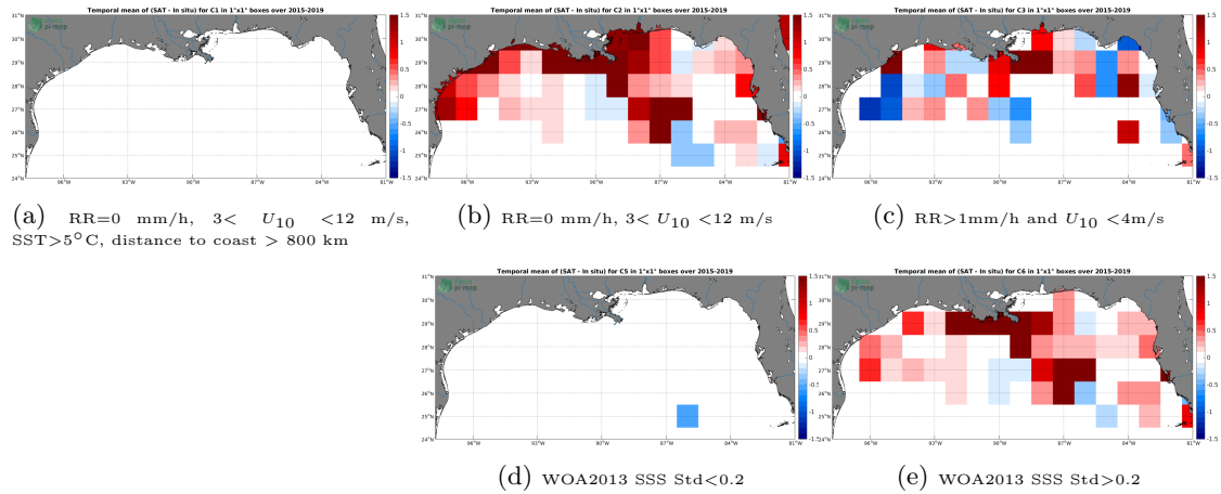
Figure 12: Temporal mean gridded over spatial boxes of size 1^\circ \times 1^\circ of \Delta SSS (SMAP-L2-JPL-V4.3 - TSG-SAMOS) for 5 different subdatasets corresponding to:RR=0 mm/h, 3 < U_{10} < 12 m/s, SST > 5^\circ\text{C} , distance to coast > 800 km (a), RR=0 mm/h, 3 < U_{10} < 12 m/s (b), RR > 1 mm/h and U_{10} < 4 m/s (c), WOA2013 SSS Std < 0.2 (d), WOA2013 SSS Std > 0.2 (e).
