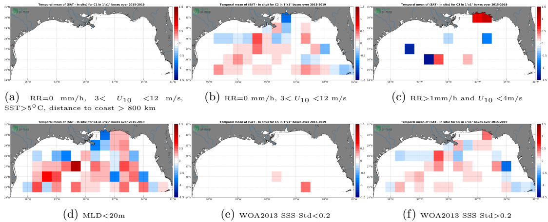
Figure 12: Temporal mean gridded over spatial boxes of size 1^\circ \times 1^\circ of \Delta SSS (SMAP-L2-JPL-V4.3 - Argo) for 6 different subdatasets corresponding to:RR=0 mm/h, 3 < U_{10} < 12 m/s, SST >5^\circ C, distance to coast > 800 km (a), RR=0 mm/h, 3 < U_{10} < 12 m/s (b), RR >1 mm/h and U_{10} < 4 m/s (c),MLD <20 m (d),WOA2013 SSS Std <0.2 (e),WOA2013 SSS Std >0.2 (f).
