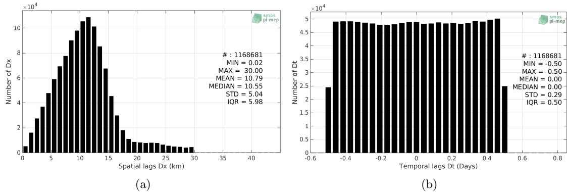
Figure 5: Histograms of the spatial (a) and temporal (b) lags between the time of the TSG-SAMOS measurements and the date of the corresponding SMAP-L2-JPL-V4.2 SSS product.
