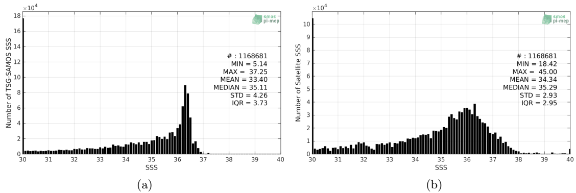
Figure 2: Histograms of SSS from TSG-SAMOS (a) and SMAP-L2-JPL-V4.2 (b) considering all match-up pairs per bins of 0.1 over the Mississippi river plume Pi-MEP region and for the full satellite product period.
