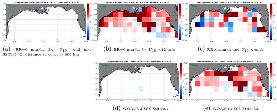
Figure 12: Temporal mean gridded over spatial boxes of size 1^\circ \times 1^\circ of \Delta SSS (SMAP-L2-JPL-V4.2 - TSG-SAMOS) for 5 different subdatasets corresponding to: RR=0 mm/h, 3 < U_{10} < 12 m/s, SST > 5^\circ C, distance to coast > 800 km (a), RR=0 mm/h, 3 < U_{10} < 12 m/s (b), RR > 1 mm/h and U_{10} < 4 m/s (c), WOA2013 SSS Std < 0.2 (d), WOA2013 SSS Std > 0.2 (e).
