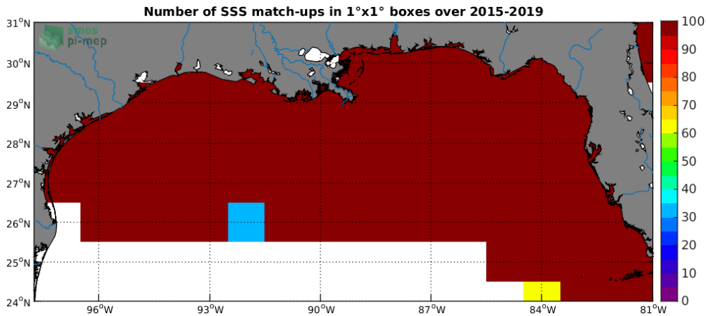
Figure 4: Number of SSS match-ups between TSG-SAMOS SSS and the SMAP-L2-JPL-V4.2 SSS product for the Mississippi river plume Pi-MEP region over 1^\circ \times 1^\circ boxes and for the full satellite product period.
