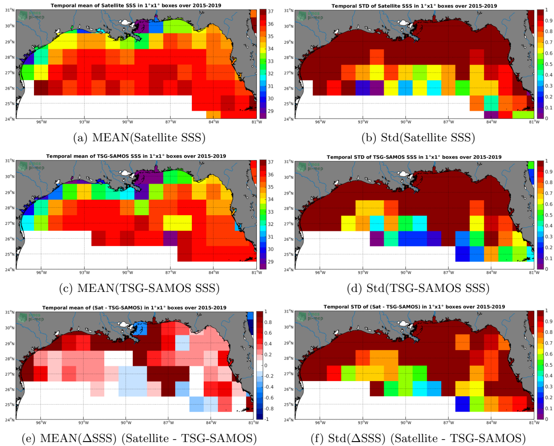
Figure 6: Temporal mean (left) and Std (right) of SSS from SMAP-L2-JPL-V4.2 (top), TSG-SAMOS (middle), and of \Delta SSS (Satellite - TSG-SAMOS). Only match-up pairs are used to generate these maps.
