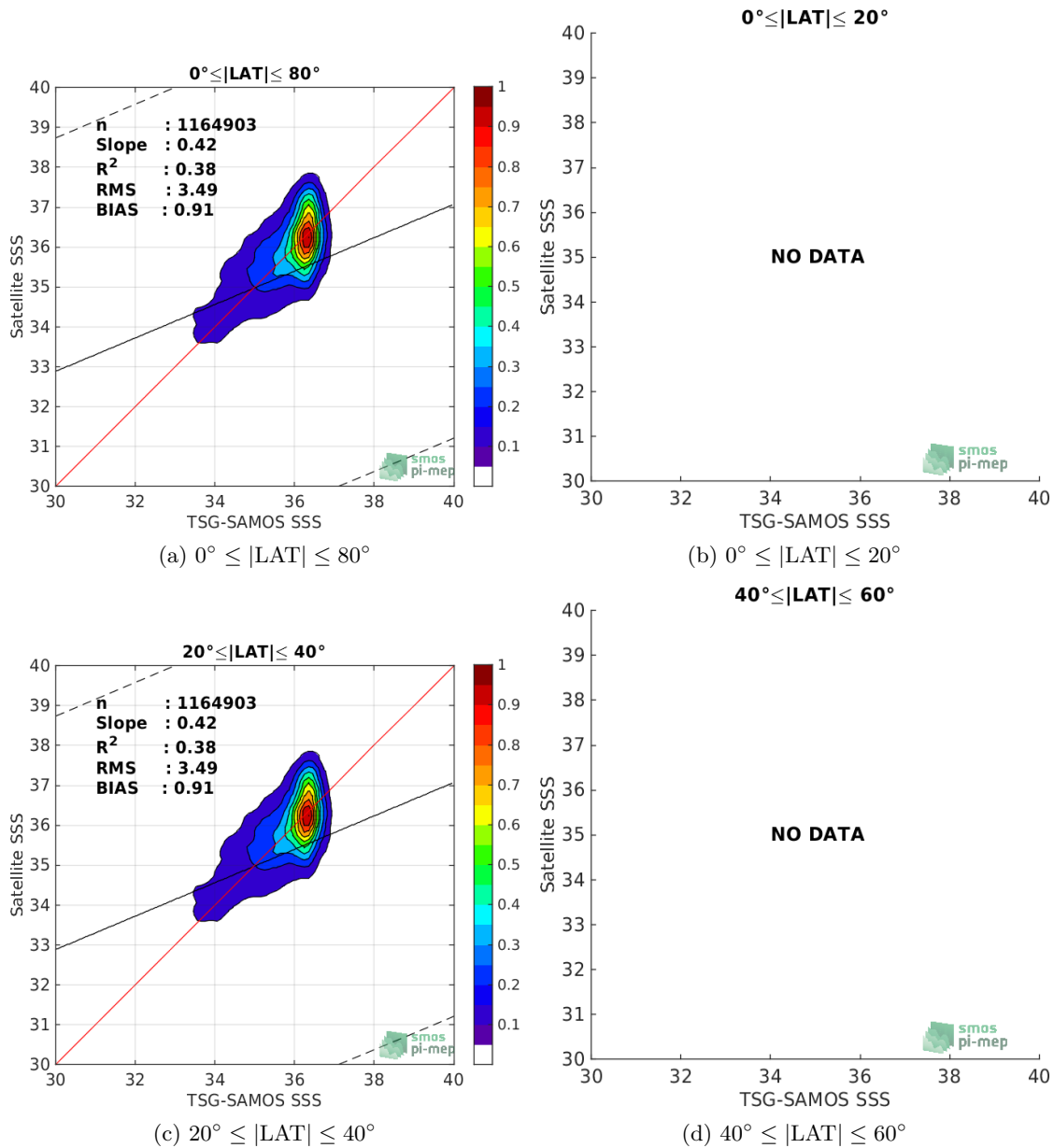
Figure 9: Contour maps of the concentration of SMAP-L2-JPL-V4.2 SSS (y-axis) versus TSG-SAMOS SSS (x-axis) at match-up pairs for different latitude bands. For each plot, the red line shows x=y . The black thin and dashed lines indicate a linear fit through the data cloud and the \pm 95\% confidence levels, respectively. The number match-up pairs n , the slope and R^2 coefficient of the linear fit, the root mean square (RMS) and the mean bias between satellite and in situ data are indicated for each latitude band in each plots.
