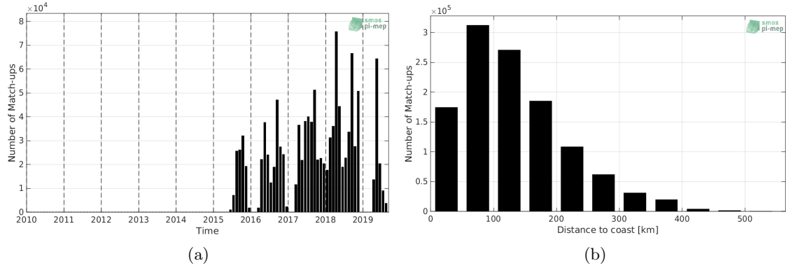
Figure 1: Number of match-ups between TSG-SAMOS and SMAP-L2-JPL-V4.2 SSS as a function of time (a) and as function of the distance to coast (b) over the Mississippi river plume Pi-MEP region and for the full satellite product period.
