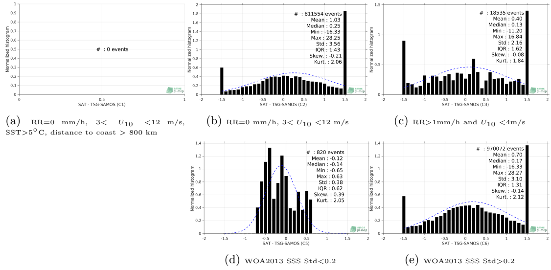
Figure 13: Normalized histogram of \Delta SSS (SMAP-L2-JPL-V4.2 - TSG-SAMOS) for 5 different subdatasets corresponding to: RR=0 mm/h, 3 < U_{10} < 12 m/s, SST>5°C, distance to coast > 800 km (a), RR=0 mm/h, 3 < U_{10} < 12 m/s (b), RR>1mm/h and U_{10} < 4 m/s (c), WOA2013 SSS Std<0.2 (d), WOA2013 SSS Std>0.2 (e).
