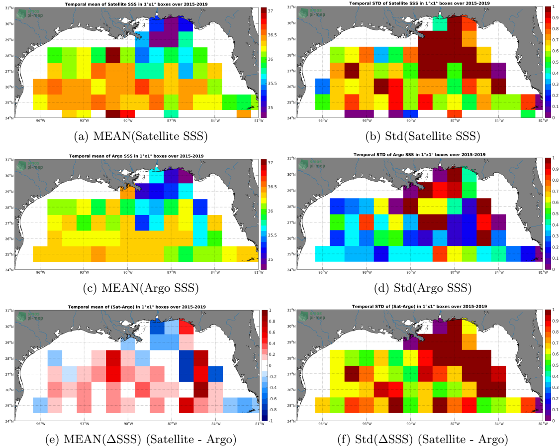
Figure 6: Temporal mean (left) and Std (right) of SSS from SMAP-L2-JPL-V4.2 (top), Argo (middle), and of \Delta SSS (Satellite - Argo). Only match-up pairs are used to generate these maps.
