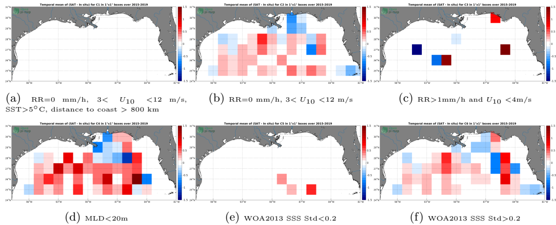
Figure 12: Temporal mean gridded over spatial boxes of size 1^\circ \times 1^\circ of \Delta SSS (SMAP-L2-JPL-V4.2 - Argo) for 6 different subdatasets corresponding to: RR=0 mm/h, 3 < U_{10} < 12 m/s, SST > 5^\circ C , distance to coast > 800 km (a), RR=0 mm/h, 3 < U_{10} < 12 m/s (b), RR > 1 mm/h and U_{10} < 4 m/s (c), MLD < 20 m (d), WOA2013 SSS Std < 0.2 (e), WOA2013 SSS Std > 0.2 (f).
