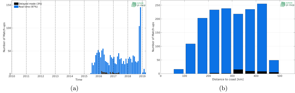
Figure 1: Number of match-ups between Argo and SMAP-L2-JPL-V4.2 SSS as a function of time (a) and as function of the distance to coast (b) over the Mississippi river plume Pi-MEP region and for the full satellite product period.
