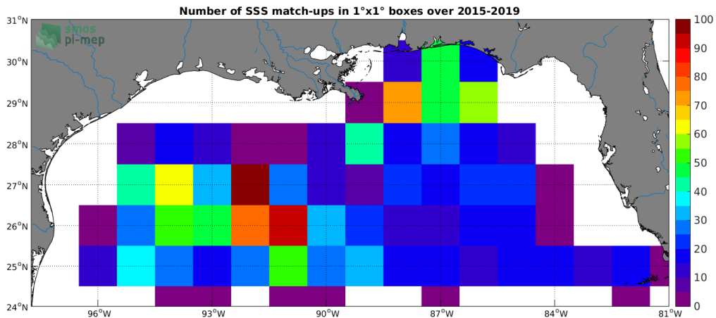
Figure 4: Number of SSS match-ups between Argo SSS and the SMAP-L2-JPL-V4.2 SSS product for the Mississippi river plume Pi-MEP region over 1^\circ \times 1^\circ boxes and for the full satellite product period.
