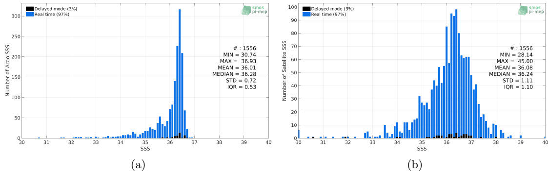
Figure 2: Histograms of SSS from Argo (a) and SMAP-L2-JPL-V4.2 (b) considering all match-up pairs per bins of 0.1 over the Mississippi river plume Pi-MEP region and for the full satellite product period.
