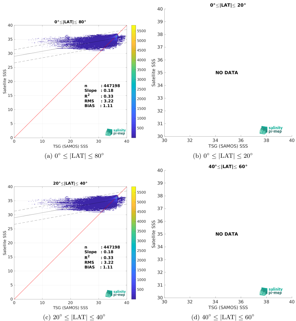
Figure 10: Contour maps of the concentration of ISAS v7 - Monthly (Ifremer-LOPS-CMEMS) SSS (y-axis) versus TSG (SAMOS) SSS (x-axis) at match-up pairs for different latitude bands. For each plot, the red line shows x=y . The black thin and dashed lines indicate a linear fit through the data cloud and the \pm 95\% confidence levels, respectively. The number match-up pairs n , the slope and R^2 coefficient of the linear fit, the root mean square (RMS) and the mean bias between satellite and in situ data are indicated for each latitude band in each plot.
