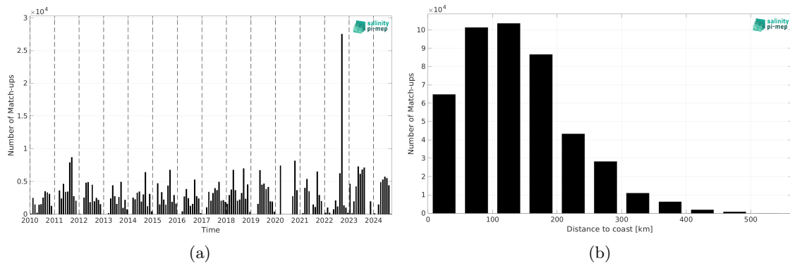
Figure 2: Number of match-ups between TSG (SAMOS) and ISAS v7 - Monthly (Ifremer-LOPS-CMEMS) SSS as a function of time (a) and as function of the distance to coast (b) over the Mississippi river plume Pi-MEP region and for the full satellite product period.
