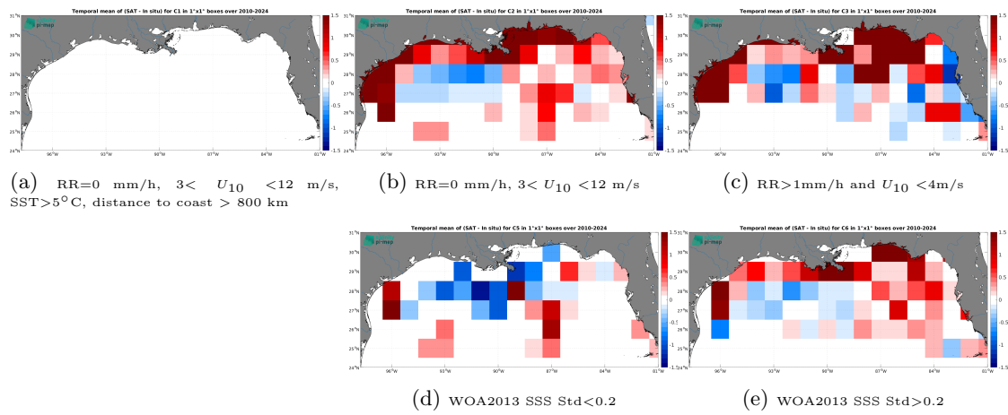
Figure 14: Temporal mean gridded over spatial boxes of size 1^\circ \times 1^\circ of \Delta SSS (ISAS v7 - Monthly (Ifremer-LOPS-CMEMS) - TSG (SAMOS)) for 5 different subdatasets corresponding to:RR=0 mm/h, 3 < U_{10} < 12 m/s, SST > 5°C, distance to coast > 800 km (a), RR=0 mm/h, 3 < U_{10} < 12 m/s (b), RR > 1mm/h and U_{10} < 4 m/s (c), WOA2013 SSS Std < 0.2 (d), WOA2013 SSS Std > 0.2 (e).
