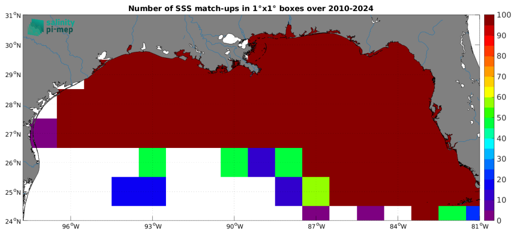
Figure 5: Number of SSS match-ups between TSG (SAMOS) SSS and the ISAS v7 - Monthly (Ifremer-LOPS-CMEMS) SSS product for the Mississippi river plume Pi-MEP region over 1^\circ \times 1^\circ boxes and for the full satellite product period.
