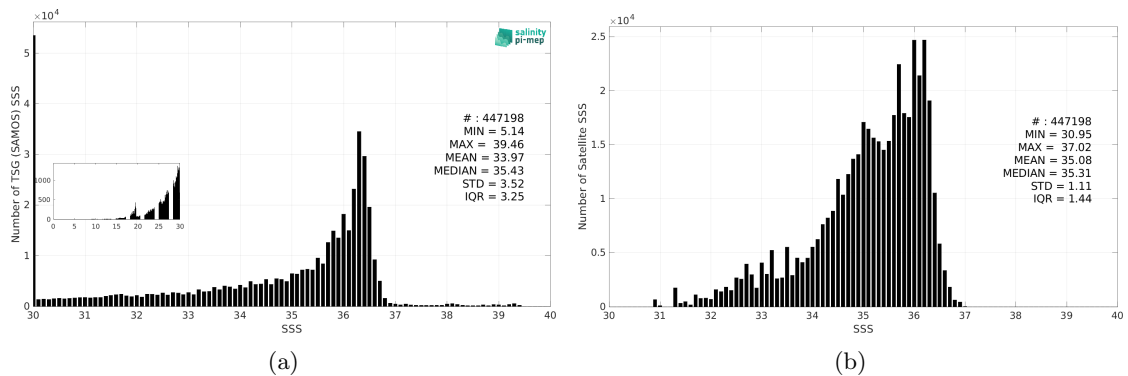
Figure 3: Histograms of SSS from TSG (SAMOS) (a) and ISAS v7 - Monthly (Ifremer-LOPS-CMEMS) (b) considering all match-up pairs per bins of 0.1 over the Mississippi river plume Pi-MEP region and for the full satellite product period.
