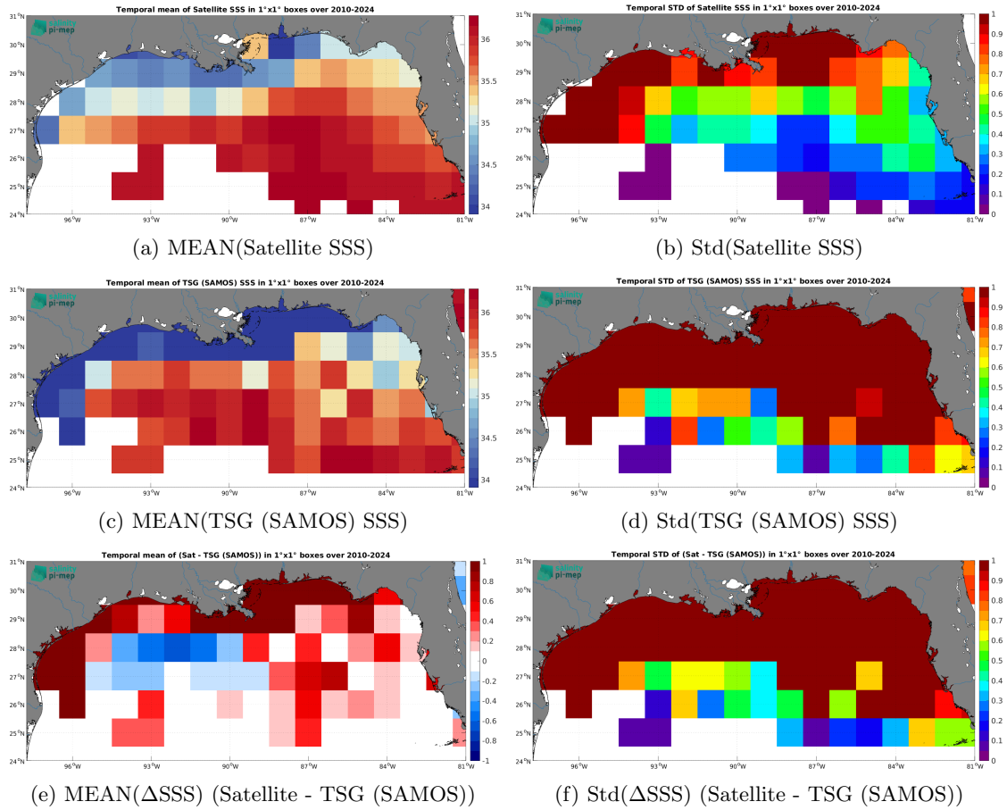
Figure 7: Temporal mean (left) and Std (right) of SSS from ISAS v7 - Monthly (Ifremer-LOPS-CMEMS) (top), TSG (SAMOS) (middle), and of \Delta SSS (Satellite - TSG (SAMOS)). Only match-up pairs are used to generate these maps.
