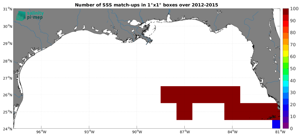
Figure 5: Number of SSS match-ups between TSG (GOSUD-Sailing-ship) SSS and the ISAS v7 - Monthly (Ifremer-LOPS-CMEMS) SSS product for the Mississippi river plume Pi-MEP region over 1^\circ \times 1^\circ boxes and for the full satellite product period.
