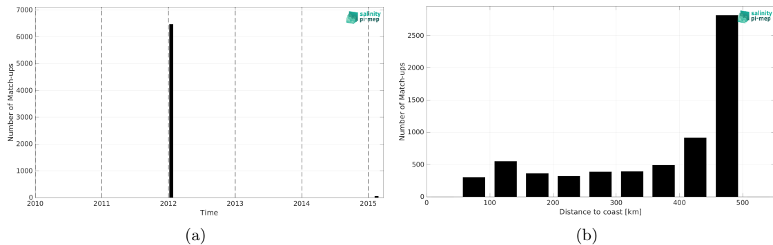
Figure 2: Number of match-ups between TSG (GOSUD-Sailing-ship) and ISAS v7 - Monthly (Ifremer-LOPS-CMEMS) SSS as a function of time (a) and as function of the distance to coast (b) over the Mississippi river plume Pi-MEP region and for the full satellite product period.
