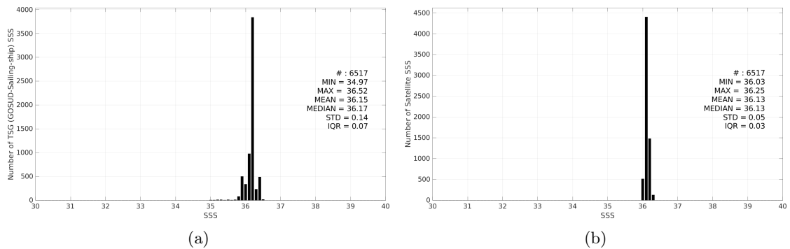
Figure 3: Histograms of SSS from TSG (GOSUD-Sailing-ship) (a) and ISAS v7 - Monthly (Ifremer-LOPS-CMEMS) (b) considering all match-up pairs per bins of 0.1 over the Mississippi river plume Pi-MEP region and for the full satellite product period.
