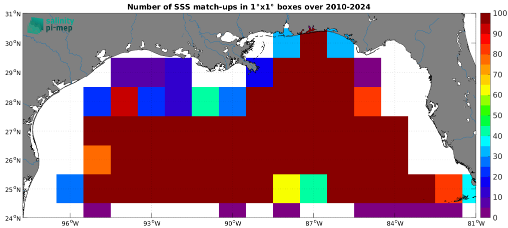
Figure 5: Number of SSS match-ups between Argo SSS and the ISAS v7 - Monthly (Ifremer-LOPS-CMEMS) SSS product for the Mississippi river plume Pi-MEP region over 1^\circ \times 1^\circ boxes and for the full satellite product period.
