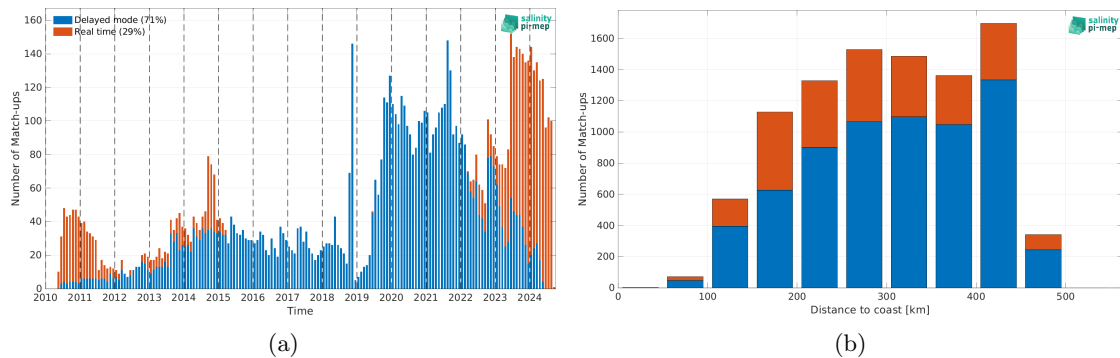
Figure 2: Number of match-ups between Argo and ISAS v7 - Monthly (Ifremer-LOPS-CMEMS) SSS as a function of time (a) and as function of the distance to coast (b) over the Mississippi river plume Pi-MEP region and for the full satellite product period.
