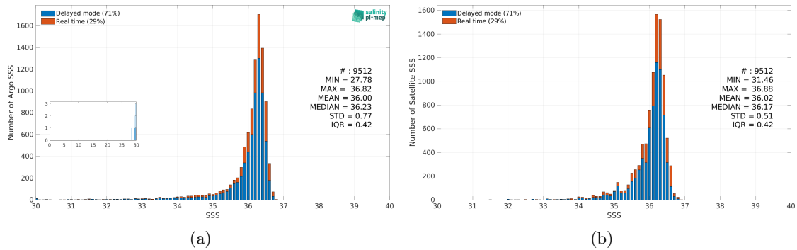
Figure 3: Histograms of SSS from Argo (a) and ISAS v7 - Monthly (Ifremer-LOPS-CMEMS) (b) considering all match-up pairs per bins of 0.1 over the Mississippi river plume Pi-MEP region and for the full satellite product period.
