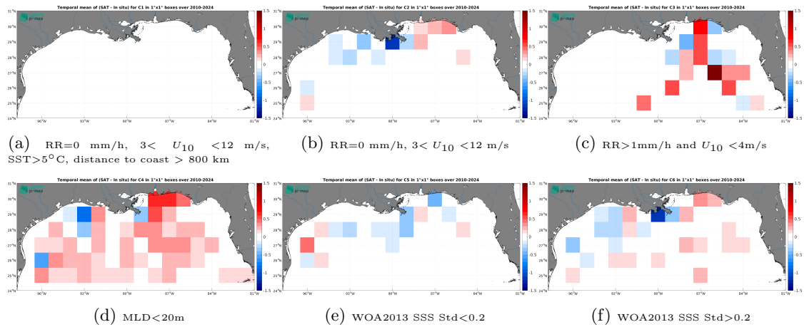
Figure 14: Temporal mean gridded over spatial boxes of size 1^\circ \times 1^\circ of \Delta SSS (ISAS v7 - Monthly (Ifremer-LOPS-CMEMS) - Argo) for 6 different subdatasets corresponding to:RR=0 mm/h, 3 < U_{10} < 12 m/s, SST >5^\circ\text{C} , distance to coast > 800 km (a), RR=0 mm/h, 3 < U_{10} < 12 m/s (b), RR >1 mm/h and U_{10} < 4 m/s (c),MLD <20 m (d),WOA2013 SSS Std <0.2 (e),WOA2013 SSS Std >0.2 (f).
