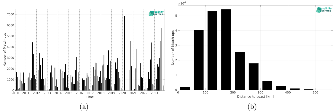
Figure 2: Number of match-ups between TSG (SAMOS) and CCI SSS L4 Merged-OI v5.5 - 7-day running (ESA) SSS as a function of time (a) and as function of the distance to coast (b) over the Mississippi river plume Pi-MEP region and for the full satellite product period.
