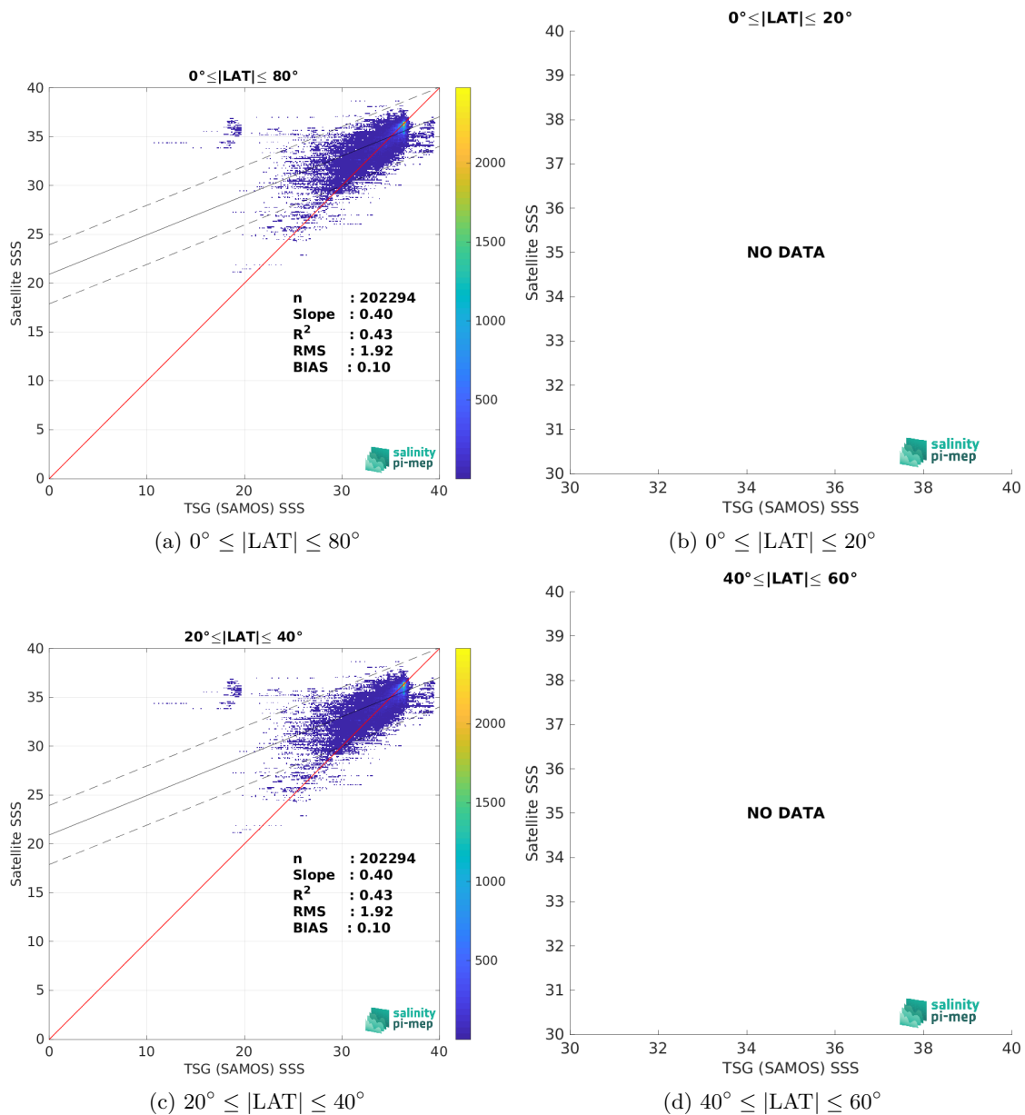
Figure 10: Contour maps of the concentration of CCI SSS L4 Merged-OI v5.5 - 7-day running (ESA) SSS (y-axis) versus TSG (SAMOS) SSS (x-axis) at match-up pairs for different latitude bands. For each plot, the red line shows x=y . The black thin and dashed lines indicate a linear fit through the data cloud and the \pm 95\% confidence levels, respectively. The number match-up pairs n , the slope and R^2 coefficient of the linear fit, the root mean square (RMS) and the mean bias between satellite and in situ data are indicated for each latitude band in each plots.
