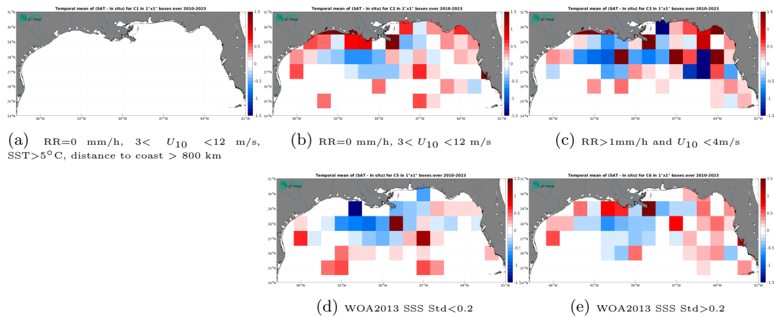
Figure 14: Temporal mean gridded over spatial boxes of size 1^\circ \times 1^\circ of \Delta SSS (CCI SSS L4 Merged-OI v5.5 - 7-day running (ESA) - TSG (SAMOS)) for 5 different subdatasets corresponding to: RR=0 mm/h, 3 < U_{10} < 12 m/s, SST > 5°C, distance to coast > 800 km (a), RR=0 mm/h, 3 < U_{10} < 12 m/s (b), RR > 1mm/h and U_{10} < 4 m/s (c), WOA2013 SSS Std < 0.2 (d), WOA2013 SSS Std > 0.2 (e).
