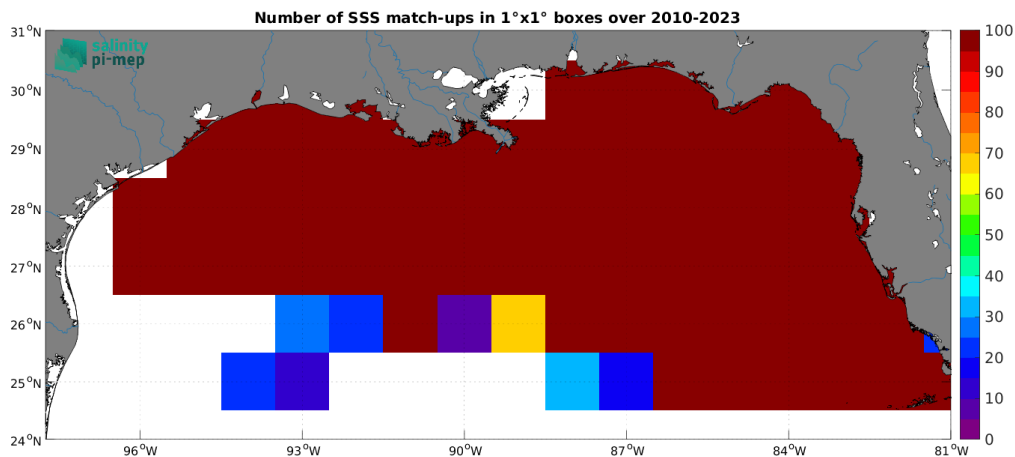
Figure 5: Number of SSS match-ups between TSG (SAMOS) SSS and the CCI SSS L4 Merged-OI v5.5 - 7-day running (ESA) SSS product for the Mississippi river plume Pi-MEP region over 1^\circ \times 1^\circ boxes and for the full satellite product period.
