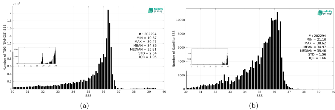
Figure 3: Histograms of SSS from TSG (SAMOS) (a) and CCI SSS L4 Merged-OI v5.5 - 7-day running (ESA) (b) considering all match-up pairs per bins of 0.1 over the Mississippi river plume Pi-MEP region and for the full satellite product period.
