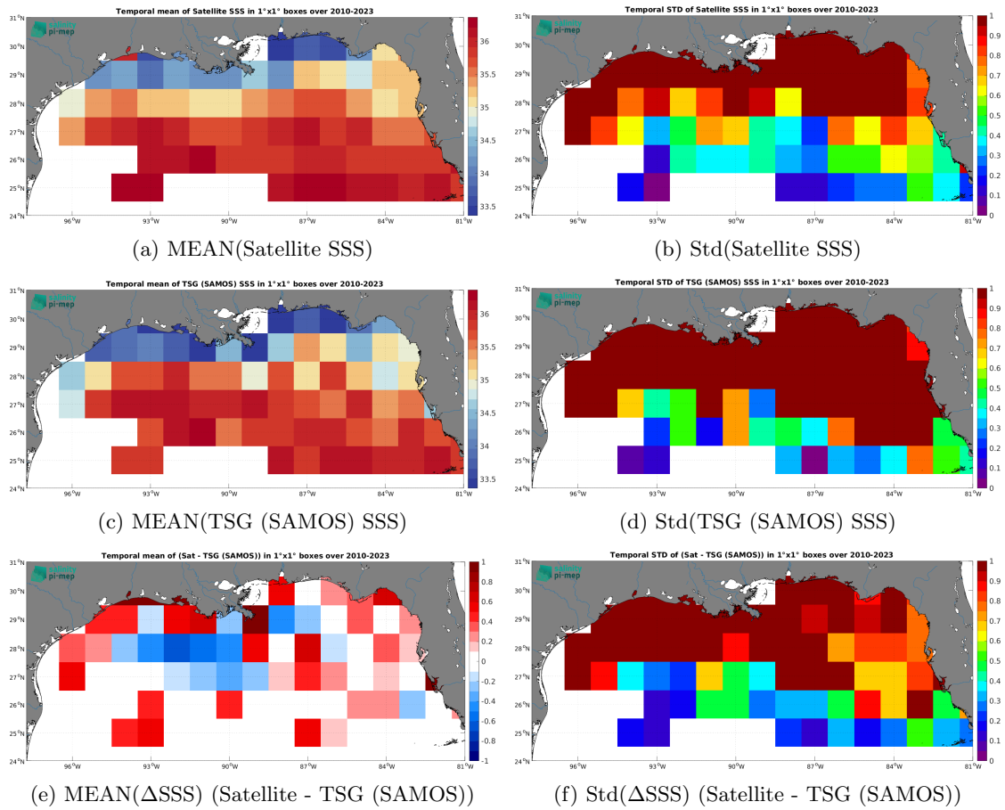
Figure 7: Temporal mean (left) and Std (right) of SSS from CCI SSS L4 Merged-OI v5.5 - 7-day running (ESA) (top), TSG (SAMOS) ( in situ ) dataset (middle), and of \Delta SSS (Satellite - TSG (SAMOS)). Only match-up pairs are used to generate these maps.
