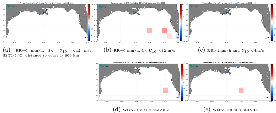
Figure 14: Temporal mean gridded over spatial boxes of size 1^\circ \times 1^\circ of \Delta SSS (CCI SSS L4 Merged-OI v5.5 - 7-day running (ESA) - TSG (GOSUD-Sailing-ship)) for 5 different subdatasets corresponding to: RR=0 mm/h, 3 < U_{10} < 12 m/s, SST>5°C, distance to coast > 800 km (a), RR=0 mm/h, 3 < U_{10} < 12 m/s (b), RR>1mm/h and U_{10} < 4 m/s (c), WOA2013 SSS Std<0.2 (d), WOA2013 SSS Std>0.2 (e).
