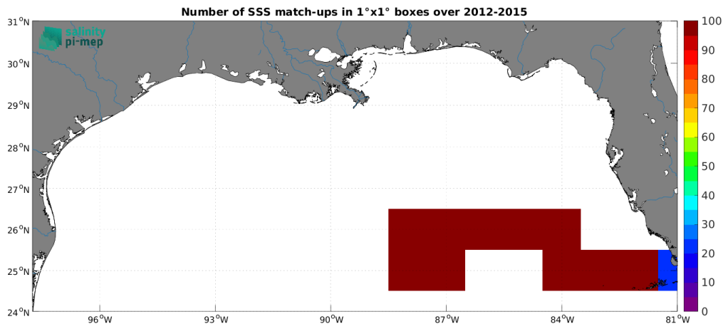
Figure 5: Number of SSS match-ups between TSG (GOSUD-Sailing-ship) SSS and the CCI SSS L4 Merged-OI v5.5 - 7-day running (ESA) SSS product for the Mississippi river plume Pi-MEP region over 1^\circ \times 1^\circ boxes and for the full satellite product period.
