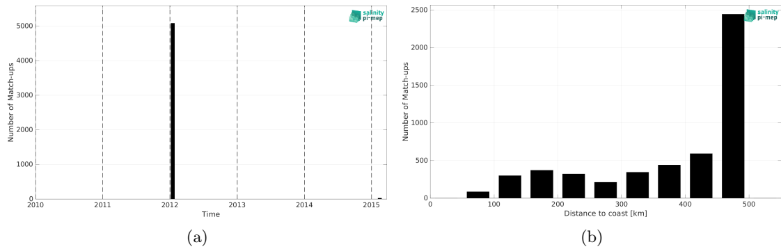
Figure 2: Number of match-ups between TSG (GOSUD-Sailing-ship) and CCI SSS L4 Merged-OI v5.5 - 7-day running (ESA) SSS as a function of time (a) and as function of the distance to coast (b) over the Mississippi river plume Pi-MEP region and for the full satellite product period.
