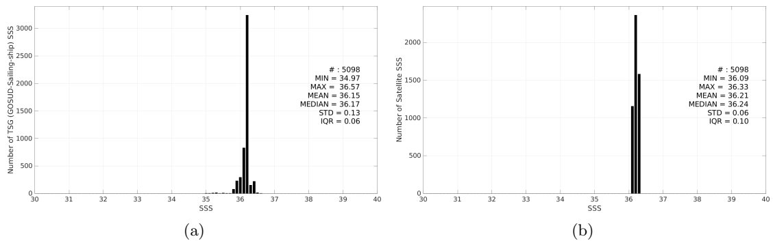
Figure 3: Histograms of SSS from TSG (GOSUD-Sailing-ship) (a) and CCI SSS L4 Merged-OI v5.5 - 7-day running (ESA) (b) considering all match-up pairs per bins of 0.1 over the Mississippi river plume Pi-MEP region and for the full satellite product period.
