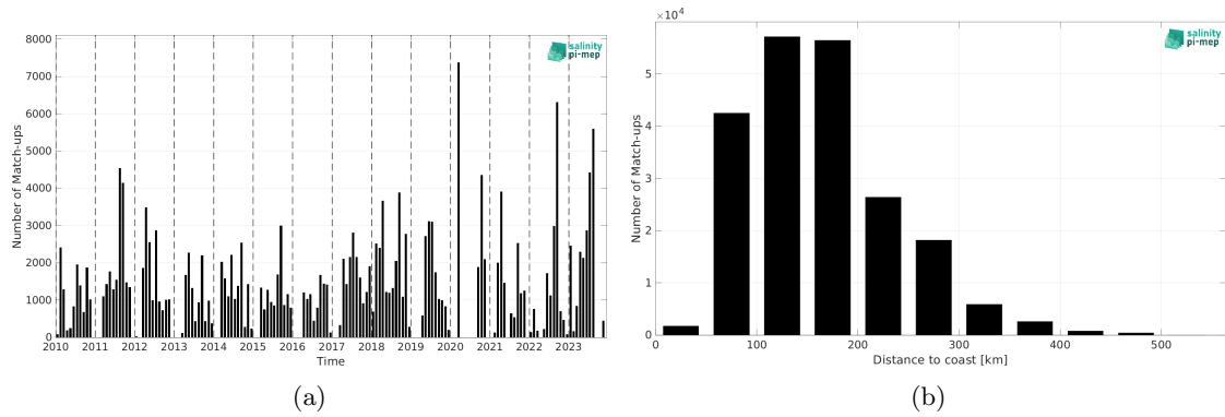
Figure 2: Number of match-ups between TSG (SAMOS) and CCI SSS L4 Merged-OI v5.5 - 30-day running (ESA) SSS as a function of time (a) and as function of the distance to coast (b) over the Mississippi river plume Pi-MEP region and for the full satellite product period.
