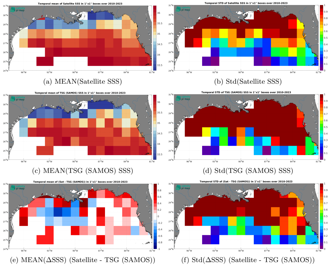
Figure 7: Temporal mean (left) and Std (right) of SSS from CCI SSS L4 Merged-OI v5.5 - 30-day running (ESA) (top), TSG (SAMOS) (middle), and of \Delta SSS (Satellite - TSG (SAMOS)). Only match-up pairs are used to generate these maps.
