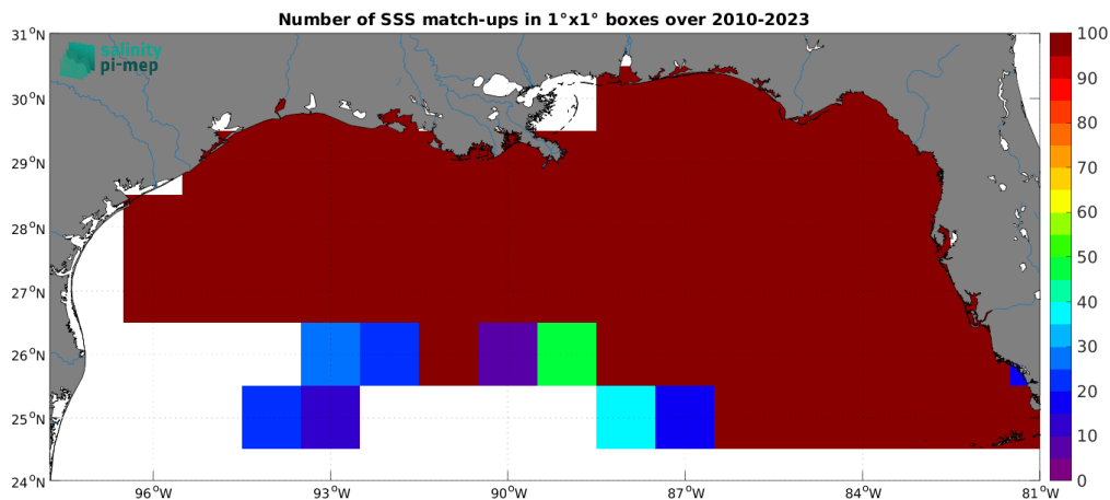
Figure 5: Number of SSS match-ups between TSG (SAMOS) SSS and the CCI SSS L4 Merged-OI v5.5 - 30-day running (ESA) SSS product for the Mississippi river plume Pi-MEP region over 1^\circ \times 1^\circ boxes and for the full satellite product period.
