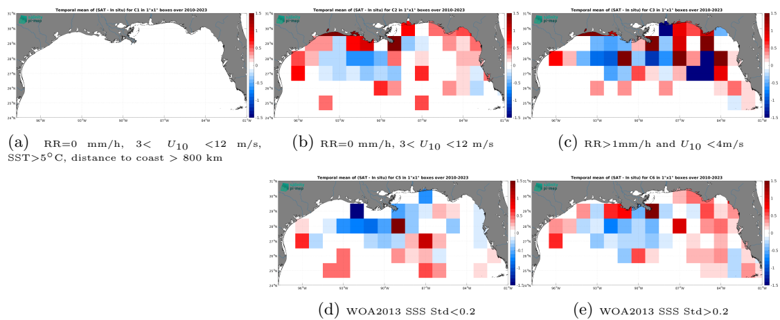
Figure 14: Temporal mean gridded over spatial boxes of size 1^\circ \times 1^\circ of \Delta SSS (CCI SSS L4 Merged-OI v5.5 - 30-day running (ESA) - TSG (SAMOS)) for 5 different subdatasets corresponding to: RR=0 mm/h, 3 < U_{10} < 12 m/s, SST > 5°C, distance to coast > 800 km (a), RR=0 mm/h, 3 < U_{10} < 12 m/s (b), RR > 1mm/h and U_{10} < 4 m/s (c), WOA2013 SSS Std < 0.2 (d), WOA2013 SSS Std > 0.2 (e).
