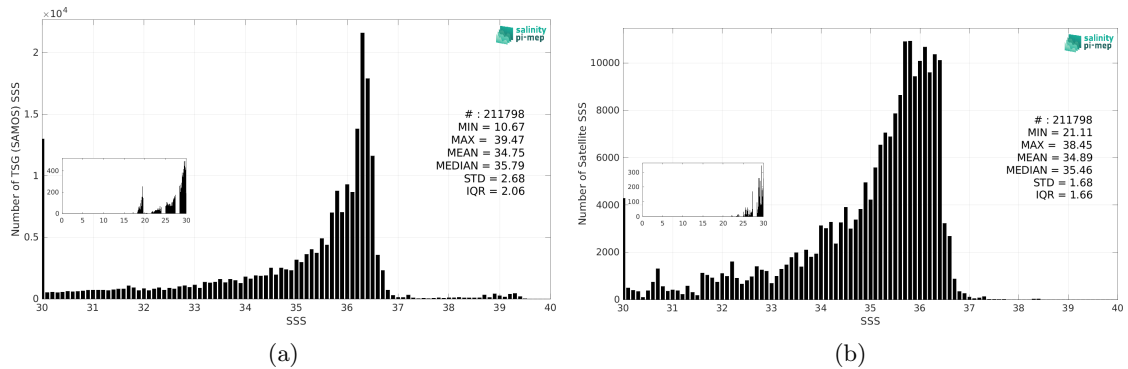
Figure 3: Histograms of SSS from TSG (SAMOS) (a) and CCI SSS L4 Merged-OI v5.5 - 30-day running (ESA) (b) considering all match-up pairs per bins of 0.1 over the Mississippi river plume Pi-MEP region and for the full satellite product period.
