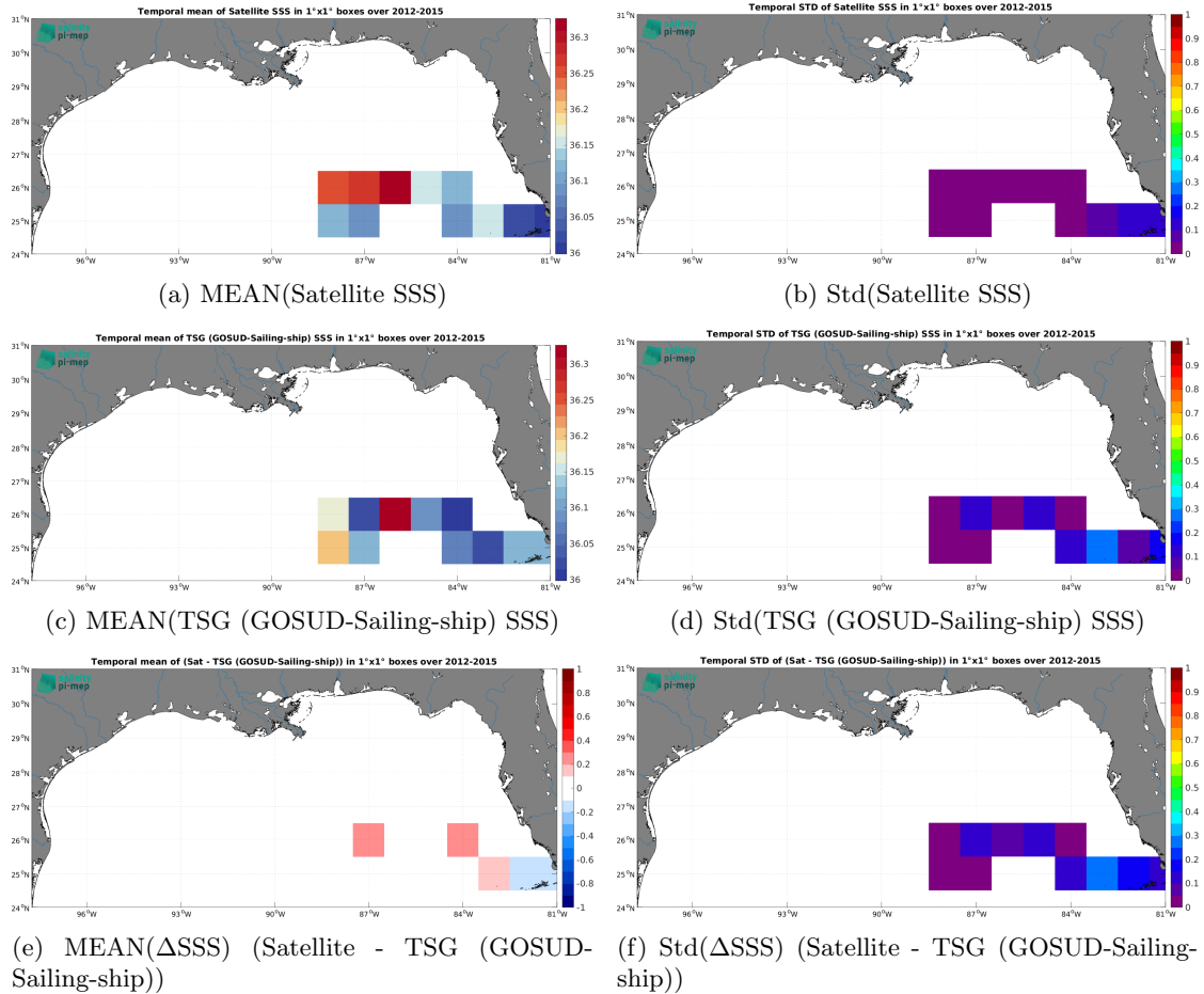
Figure 7: Temporal mean (left) and Std (right) of SSS from CCI SSS L4 Merged-OI v4.41 - 7-day running (ESA) (top), TSG (GOSUD-Sailing-ship) (middle), and of \Delta\text{SSS} (Satellite - TSG (GOSUD-Sailing-ship)). Only match-up pairs are used to generate these maps.
