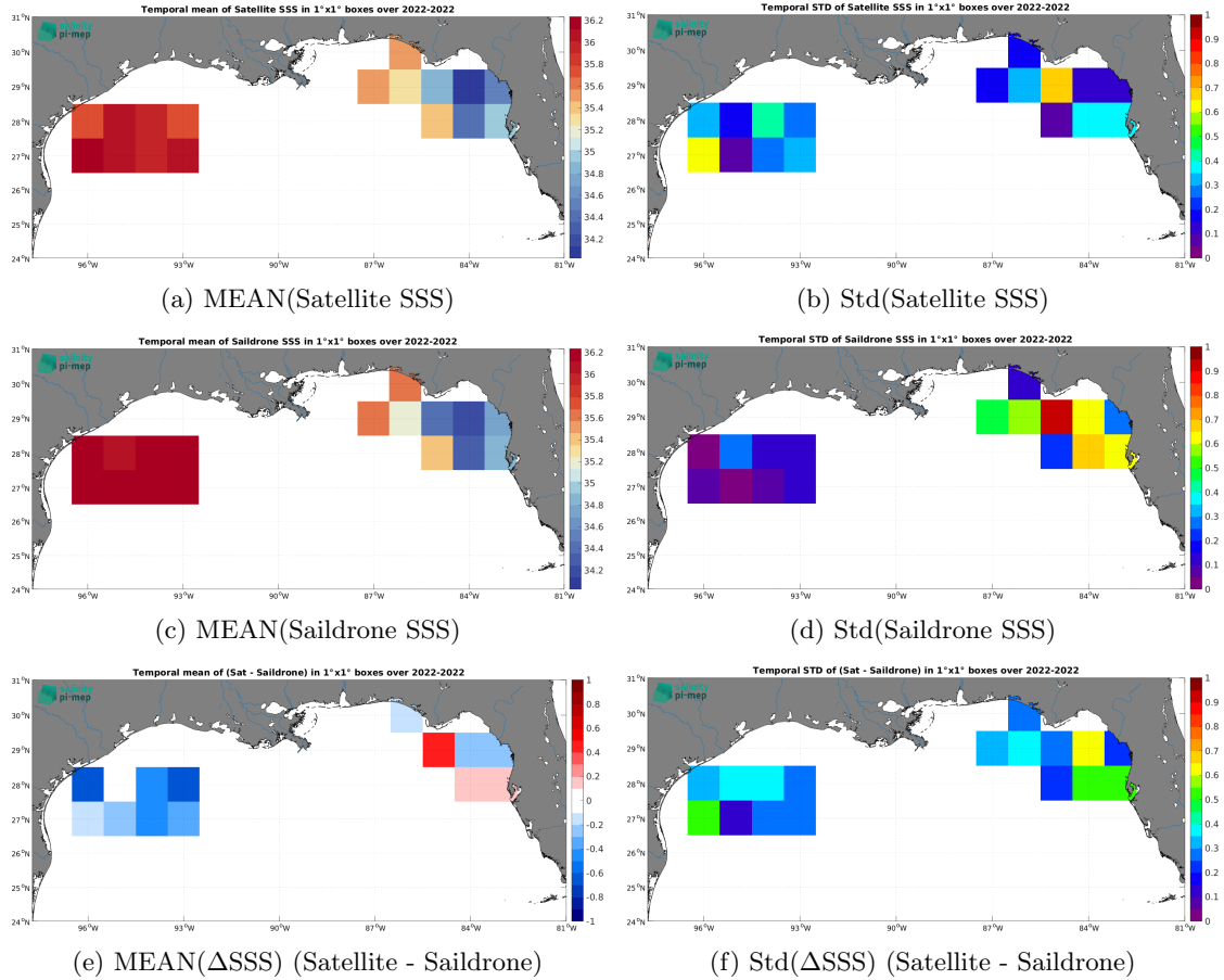
Figure 7: Temporal mean (left) and Std (right) of SSS from CCI SSS L4 Merged-OI v4.41 - 7-day running (ESA) (top), Saildrone (middle), and of \Delta\text{SSS} (Satellite - Saildrone). Only match-up pairs are used to generate these maps.
