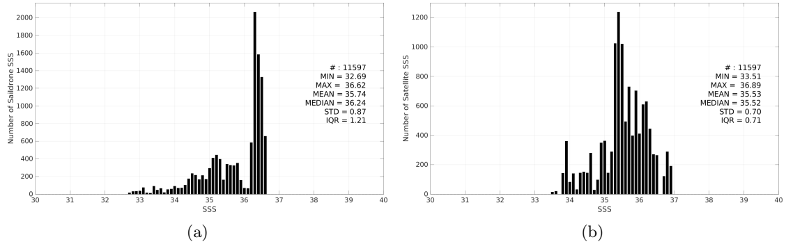
Figure 3: Histograms of SSS from Saildrone (a) and CCI SSS L4 Merged-OI v4.41 - 7-day running (ESA) (b) considering all match-up pairs per bins of 0.1 over the Mississippi river plume Pi-MEP region and for the full satellite product period.
