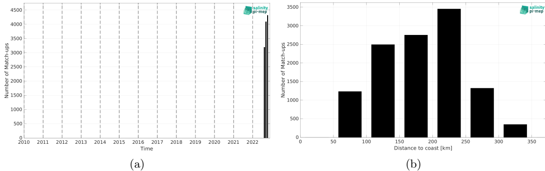
Figure 2: Number of match-ups between Saildrone and CCI SSS L4 Merged-OI v4.41 - 7-day running (ESA) SSS as a function of time (a) and as function of the distance to coast (b) over the Mississippi river plume Pi-MEP region and for the full satellite product period.
