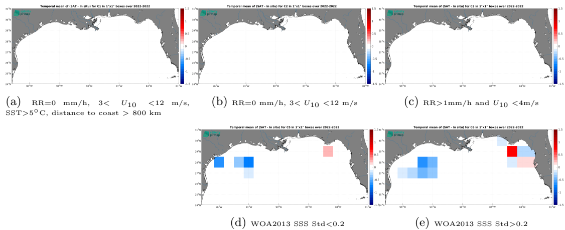
Figure 14: Temporal mean gridded over spatial boxes of size 1^\circ \times 1^\circ of \Delta SSS (CCI SSS L4 Merged-OI v4.41 - 7-day running (ESA) - Saildrone) for 5 different subdatasets corresponding to: RR=0 mm/h, 3 < U_{10} < 12 m/s, SST > 5^\circ\text{C} , distance to coast > 800 km (a), RR=0 mm/h, 3 < U_{10} < 12 m/s (b), RR > 1 mm/h and U_{10} < 4 m/s (c), WOA2013 SSS Std < 0.2 (d), WOA2013 SSS Std > 0.2 (e).
