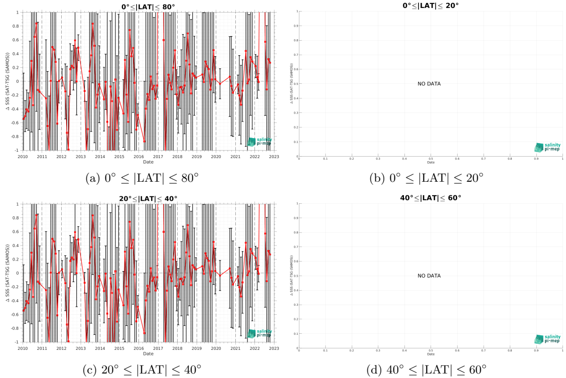
Figure 11: Monthly median (red curves) of \Delta SSS (Satellite - in situ ) between CCI SSS L4 Merged-OI v4.41 - 30-day running (ESA) and TSG (SAMOS) SSS as function of time for all the collected Pi-MEP match-up pairs estimated over the Mississippi river plume Pi-MEP region and for the full satellite product period are shown for different latitude bands: (a) 80^{\circ}\text{S}-80^{\circ}\text{N} , (b) 20^{\circ}\text{S}-20^{\circ}\text{N} , (c) 40^{\circ}\text{S}-20^{\circ}\text{S} and 20^{\circ}\text{N}-40^{\circ}\text{N} and (d) 60^{\circ}\text{S}-40^{\circ}\text{S} and 40^{\circ}\text{N}-60^{\circ}\text{N} .
