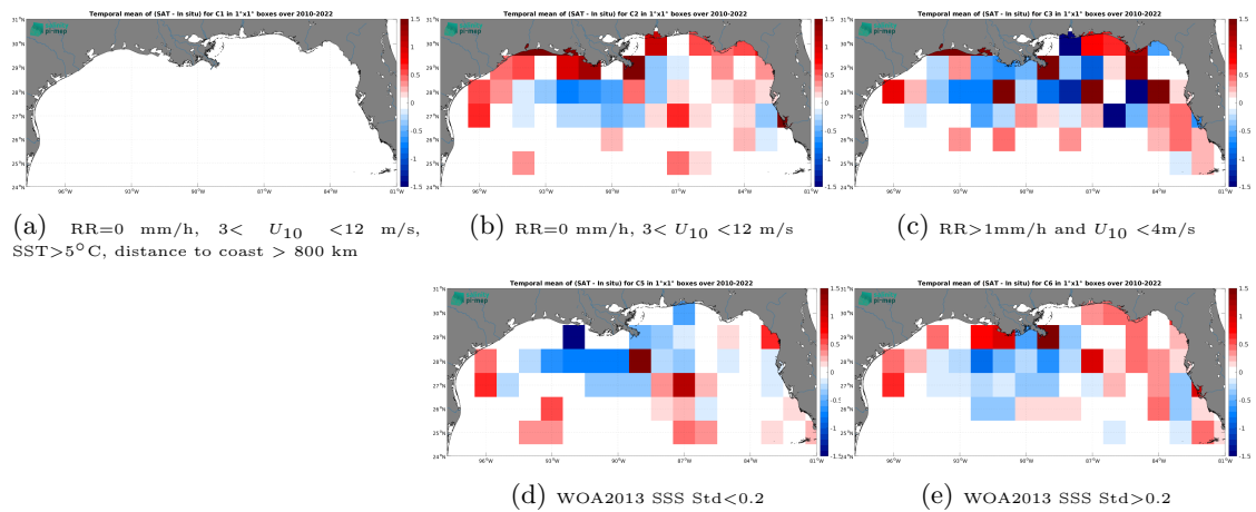
Figure 14: Temporal mean gridded over spatial boxes of size 1^\circ \times 1^\circ of \Delta SSS (CCI SSS L4 Merged-OI v4.41 - 30-day running (ESA) - TSG (SAMOS)) for 5 different subdatasets corresponding to: RR=0 mm/h, 3 < U_{10} < 12 m/s, SST > 5°C, distance to coast > 800 km (a), RR=0 mm/h, 3 < U_{10} < 12 m/s (b), RR > 1mm/h and U_{10} < 4 m/s (c), WOA2013 SSS Std < 0.2 (d), WOA2013 SSS Std > 0.2 (e).
