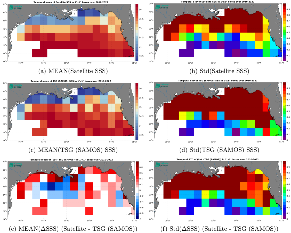
Figure 7: Temporal mean (left) and Std (right) of SSS from CCI SSS L4 Merged-OI v4.41 - 30-day running (ESA) (top), TSG (SAMOS) (middle), and of \Delta SSS (Satellite - TSG (SAMOS)). Only match-up pairs are used to generate these maps.
