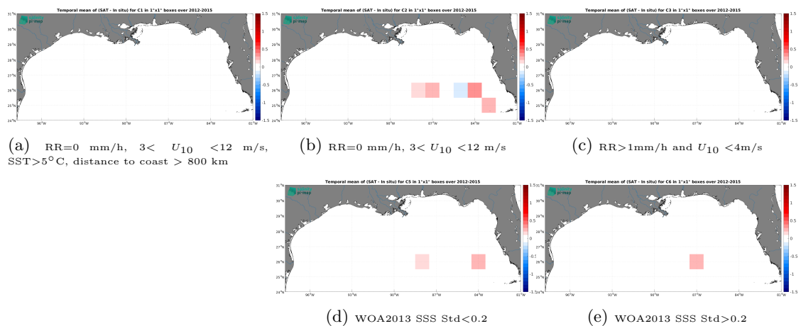
Figure 14: Temporal mean gridded over spatial boxes of size 1^\circ \times 1^\circ of \Delta SSS (CCI SSS L4 Merged-OI v4.41 - 30-day running (ESA) - TSG (GOSUD-Sailing-ship)) for 5 different subdatasets corresponding to: RR=0 mm/h, 3 < U_{10} < 12 m/s, SST > 5°C, distance to coast > 800 km (a), RR=0 mm/h, 3 < U_{10} < 12 m/s (b), RR > 1mm/h and U_{10} < 4 m/s (c), WOA2013 SSS Std < 0.2 (d), WOA2013 SSS Std > 0.2 (e).
