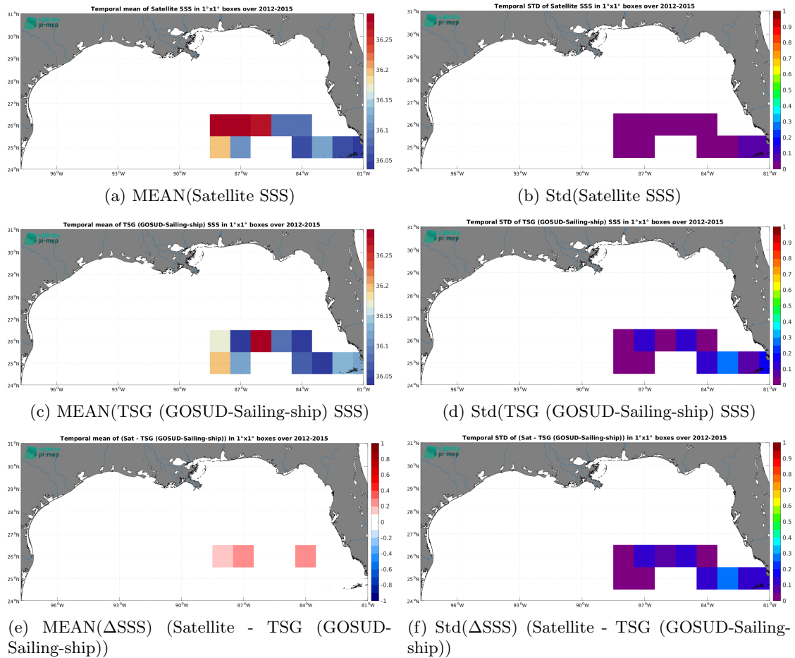
Figure 7: Temporal mean (left) and Std (right) of SSS from CCI SSS L4 Merged-OI v4.41 - 30-day running (ESA) (top), TSG (GOSUD-Sailing-ship) (middle), and of \Delta\text{SSS} (Satellite - TSG (GOSUD-Sailing-ship)). Only match-up pairs are used to generate these maps.
