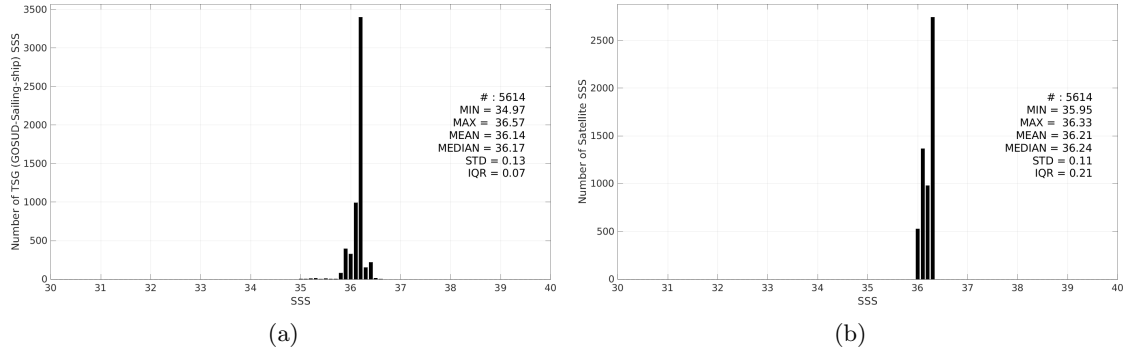
Figure 3: Histograms of SSS from TSG (GOSUD-Sailing-ship) (a) and CCI SSS L4 Merged-OI v4.41 - 30-day running (ESA) (b) considering all match-up pairs per bins of 0.1 over the Mississippi river plume Pi-MEP region and for the full satellite product period.
