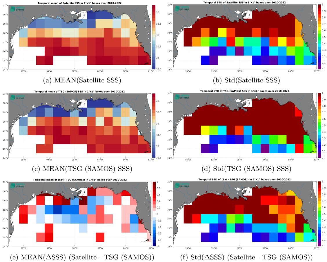
Figure 6: Temporal mean (left) and Std (right) of SSS from CCI SSS L4 Merged-OI v4.4 - 7-day running (ESA) (top), TSG (SAMOS) (middle), and of \Delta\text{SSS} (Satellite - TSG (SAMOS)). Only match-up pairs are used to generate these maps.
