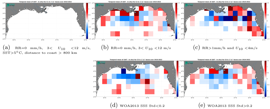
Figure 12: Temporal mean gridded over spatial boxes of size 1^{\circ}\times 1^{\circ} of \Delta\text{SSS} (CCI SSS L4 Merged-OI v4.4 - 7-day running (ESA) - TSG (SAMOS)) for 5 different subdatasets corresponding to:RR=0 mm/h, 3 < U_{10} < 12 m/s, SST > 5^{\circ}\text{C} , distance to coast > 800 km (a), RR=0 mm/h, 3 < U_{10} < 12 m/s (b), RR > 1 mm/h and U_{10} < 4 m/s (c), WOA2013 SSS Std < 0.2 (d), WOA2013 SSS Std > 0.2 (e).
