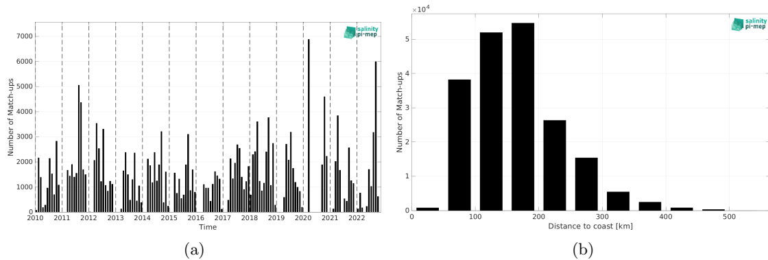
Figure 1: Number of match-ups between TSG (SAMOS) and CCI SSS L4 Merged-OI v4.4 - 7-day running (ESA) SSS as a function of time (a) and as function of the distance to coast (b) over the Mississippi river plume Pi-MEP region and for the full satellite product period.
