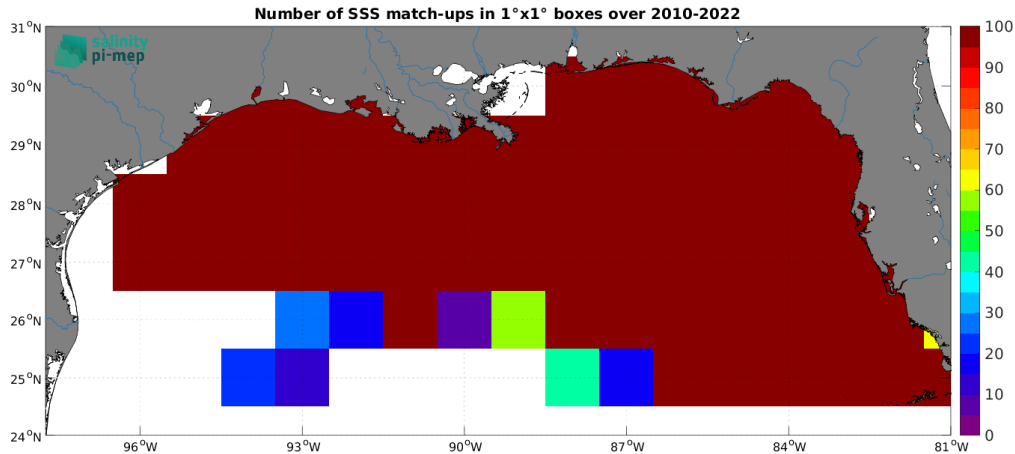
Figure 4: Number of SSS match-ups between TSG (SAMOS) SSS and the CCI SSS L4 Merged-OI v4.4 - 7-day running (ESA) SSS product for the Mississippi river plume Pi-MEP region over 1^\circ \times 1^\circ boxes and for the full satellite product period.
