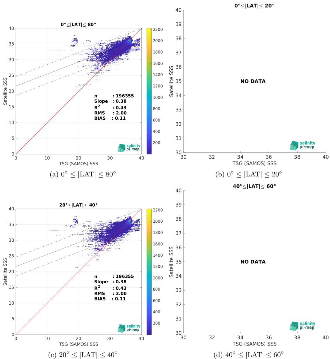
Figure 9: Contour maps of the concentration of CCI SSS L4 Merged-OI v4.4 - 7-day running (ESA) SSS (y-axis) versus TSG (SAMOS) SSS (x-axis) at match-up pairs for different latitude bands. For each plot, the red line shows x=y . The black thin and dashed lines indicate a linear fit through the data cloud and the \pm 95\% confidence levels, respectively. The number match-up pairs n , the slope and R^2 coefficient of the linear fit, the root mean square (RMS) and the mean bias between satellite and in situ data are indicated for each latitude band in each plots.
