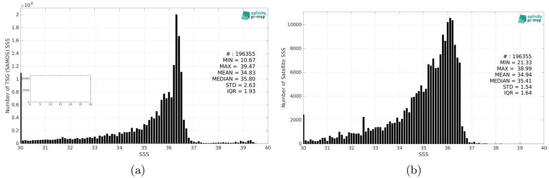
Figure 2: Histograms of SSS from TSG (SAMOS) (a) and CCI SSS L4 Merged-OI v4.4 - 7-day running (ESA) (b) considering all match-up pairs per bins of 0.1 over the Mississippi river plume Pi-MEP region and for the full satellite product period.
