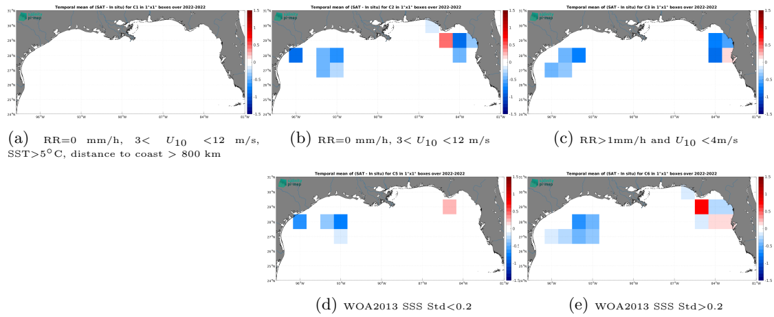
Figure 12: Temporal mean gridded over spatial boxes of size 1^{\circ}\times 1^{\circ} of \Delta\text{SSS} (CCI SSS L4 Merged-OI v4.4 - 7-day running (ESA) - Saildrone) for 5 different subdatasets corresponding to:RR=0 mm/h, 3 < U_{10} < 12 m/s, SST >5^{\circ}\text{C} , distance to coast > 800 km (a), RR=0 mm/h, 3 < U_{10} < 12 m/s (b), RR >1 mm/h and U_{10} < 4 m/s (c), WOA2013 SSS Std <0.2 (d), WOA2013 SSS Std >0.2 (e).
