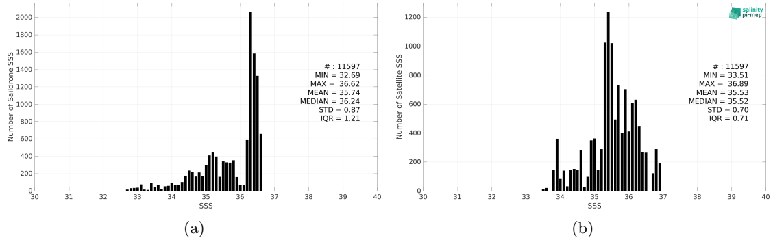
Figure 2: Histograms of SSS from Saildrone (a) and CCI SSS L4 Merged-OI v4.4 - 7-day running (ESA) (b) considering all match-up pairs per bins of 0.1 over the Mississippi river plume Pi-MEP region and for the full satellite product period.
