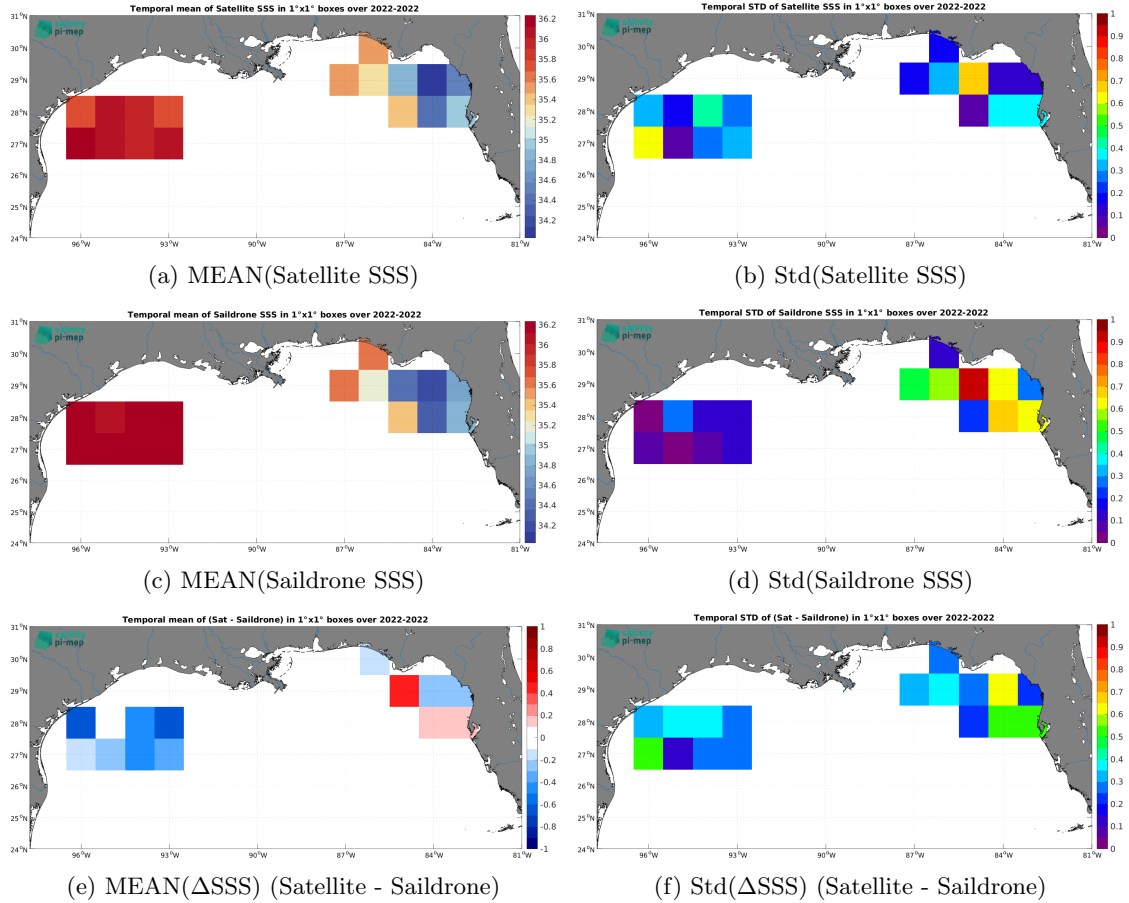
Figure 6: Temporal mean (left) and Std (right) of SSS from CCI SSS L4 Merged-OI v4.4 - 7-day running (ESA) (top), Saildrone (middle), and of \Delta\text{SSS} (Satellite - Saildrone). Only match-up pairs are used to generate these maps.
