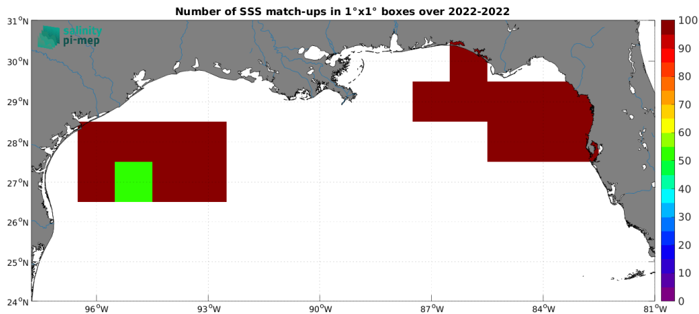
Figure 4: Number of SSS match-ups between Saildrone SSS and the CCI SSS L4 Merged-OI v4.4 - 7-day running (ESA) SSS product for the Mississippi river plume Pi-MEP region over 1^\circ \times 1^\circ boxes and for the full satellite product period.
