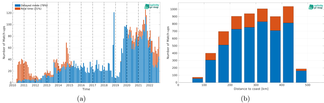
Figure 1: Number of match-ups between Argo and CCI SSS L4 Merged-OI v4.4 - 7-day running (ESA) SSS as a function of time (a) and as function of the distance to coast (b) over the Mississippi river plume Pi-MEP region and for the full satellite product period.
