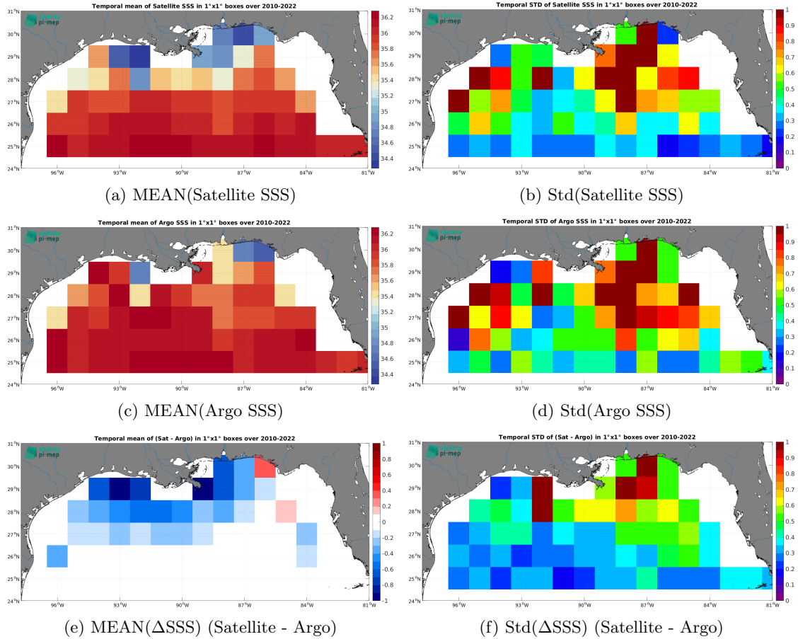
Figure 6: Temporal mean (left) and Std (right) of SSS from CCI SSS L4 Merged-OI v4.4 - 7-day running (ESA) (top), Argo (middle), and of \Delta\text{SSS} (Satellite - Argo). Only match-up pairs are used to generate these maps.
