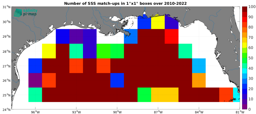
Figure 4: Number of SSS match-ups between Argo SSS and the CCI SSS L4 Merged-OI v4.4 - 7-day running (ESA) SSS product for the Mississippi river plume Pi-MEP region over 1^\circ \times 1^\circ boxes and for the full satellite product period.
