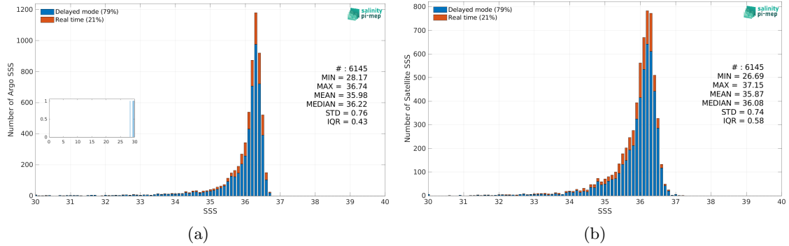
Figure 2: Histograms of SSS from Argo (a) and CCI SSS L4 Merged-OI v4.4 - 7-day running (ESA) (b) considering all match-up pairs per bins of 0.1 over the Mississippi river plume Pi-MEP region and for the full satellite product period.
