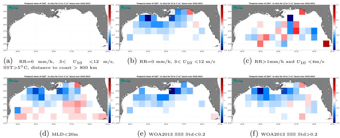
Figure 12: Temporal mean gridded over spatial boxes of size 1^{\circ}\times 1^{\circ} of \Delta\text{SSS} (CCI SSS L4 Merged-OI v4.4 - 7-day running (ESA) - Argo) for 6 different subdatasets corresponding to:RR=0 mm/h, 3 < U_{10} < 12 m/s, SST > 5^{\circ}\text{C} , distance to coast > 800 km (a), RR=0 mm/h, 3 < U_{10} < 12 m/s (b), RR > 1\text{mm/h} and U_{10} < 4\text{m/s} (c),MLD < 20\text{m} (d),WOA2013 SSS Std < 0.2 (e),WOA2013 SSS Std > 0.2 (f).
