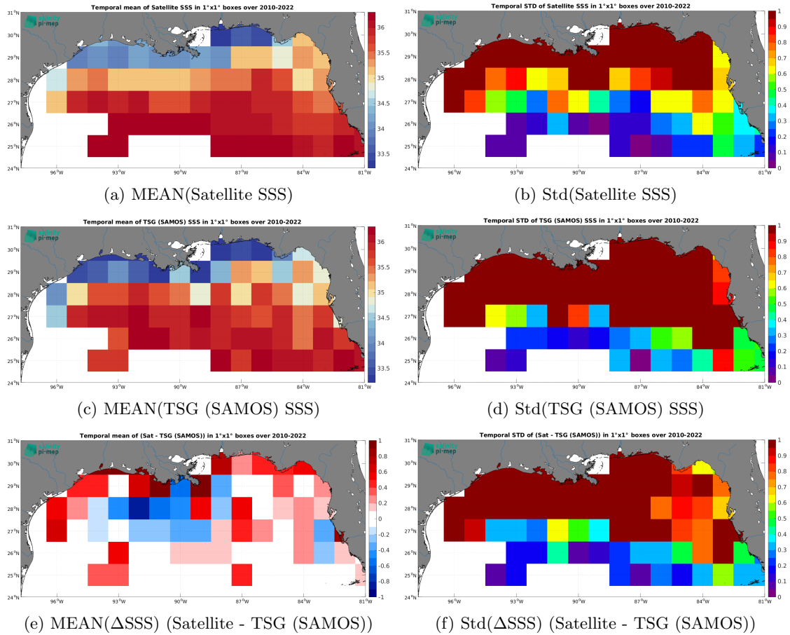
Figure 6: Temporal mean (left) and Std (right) of SSS from CCI SSS L4 Merged-OI v4.4 - 30-day running (ESA) (top), TSG (SAMOS) (middle), and of \Delta\text{SSS} (Satellite - TSG (SAMOS)). Only match-up pairs are used to generate these maps.
