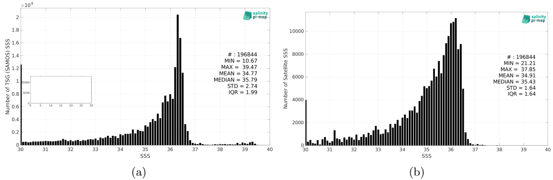
Figure 2: Histograms of SSS from TSG (SAMOS) (a) and CCI SSS L4 Merged-OI v4.4 - 30-day running (ESA) (b) considering all match-up pairs per bins of 0.1 over the Mississippi river plume Pi-MEP region and for the full satellite product period.
