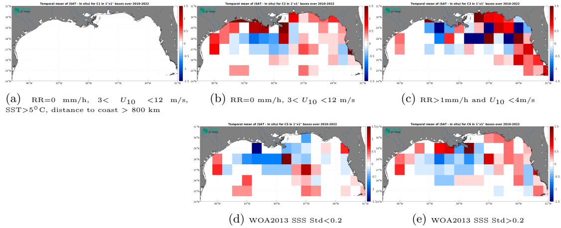
Figure 12: Temporal mean gridded over spatial boxes of size 1^{\circ}\times 1^{\circ} of \Delta\text{SSS} (CCI SSS L4 Merged-OI v4.4 - 30-day running (ESA) - TSG (SAMOS)) for 5 different subdatasets corresponding to:RR=0 mm/h, 3 < U_{10} < 12 m/s, SST > 5^{\circ}\text{C} , distance to coast > 800 km (a), RR=0 mm/h, 3 < U_{10} < 12 m/s (b), RR > 1 mm/h and U_{10} < 4 m/s (c), WOA2013 SSS Std < 0.2 (d), WOA2013 SSS Std > 0.2 (e).
