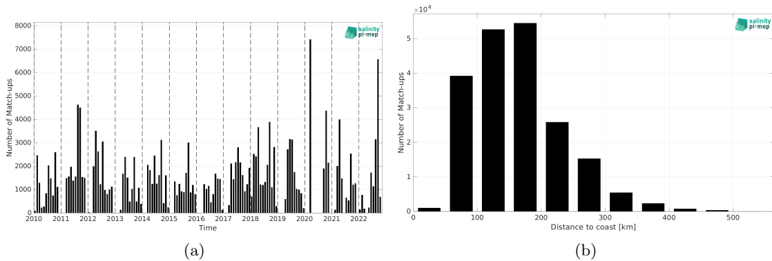
Figure 1: Number of match-ups between TSG (SAMOS) and CCI SSS L4 Merged-OI v4.4 - 30-day running (ESA) SSS as a function of time (a) and as function of the distance to coast (b) over the Mississippi river plume Pi-MEP region and for the full satellite product period.
