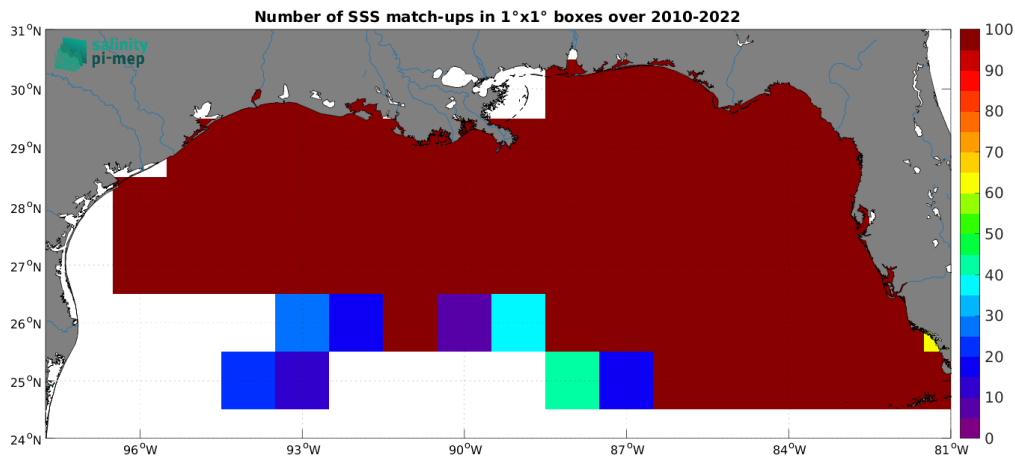
Figure 4: Number of SSS match-ups between TSG (SAMOS) SSS and the CCI SSS L4 Merged-OI v4.4 - 30-day running (ESA) SSS product for the Mississippi river plume Pi-MEP region over 1^\circ \times 1^\circ boxes and for the full satellite product period.
