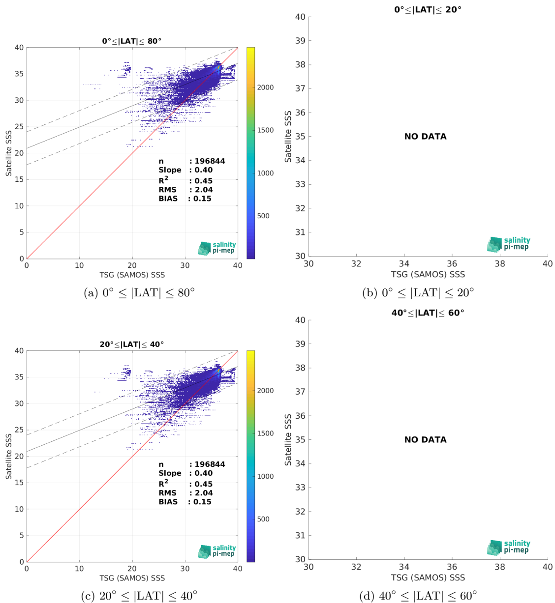
Figure 9: Contour maps of the concentration of CCI SSS L4 Merged-OI v4.4 - 30-day running (ESA) SSS (y-axis) versus TSG (SAMOS) SSS (x-axis) at match-up pairs for different latitude bands. For each plot, the red line shows x=y . The black thin and dashed lines indicate a linear fit through the data cloud and the \pm 95\% confidence levels, respectively. The number match-up pairs n , the slope and R^2 coefficient of the linear fit, the root mean square (RMS) and the mean bias between satellite and in situ data are indicated for each latitude band in each plot.
