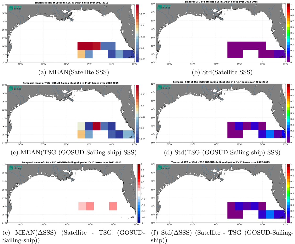
Figure 6: Temporal mean (left) and Std (right) of SSS from CCI SSS L4 Merged-OI v4.4 - 30-day running (ESA) (top), TSG (GOSUD-Sailing-ship) (middle), and of \Delta\text{SSS} (Satellite - TSG (GOSUD-Sailing-ship)). Only match-up pairs are used to generate these maps.
