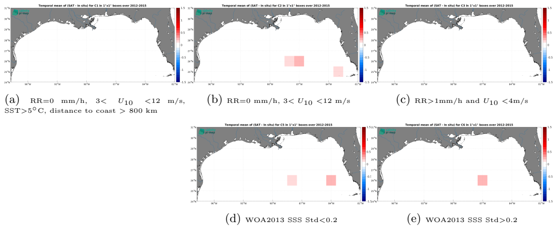
Figure 12: Temporal mean gridded over spatial boxes of size 1^{\circ}\times 1^{\circ} of \Delta SSS (CCI SSS L4 Merged-OI v4.4 - 30-day running (ESA) - TSG (GOSUD-Sailing-ship)) for 5 different subdatasets corresponding to:RR=0 mm/h, 3 < U_{10} < 12 m/s, SST > 5^{\circ}\text{C} , distance to coast > 800 km (a), RR=0 mm/h, 3 < U_{10} < 12 m/s (b), RR > 1 mm/h and U_{10} < 4 m/s (c), WOA2013 SSS Std < 0.2 (d), WOA2013 SSS Std > 0.2 (e).
