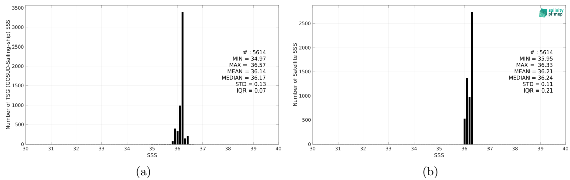
Figure 2: Histograms of SSS from TSG (GOSUD-Sailing-ship) (a) and CCI SSS L4 Merged-OI v4.4 - 30-day running (ESA) (b) considering all match-up pairs per bins of 0.1 over the Mississippi river plume Pi-MEP region and for the full satellite product period.
