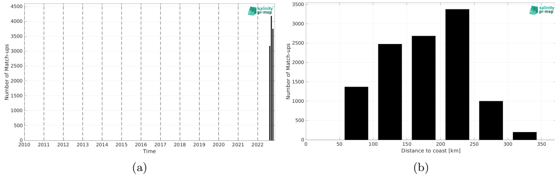
Figure 1: Number of match-ups between Saildrone and CCI SSS L4 Merged-OI v4.4 - 30-day running (ESA) SSS as a function of time (a) and as function of the distance to coast (b) over the Mississippi river plume Pi-MEP region and for the full satellite product period.
