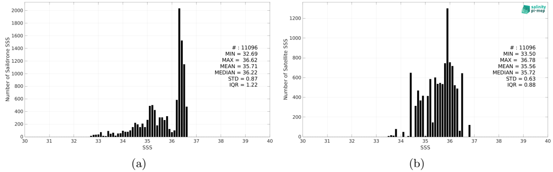
Figure 2: Histograms of SSS from Saildrone (a) and CCI SSS L4 Merged-OI v4.4 - 30-day running (ESA) (b) considering all match-up pairs per bins of 0.1 over the Mississippi river plume Pi-MEP region and for the full satellite product period.
