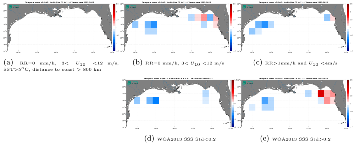
Figure 12: Temporal mean gridded over spatial boxes of size 1^{\circ}\times 1^{\circ} of \Delta\text{SSS} (CCI SSS L4 Merged-OI v4.4 - 30-day running (ESA) - Saildrone) for 5 different subdatasets corresponding to:RR=0 mm/h, 3 < U_{10} < 12 m/s, SST >5^{\circ}\text{C} , distance to coast > 800 km (a), RR=0 mm/h, 3 < U_{10} < 12 m/s (b), RR >1 mm/h and U_{10} < 4 m/s (c), WOA2013 SSS Std <0.2 (d), WOA2013 SSS Std >0.2 (e).
