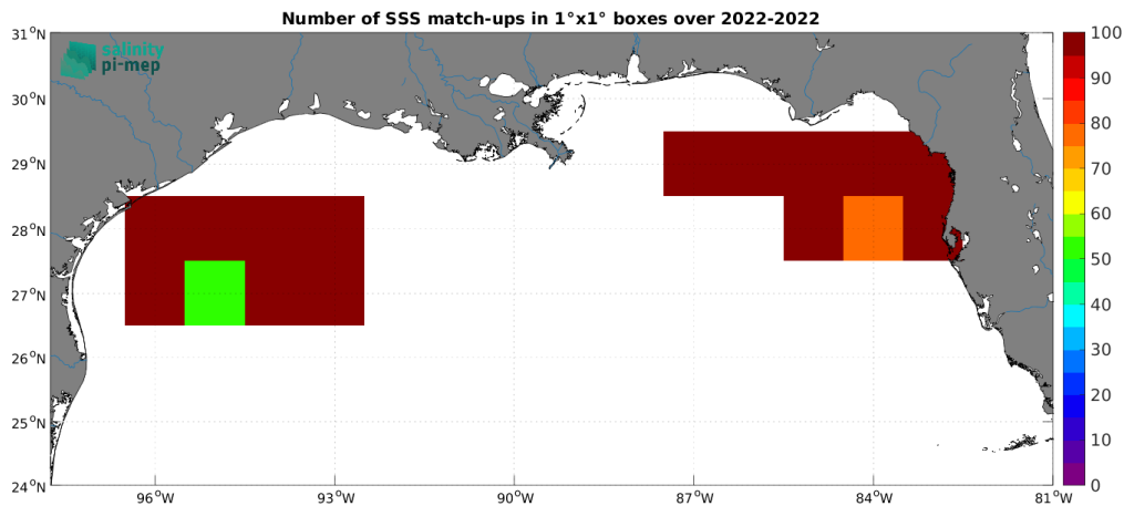
Figure 4: Number of SSS match-ups between Saildrone SSS and the CCI SSS L4 Merged-OI v4.4 - 30-day running (ESA) SSS product for the Mississippi river plume Pi-MEP region over 1^\circ \times 1^\circ boxes and for the full satellite product period.
