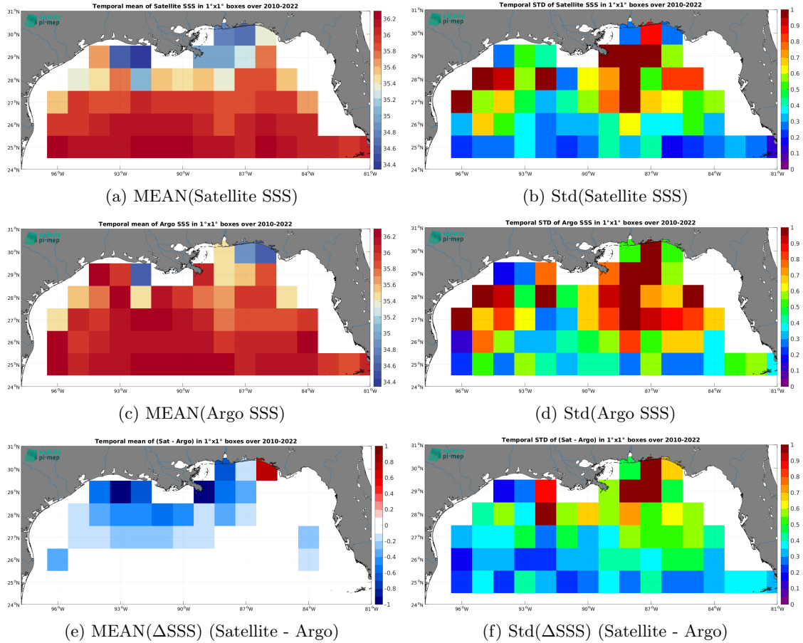
Figure 6: Temporal mean (left) and Std (right) of SSS from CCI SSS L4 Merged-OI v4.4 - 30-day running (ESA) (top), Argo (middle), and of \Delta\text{SSS} (Satellite - Argo). Only match-up pairs are used to generate these maps.
