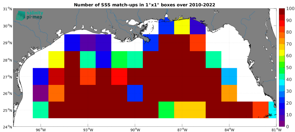
Figure 4: Number of SSS match-ups between Argo SSS and the CCI SSS L4 Merged-OI v4.4 - 30-day running (ESA) SSS product for the Mississippi river plume Pi-MEP region over 1^\circ \times 1^\circ boxes and for the full satellite product period.
