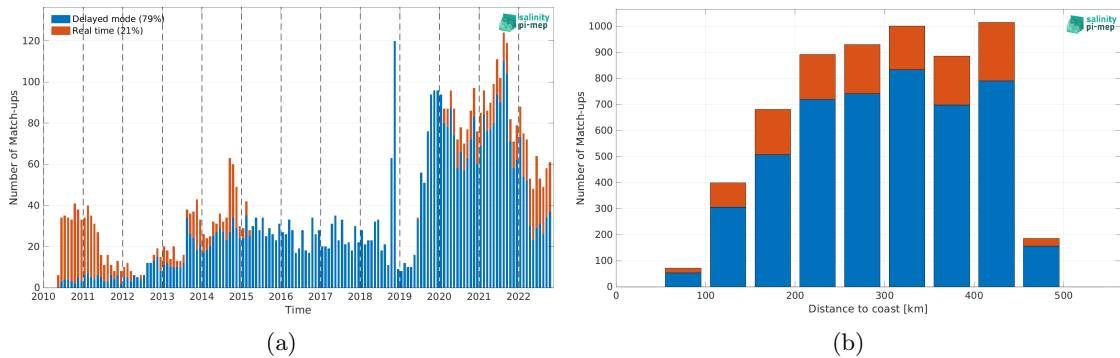
Figure 1: Number of match-ups between Argo and CCI SSS L4 Merged-OI v4.4 - 30-day running (ESA) SSS as a function of time (a) and as function of the distance to coast (b) over the Mississippi river plume Pi-MEP region and for the full satellite product period.
