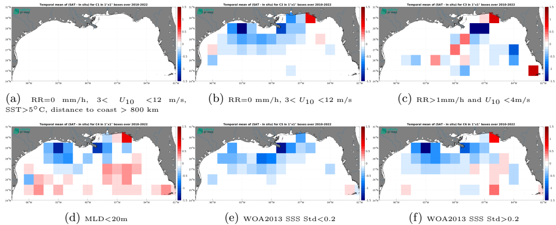
Figure 12: Temporal mean gridded over spatial boxes of size 1^{\circ}\times 1^{\circ} of \Delta\text{SSS} (CCI SSS L4 Merged-OI v4.4 - 30-day running (ESA) - Argo) for 6 different subdatasets corresponding to:RR=0 mm/h, 3 < U_{10} < 12 m/s, SST > 5^{\circ}\text{C} , distance to coast > 800 km (a), RR=0 mm/h, 3 < U_{10} < 12 m/s (b), RR > 1\text{mm/h} and U_{10} < 4\text{m/s} (c),MLD < 20\text{m} (d),WOA2013 SSS Std < 0.2 (e),WOA2013 SSS Std > 0.2 (f).
