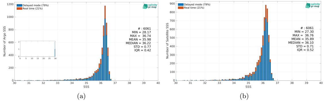
Figure 2: Histograms of SSS from Argo (a) and CCI SSS L4 Merged-OI v4.4 - 30-day running (ESA) (b) considering all match-up pairs per bins of 0.1 over the Mississippi river plume Pi-MEP region and for the full satellite product period.
