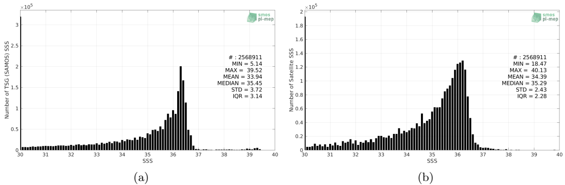
Figure 2: Histograms of SSS from TSG (SAMOS) (a) and CCI SSS L4 Merged-OI v3.2 - 30-day running (ESA) (b) considering all match-up pairs per bins of 0.1 over the Mississippi river plume Pi-MEP region and for the full satellite product period.
