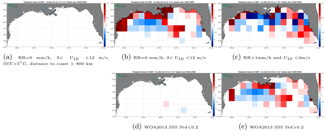
Figure 12: Temporal mean gridded over spatial boxes of size 1^{\circ}\times 1^{\circ} of \Delta\text{SSS} (CCI SSS L4 Merged-OI v3.2 - 30-day running (ESA) - TSG (SAMOS)) for 5 different subdatasets corresponding to:RR=0 mm/h, 3 < U_{10} < 12 m/s, SST >5^{\circ}\text{C} , distance to coast > 800 km (a), RR=0 mm/h, 3 < U_{10} < 12 m/s (b), RR >1 mm/h and U_{10} < 4 m/s (c), WOA2013 SSS Std <0.2 (d), WOA2013 SSS Std >0.2 (e).
