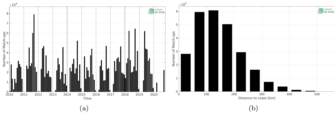
Figure 1: Number of match-ups between TSG (SAMOS) and CCI SSS L4 Merged-OI v3.2 - 30-day running (ESA) SSS as a function of time (a) and as function of the distance to coast (b) over the Mississippi river plume Pi-MEP region and for the full satellite product period.
