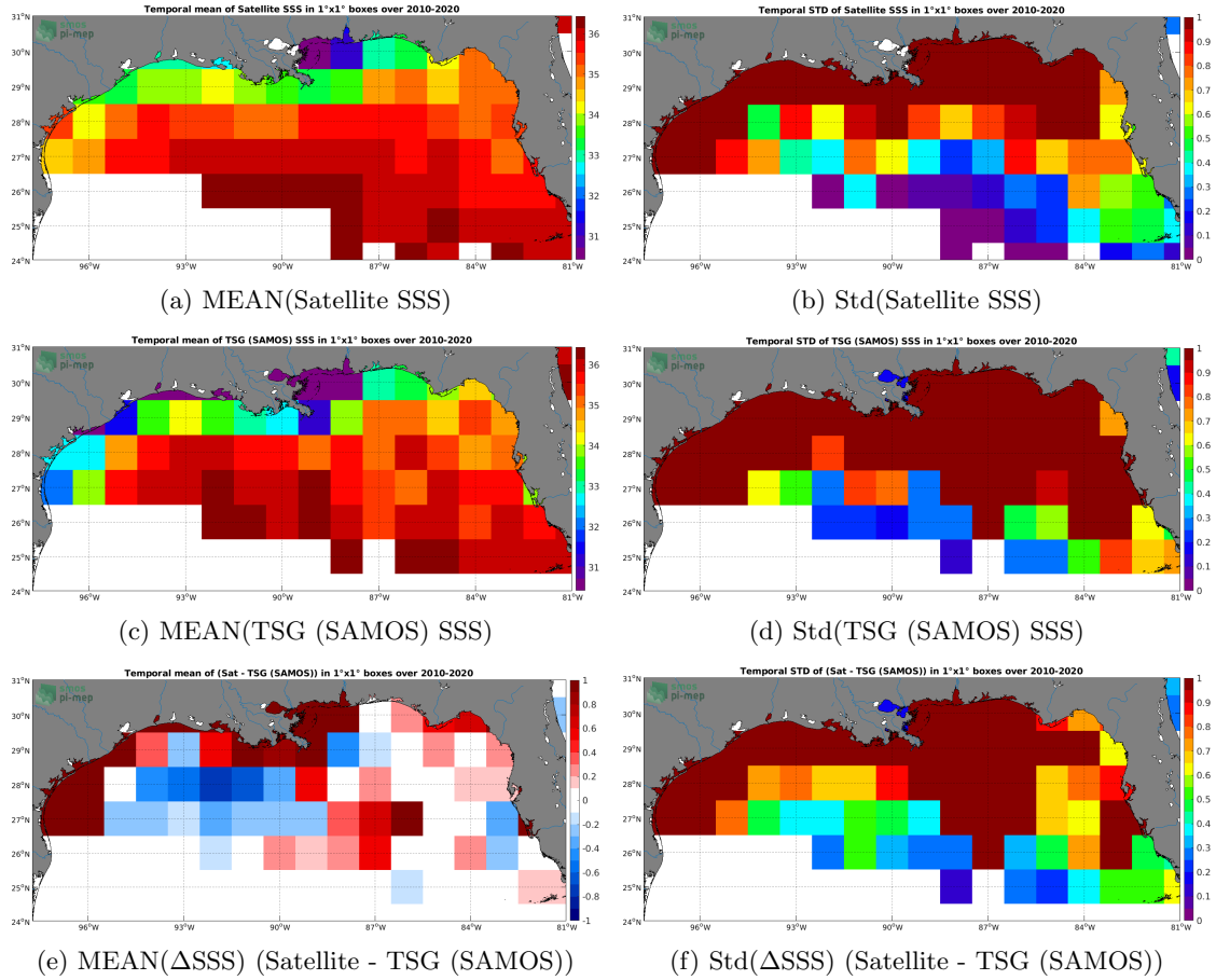
Figure 6: Temporal mean (left) and Std (right) of SSS from CCI SSS L4 Merged-OI v3.2 - 30-day running (ESA) (top), TSG (SAMOS) (middle), and of \Delta SSS (Satellite - TSG (SAMOS)). Only match-up pairs are used to generate these maps.
