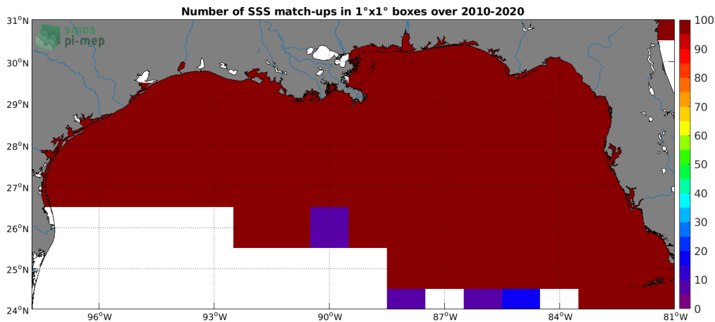
Figure 4: Number of SSS match-ups between TSG (SAMOS) SSS and the CCI SSS L4 Merged-OI v3.2 - 30-day running (ESA) SSS product for the Mississippi river plume Pi-MEP region over 1°x1° boxes and for the full satellite product period.
