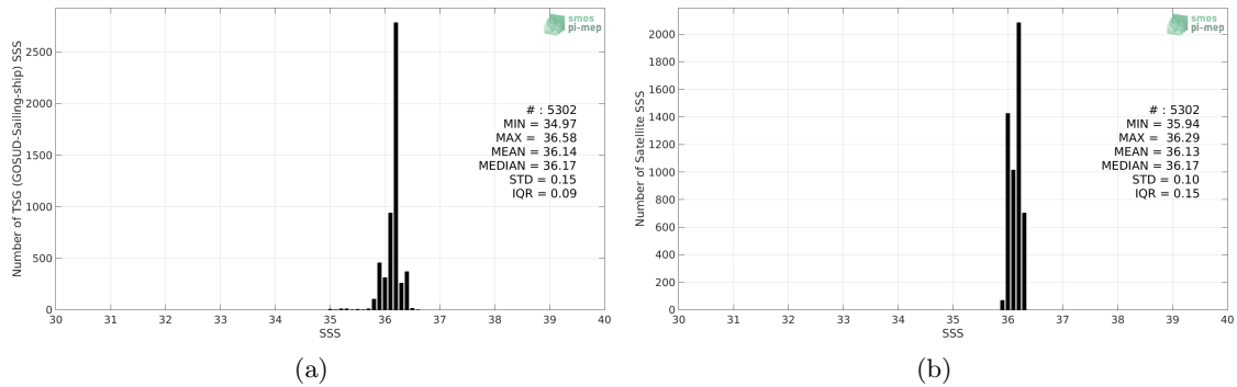
Figure 2: Histograms of SSS from TSG (GOSUD-Sailing-ship) (a) and CCI SSS L4 Merged-OI v3.2 - 30-day running (ESA) (b) considering all match-up pairs per bins of 0.1 over the Mississippi river plume Pi-MEP region and for the full satellite product period.
