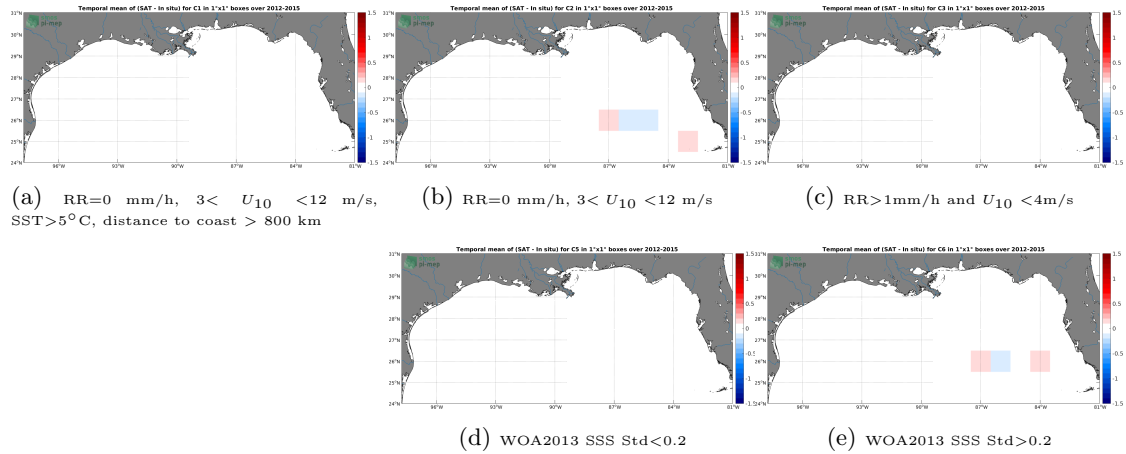
Figure 12: Temporal mean gridded over spatial boxes of size 1^\circ \times 1^\circ of \Delta SSS (CCI SSS L4 Merged-OI v3.2 - 30-day running (ESA) - TSG (GOSUD-Sailing-ship)) for 5 different subdatasets corresponding to: RR=0 mm/h, 3 < U_{10} < 12 m/s, SST > 5^\circ\text{C} , distance to coast > 800 km (a), RR=0 mm/h, 3 < U_{10} < 12 m/s (b), RR > 1 mm/h and U_{10} < 4 m/s (c), WOA2013 SSS Std < 0.2 (d), WOA2013 SSS Std > 0.2 (e).
