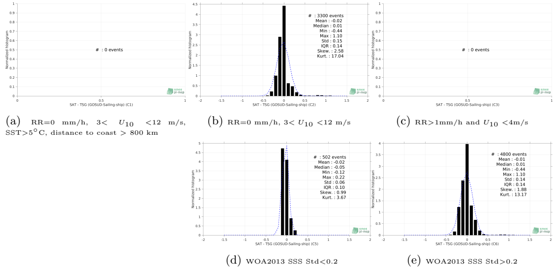
Figure 13: Normalized histogram of \Delta\text{SSS} (CCI SSS L4 Merged-OI v3.2 - 30-day running (ESA) - TSG (GOSUD-Sailing-ship)) for 5 different subdatasets corresponding to: RR=0 mm/h, 3 < U_{10} < 12 m/s, SST > 5^\circ\text{C} , distance to coast > 800 km (a), RR=0 mm/h, 3 < U_{10} < 12 m/s (b), RR > 1\text{mm/h} and U_{10} < 4\text{m/s} (c), WOA2013 SSS \text{Std} < 0.2 (d), WOA2013 SSS \text{Std} > 0.2 (e).
