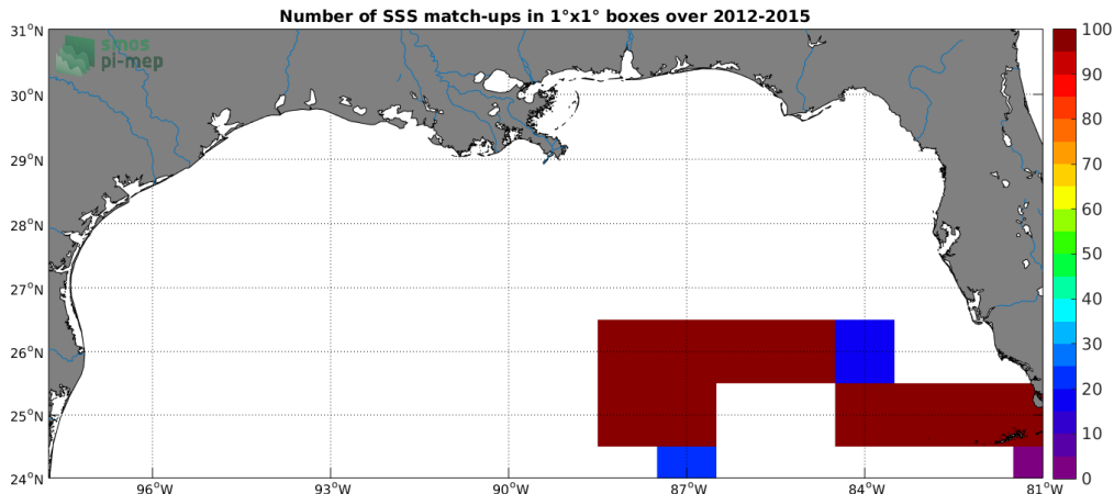
Figure 4: Number of SSS match-ups between TSG (GOSUD-Sailing-ship) SSS and the CCI SSS L4 Merged-OI v3.2 - 30-day running (ESA) SSS product for the Mississippi river plume Pi-MEP region over 1°x1° boxes and for the full satellite product period.
