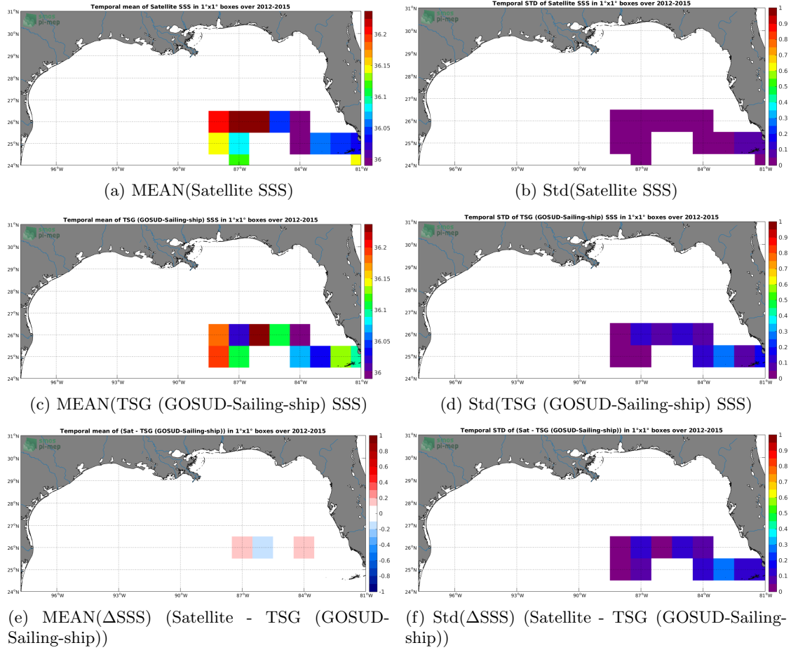
Figure 6: Temporal mean (left) and Std (right) of SSS from CCI SSS L4 Merged-OI v3.2 - 30-day running (ESA) (top), TSG (GOSUD-Sailing-ship) (middle), and of \Delta SSS (Satellite - TSG (GOSUD-Sailing-ship)). Only match-up pairs are used to generate these maps.
