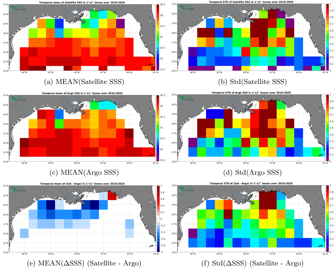
Figure 6: Temporal mean (left) and Std (right) of SSS from CCI SSS L4 Merged-OI v3.2 - 30-day running (ESA) (top), Argo (middle), and of \Delta SSS (Satellite - Argo). Only match-up pairs are used to generate these maps.
