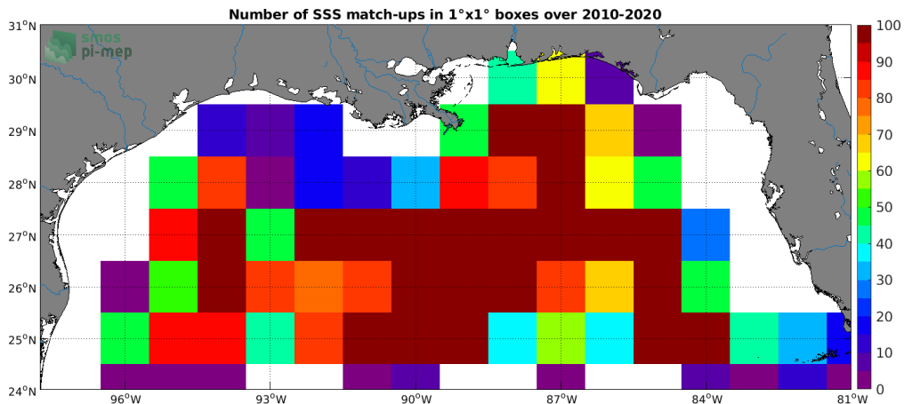
Figure 4: Number of SSS match-ups between Argo SSS and the CCI SSS L4 Merged-OI v3.2 - 30-day running (ESA) SSS product for the Mississippi river plume Pi-MEP region over 1°x1° boxes and for the full satellite product period.
