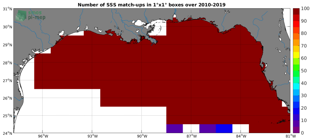
Figure 4: Number of SSS match-ups between TSG (SAMOS) SSS and the CCI SSS L4 Merged-OI v2.31 - 7-day running (ESA) SSS product for the Mississippi river plume Pi-MEP region over 1°x1° boxes and for the full satellite product period.
