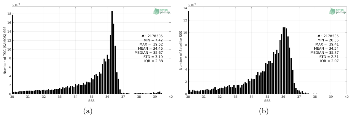
Figure 2: Histograms of SSS from TSG (SAMOS) (a) and CCI SSS L4 Merged-OI v2.31 - 7-day running (ESA) (b) considering all match-up pairs per bins of 0.1 over the Mississippi river plume Pi-MEP region and for the full satellite product period.
