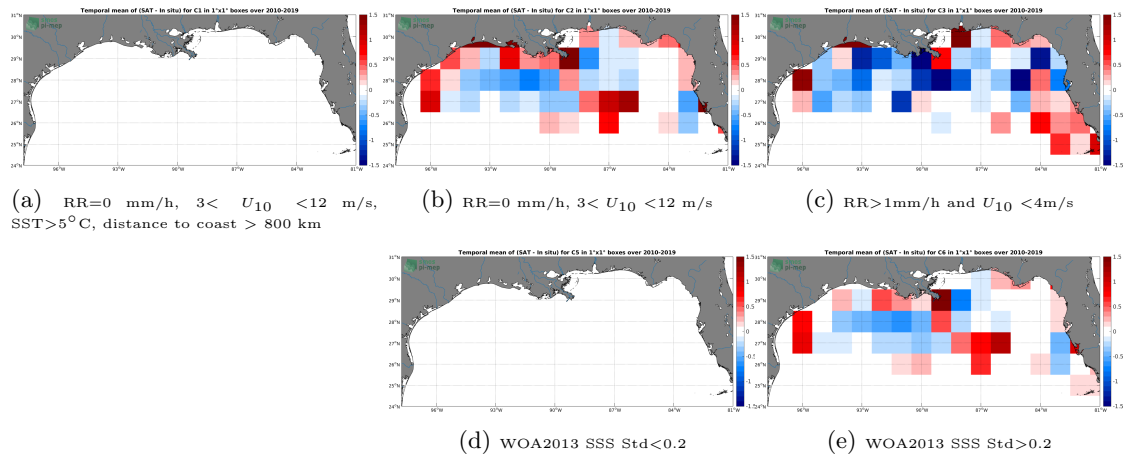
Figure 12: Temporal mean gridded over spatial boxes of size 1^{\circ}\times 1^{\circ} of \Delta\text{SSS} (CCI SSS L4 Merged-OI v2.31 - 7-day running (ESA) - TSG (SAMOS)) for 5 different subdatasets corresponding to:RR=0 mm/h, 3 < U_{10} < 12 m/s, SST >5^{\circ}\text{C} , distance to coast > 800 km (a), RR=0 mm/h, 3 < U_{10} < 12 m/s (b), RR >1 mm/h and U_{10} < 4 m/s (c), WOA2013 SSS Std <0.2 (d), WOA2013 SSS Std >0.2 (e).
