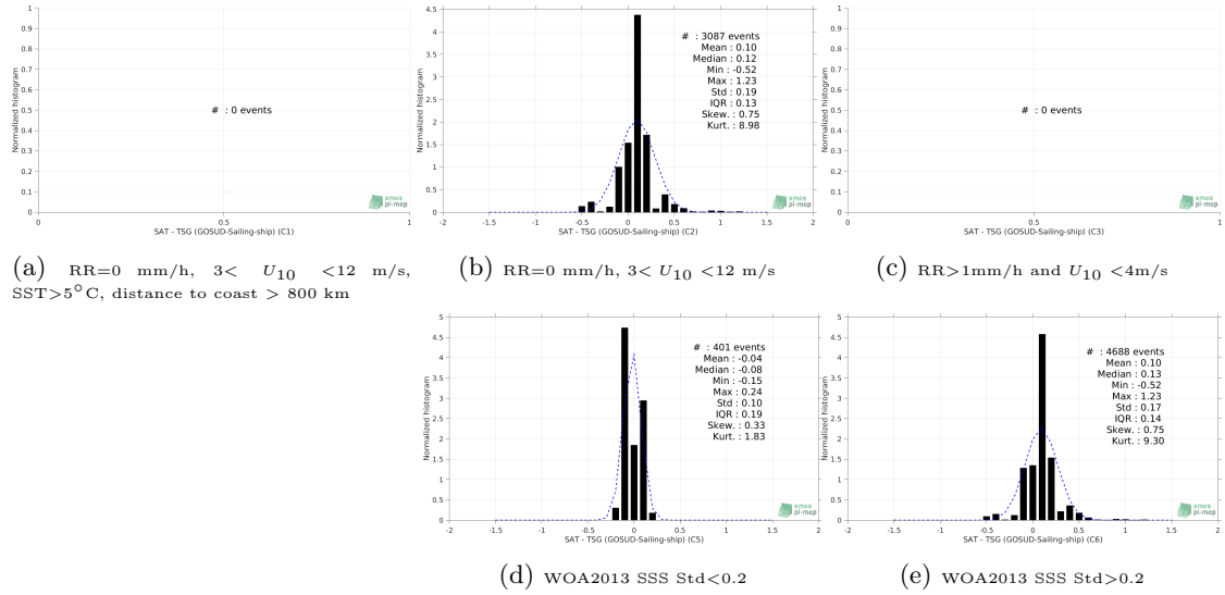
Figure 13: Normalized histogram of \Delta\text{SSS} (CCI SSS L4 Merged-OI v2.31 - 7-day running (ESA) - TSG (GOSUD-Sailing-ship)) for 5 different subdatasets corresponding to: RR=0 mm/h, 3 < U_{10} < 12 m/s, SST > 5^\circ\text{C} , distance to coast > 800 km (a), RR=0 mm/h, 3 < U_{10} < 12 m/s (b), RR > 1\text{mm/h} and U_{10} < 4\text{m/s} (c), WOA2013 SSS \text{Std} < 0.2 (d), WOA2013 SSS \text{Std} > 0.2 (e).
