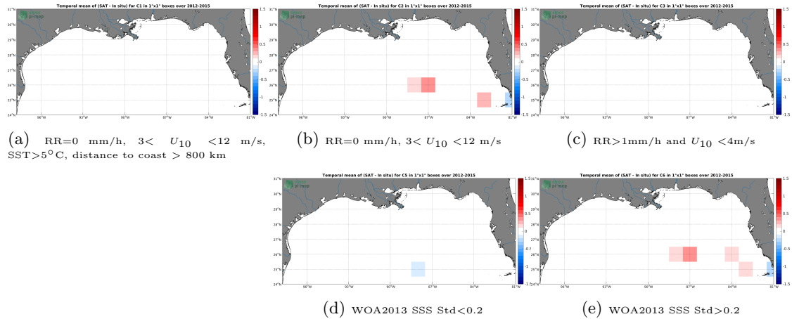
Figure 12: Temporal mean gridded over spatial boxes of size 1^\circ \times 1^\circ of \Delta SSS (CCI SSS L4 Merged-OI v2.31 - 7-day running (ESA) - TSG (GOSUD-Sailing-ship)) for 5 different subdatasets corresponding to: RR=0 mm/h, 3 < U_{10} < 12 m/s, SST > 5^\circ\text{C} , distance to coast > 800 km (a), RR=0 mm/h, 3 < U_{10} < 12 m/s (b), RR > 1 mm/h and U_{10} < 4 m/s (c), WOA2013 SSS Std < 0.2 (d), WOA2013 SSS Std > 0.2 (e).
