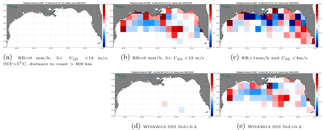
Figure 12: Temporal mean gridded over spatial boxes of size 1^{\circ}\times 1^{\circ} of \Delta\text{SSS} (CCI SSS L4 Merged-OI v2.31 - 30-day running (ESA) - TSG (SAMOS)) for 5 different subdatasets corresponding to:RR=0 mm/h, 3 < U_{10} < 12 m/s, SST >5^{\circ}\text{C} , distance to coast > 800 km (a), RR=0 mm/h, 3 < U_{10} < 12 m/s (b), RR >1 mm/h and U_{10} < 4 m/s (c), WOA2013 SSS Std <0.2 (d), WOA2013 SSS Std >0.2 (e).
