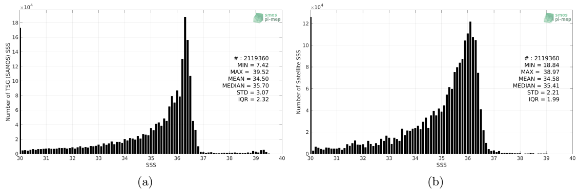
Figure 2: Histograms of SSS from TSG (SAMOS) (a) and CCI SSS L4 Merged-OI v2.31 - 30-day running (ESA) (b) considering all match-up pairs per bins of 0.1 over the Mississippi river plume Pi-MEP region and for the full satellite product period.
