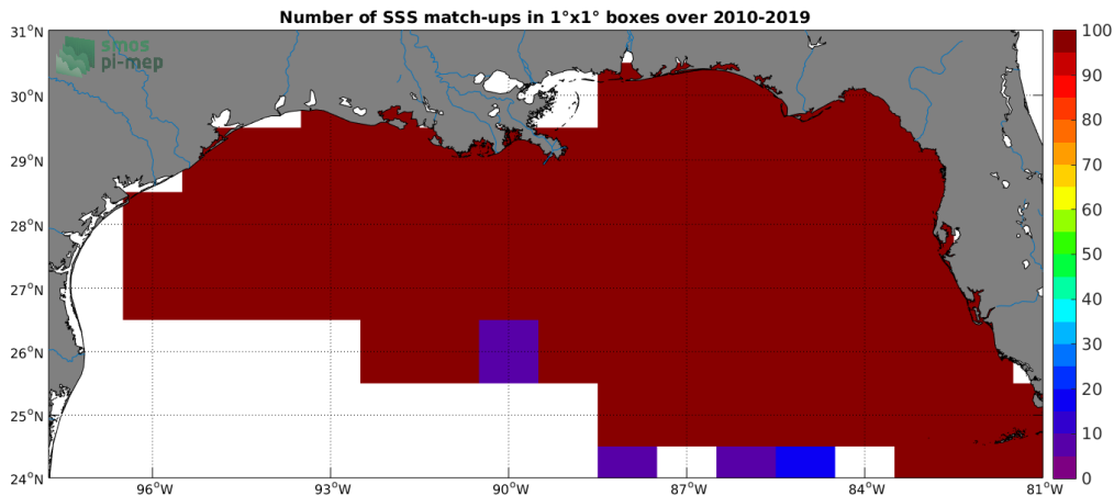
Figure 4: Number of SSS match-ups between TSG (SAMOS) SSS and the CCI SSS L4 Merged-OI v2.31 - 30-day running (ESA) SSS product for the Mississippi river plume Pi-MEP region over 1°x1° boxes and for the full satellite product period.
