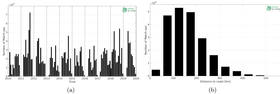
Figure 1: Number of match-ups between TSG (SAMOS) and CCI SSS L4 Merged-OI v2.31 - 30-day running (ESA) SSS as a function of time (a) and as function of the distance to coast (b) over the Mississippi river plume Pi-MEP region and for the full satellite product period.
