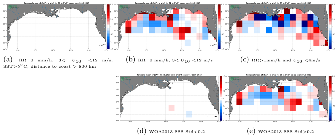
Figure 12: Temporal mean gridded over spatial boxes of size 1^{\circ}\times 1^{\circ} of \Delta\text{SSS} (CCI L4 Merged-OI v2.31 - 30-day running (ESA) - TSG (SAMOS)) for 5 different subdatasets corresponding to:RR=0 mm/h, 3 < U_{10} < 12 m/s, SST >5^{\circ}\text{C} , distance to coast > 800 km (a), RR=0 mm/h, 3 < U_{10} < 12 m/s (b), RR >1 mm/h and U_{10} < 4 m/s (c), WOA2013 SSS Std <0.2 (d), WOA2013 SSS Std >0.2 (e).
