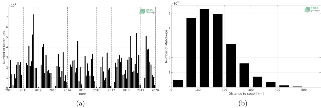
Figure 1: Number of match-ups between TSG (SAMOS) and CCI L4 Merged-OI v2.31 - 30-day running (ESA) SSS as a function of time (a) and as function of the distance to coast (b) over the Mississippi river plume Pi-MEP region and for the full satellite product period.
