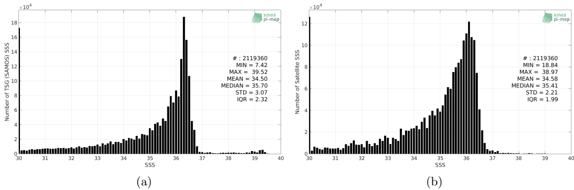
Figure 2: Histograms of SSS from TSG (SAMOS) (a) and CCI L4 Merged-OI v2.31 - 30-day running (ESA) (b) considering all match-up pairs per bins of 0.1 over the Mississippi river plume Pi-MEP region and for the full satellite product period.
