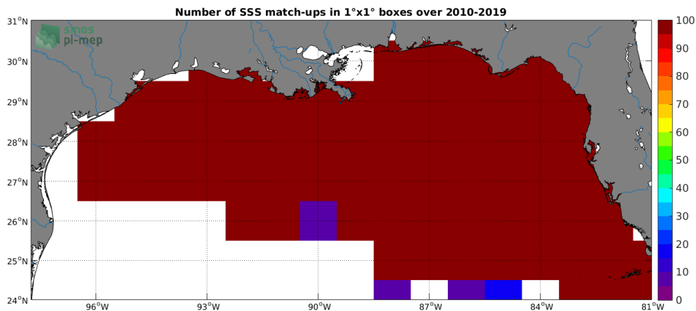
Figure 4: Number of SSS match-ups between TSG (SAMOS) SSS and the CCI L4 Merged-OI v2.31 - 30-day running (ESA) SSS product for the Mississippi river plume Pi-MEP region over 1^\circ \times 1^\circ boxes and for the full satellite product period.
