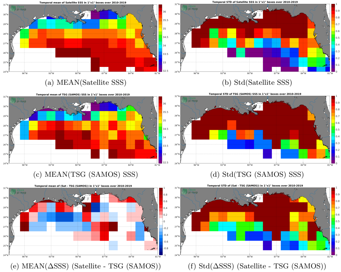
Figure 6: Temporal mean (left) and Std (right) of SSS from CCI L4 Merged-OI v2.31 - 30-day running (ESA) (top), TSG (SAMOS) (middle), and of \Delta SSS (Satellite - TSG (SAMOS)). Only match-up pairs are used to generate these maps.
