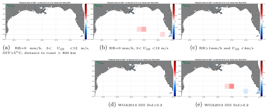
Figure 12: Temporal mean gridded over spatial boxes of size 1^\circ \times 1^\circ of \Delta SSS (CCI L4 Merged-OI v2.31 - 30-day running (ESA) - TSG (GOSUD-Sailing-ship)) for 5 different subdatasets corresponding to: RR=0 mm/h, 3 < U_{10} < 12 m/s, SST > 5^\circ\text{C} , distance to coast > 800 km (a), RR=0 mm/h, 3 < U_{10} < 12 m/s (b), RR > 1 mm/h and U_{10} < 4 m/s (c), WOA2013 SSS Std < 0.2 (d), WOA2013 SSS Std > 0.2 (e).
