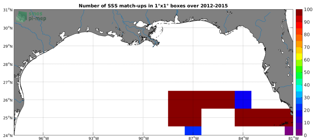
Figure 4: Number of SSS match-ups between TSG (GOSUD-Sailing-ship) SSS and the CCI L4 Merged-OI v2.31 - 30-day running (ESA) SSS product for the Mississippi river plume Pi-MEP region over 1°x1° boxes and for the full satellite product period.
