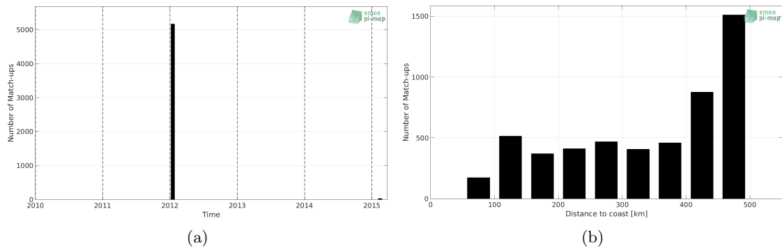
Figure 1: Number of match-ups between TSG (GOSUD-Sailing-ship) and CCI L4 Merged-OI v2.31 - 30-day running (ESA) SSS as a function of time (a) and as function of the distance to coast (b) over the Mississippi river plume Pi-MEP region and for the full satellite product period.
