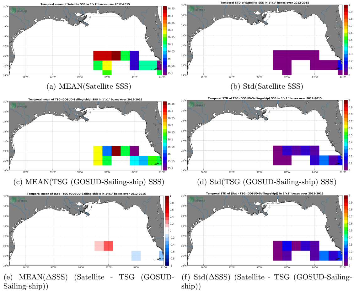
Figure 6: Temporal mean (left) and Std (right) of SSS from CCI L4 Merged-OI v2.31 - 30-day running (ESA) (top), TSG (GOSUD-Sailing-ship) (middle), and of \Delta SSS (Satellite - TSG (GOSUD-Sailing-ship)). Only match-up pairs are used to generate these maps.
