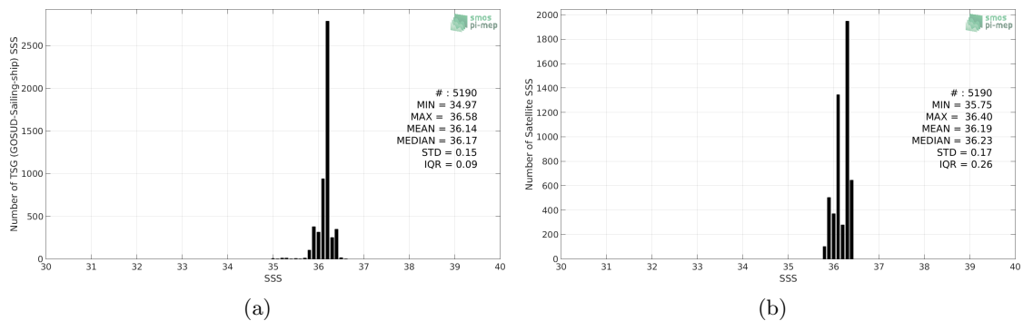
Figure 2: Histograms of SSS from TSG (GOSUD-Sailing-ship) (a) and CCI L4 Merged-OI v2.31 - 30-day running (ESA) (b) considering all match-up pairs per bins of 0.1 over the Mississippi river plume Pi-MEP region and for the full satellite product period.
