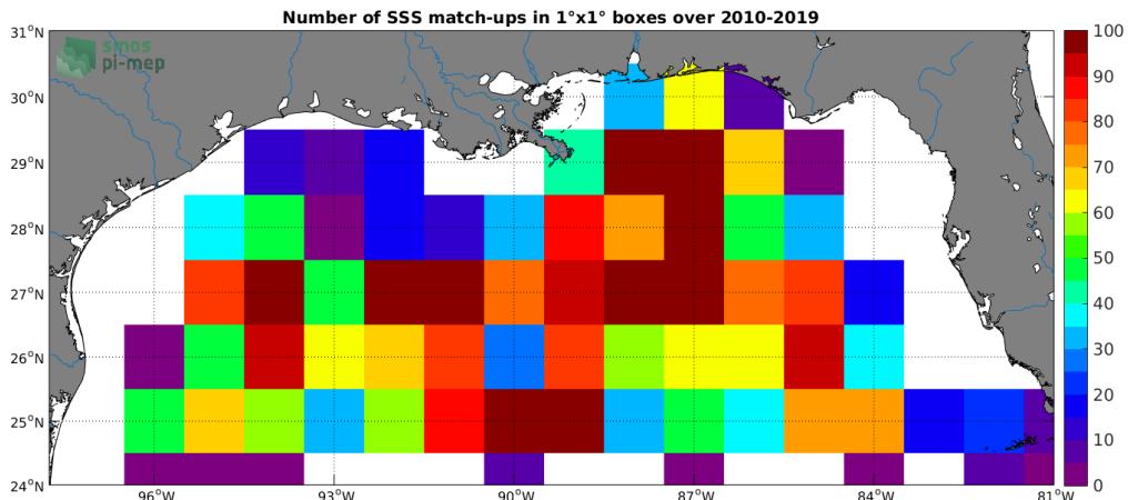
Figure 4: Number of SSS match-ups between Argo SSS and the CCI SSS L4 Merged-OI v2.31 - 30-day running (ESA) SSS product for the Mississippi river plume Pi-MEP region over 1°x1° boxes and for the full satellite product period.
