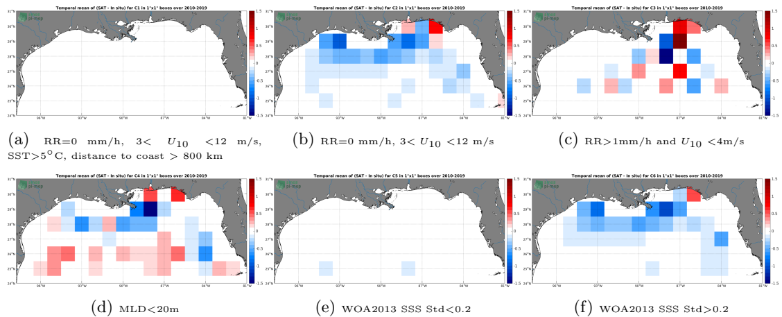
Figure 12: Temporal mean gridded over spatial boxes of size 1^{\circ}\times 1^{\circ} of \Delta\text{SSS} (CCI SSS L4 Merged-OI v2.31 - 30-day running (ESA) - Argo) for 6 different subdatasets corresponding to:RR=0 mm/h, 3 < U_{10} < 12 m/s, SST >5^{\circ}\text{C} , distance to coast > 800 km (a), RR=0 mm/h, 3 < U_{10} < 12 m/s (b), RR >1\text{mm/h} and U_{10} < 4\text{m/s} (c),MLD <20\text{m} (d),WOA2013 SSS Std <0.2 (e),WOA2013 SSS Std >0.2 (f).
