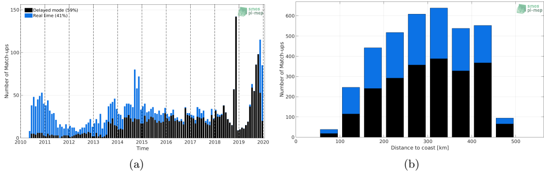
Figure 1: Number of match-ups between Argo and CCI SSS L4 Merged-OI v2.31 - 30-day running (ESA) SSS as a function of time (a) and as function of the distance to coast (b) over the Mississippi river plume Pi-MEP region and for the full satellite product period.
