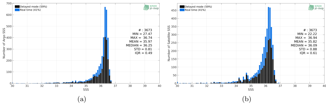
Figure 2: Histograms of SSS from Argo (a) and CCI SSS L4 Merged-OI v2.31 - 30-day running (ESA) (b) considering all match-up pairs per bins of 0.1 over the Mississippi river plume Pi-MEP region and for the full satellite product period.
