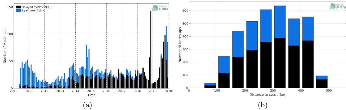
Figure 1: Number of match-ups between Argo and CCI L4 Merged-OI v2.31 - 30-day running (ESA) SSS as a function of time (a) and as function of the distance to coast (b) over the Mississippi river plume Pi-MEP region and for the full satellite product period.
