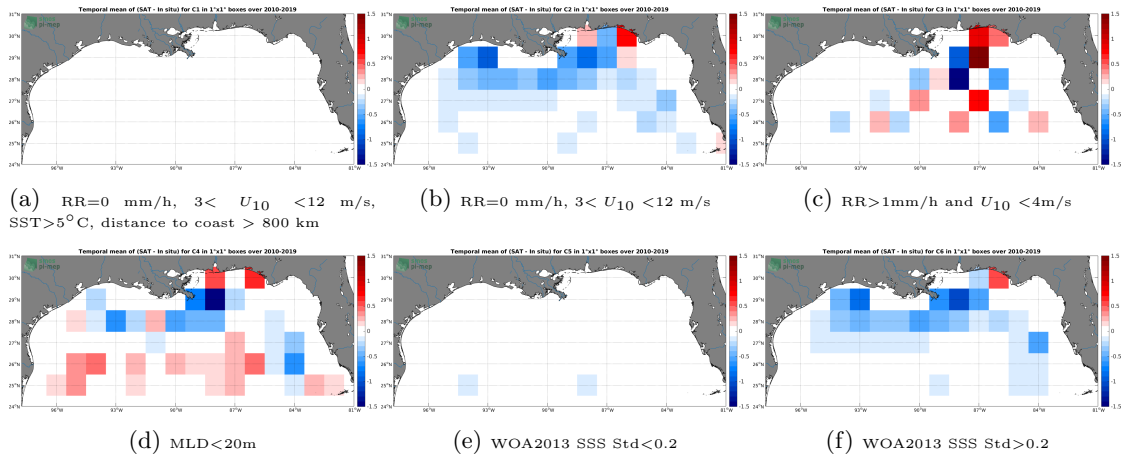
Figure 12: Temporal mean gridded over spatial boxes of size 1^{\circ}\times 1^{\circ} of \Delta\text{SSS} (CCI L4 Merged-OI v2.31 - 30-day running (ESA) - Argo) for 6 different subdatasets corresponding to:RR=0 mm/h, 3 < U_{10} < 12 m/s, \text{SST} > 5^{\circ}\text{C} , distance to coast > 800 km (a), RR=0 mm/h, 3 < U_{10} < 12 m/s (b), RR > 1\text{mm/h} and U_{10} < 4\text{m/s} (c),MLD < 20\text{m} (d),WOA2013 SSS Std < 0.2 (e),WOA2013 SSS Std > 0.2 (f).
