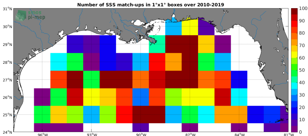
Figure 4: Number of SSS match-ups between Argo SSS and the CCI L4 Merged-OI v2.31 - 30-day running (ESA) SSS product for the Mississippi river plume Pi-MEP region over 1°x1° boxes and for the full satellite product period.
