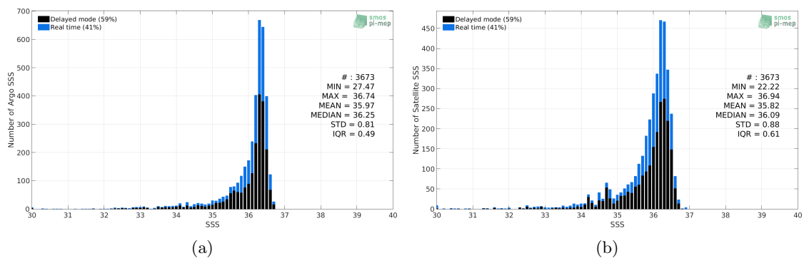
Figure 2: Histograms of SSS from Argo (a) and CCI L4 Merged-OI v2.31 - 30-day running (ESA) (b) considering all match-up pairs per bins of 0.1 over the Mississippi river plume Pi-MEP region and for the full satellite product period.
