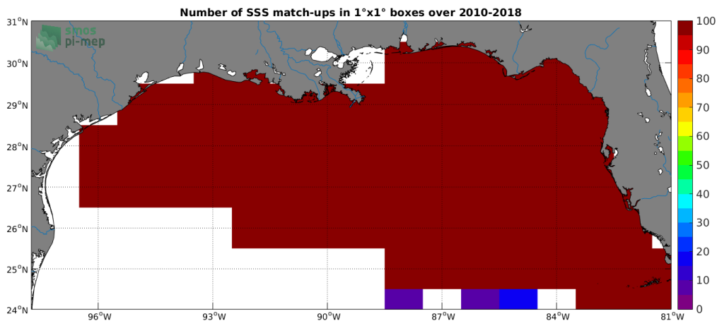
Figure 4: Number of SSS match-ups between TSG-SAMOS SSS and the CCI-L4-ESA-MERGED-OI-V1.8-7DAY-RUNNING SSS product for the Mississippi river plume Pi-MEP region over 1^\circ \times 1^\circ boxes and for the full satellite product period.
