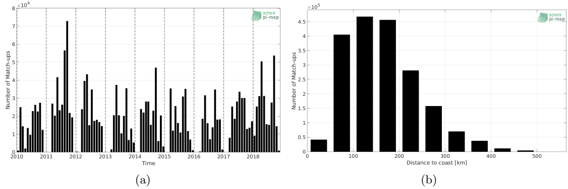
Figure 1: Number of match-ups between TSG-SAMOS and CCI-L4-ESA-MERGED-OI-V1.8-7DAY-RUNNING SSS as a function of time (a) and as function of the distance to coast (b) over the Mississippi river plume Pi-MEP region and for the full satellite product period.
