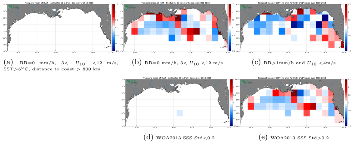
Figure 12: Temporal mean gridded over spatial boxes of size 1^\circ \times 1^\circ of \Delta SSS (CCI-L4-ESAMERGED-OI-V1.8-7DAY-RUNNING - TSG-SAMOS) for 5 different subdatasets corresponding to: RR=0 mm/h, 3 < U_{10} < 12 m/s, SST > 5^\circ\text{C} , distance to coast > 800 km (a), RR=0 mm/h, 3 < U_{10} < 12 m/s (b), RR > 1 mm/h and U_{10} < 4 m/s (c), WOA2013 SSS Std < 0.2 (d), WOA2013 SSS Std > 0.2 (e).
