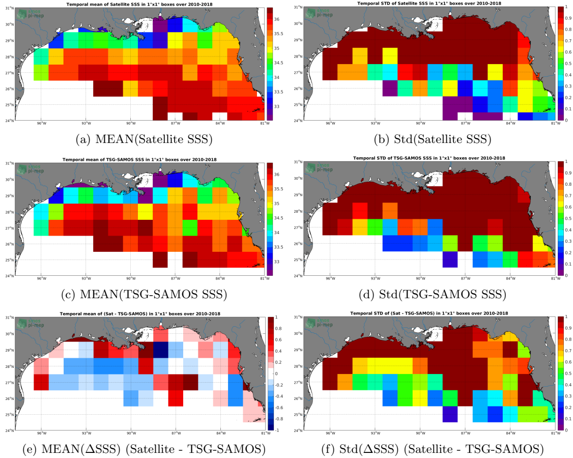
Figure 6: Temporal mean (left) and Std (right) of SSS from CCI-L4-ESA-MERGED-OI-V1.8-7DAY-RUNNING (top), TSG-SAMOS (middle), and of \Delta SSS (Satellite - TSG-SAMOS). Only match-up pairs are used to generate these maps.
