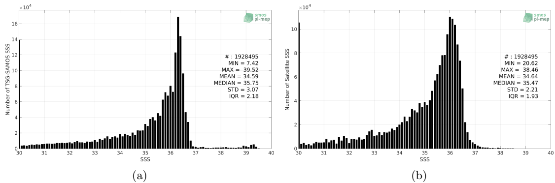
Figure 2: Histograms of SSS from TSG-SAMOS (a) and CCI-L4-ESA-MERGED-OI-V1.8-7DAY-RUNNING (b) considering all match-up pairs per bins of 0.1 over the Mississippi river plume Pi-MEP region and for the full satellite product period.
