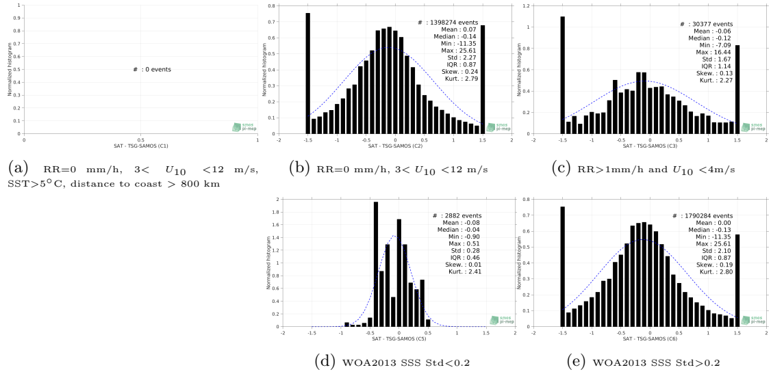
Figure 13: Normalized histogram of \Delta SSS (CCI-L4-ESA-MERGED-OI-V1.8-7DAY-RUNNING - TSG-SAMOS) for 5 different subdatasets corresponding to: RR=0 mm/h, 3 < U_{10} < 12 m/s, SST > 5°C, distance to coast > 800 km (a), RR=0 mm/h, 3 < U_{10} < 12 m/s (b), RR > 1mm/h and U_{10} < 4 m/s (c), WOA2013 SSS Std < 0.2 (d), WOA2013 SSS Std > 0.2 (e).
