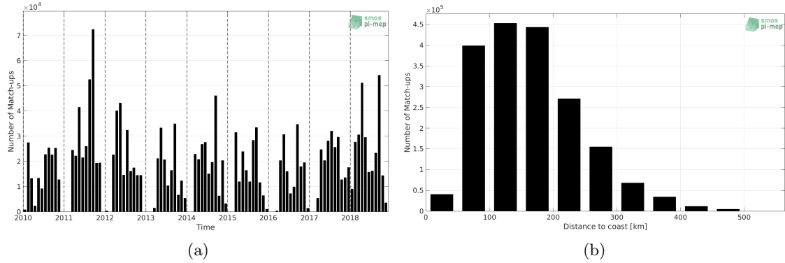
Figure 1: Number of match-ups between TSG-SAMOS and CCI L4 Merged-OI v1.8 - 30-day running (ESA) SSS as a function of time (a) and as function of the distance to coast (b) over the Mississippi river plume Pi-MEP region and for the full satellite product period.
