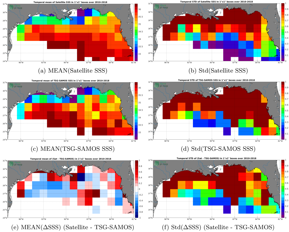
Figure 6: Temporal mean (left) and Std (right) of SSS from CCI L4 Merged-OI v1.8 - 30-day running (ESA) (top), TSG-SAMOS (middle), and of \Delta SSS (Satellite - TSG-SAMOS). Only match-up pairs are used to generate these maps.
