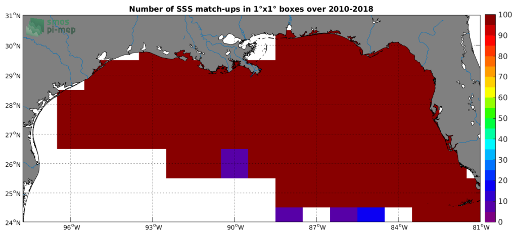
Figure 4: Number of SSS match-ups between TSG-SAMOS SSS and the CCI L4 Merged-OI v1.8 - 30-day running (ESA) SSS product for the Mississippi river plume Pi-MEP region over 1°x1° boxes and for the full satellite product period.
