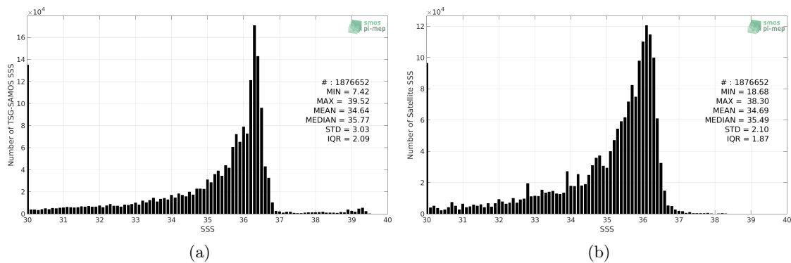
Figure 2: Histograms of SSS from TSG-SAMOS (a) and CCI L4 Merged-OI v1.8 - 30-day running (ESA) (b) considering all match-up pairs per bins of 0.1 over the Mississippi river plume Pi-MEP region and for the full satellite product period.
