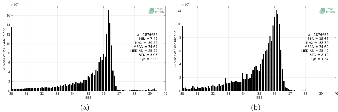
Figure 2: Histograms of SSS from TSG-SAMOS (a) and CCI-L4-ESA-MERGED-OI-V1.8-30DAY-RUNNING (b) considering all match-up pairs per bins of 0.1 over the Mississippi river plume Pi-MEP region and for the full satellite product period.
