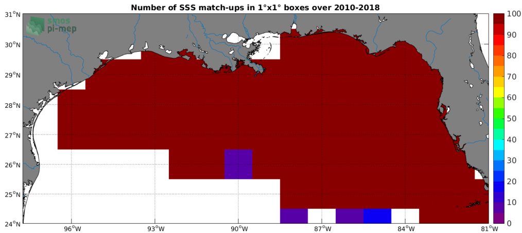
Figure 4: Number of SSS match-ups between TSG-SAMOS SSS and the CCI-L4-ESA-MERGED-OI-V1.8-30DAY-RUNNING SSS product for the Mississippi river plume Pi-MEP region over 1^\circ \times 1^\circ boxes and for the full satellite product period.
