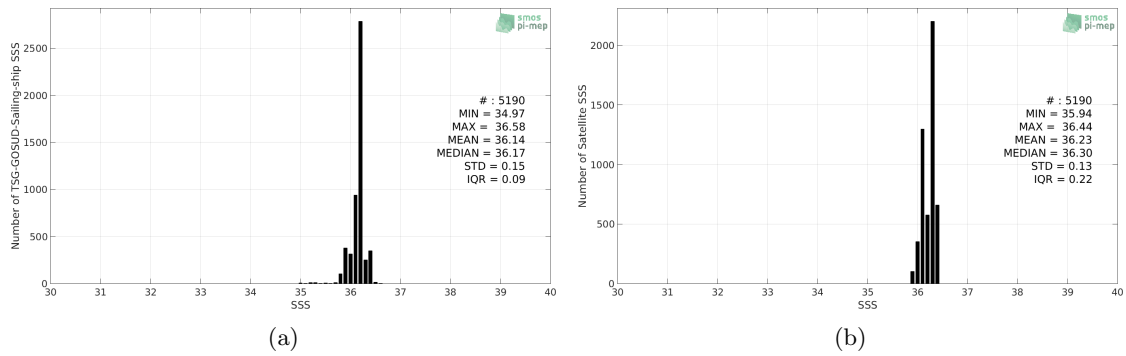
Figure 2: Histograms of SSS from TSG-GOSUD-Sailing-ship (a) and CCI-L4-ESA-MERGED-OI-V1.8-30DAY-RUNNING (b) considering all match-up pairs per bins of 0.1 over the Mississippi river plume Pi-MEP region and for the full satellite product period.
