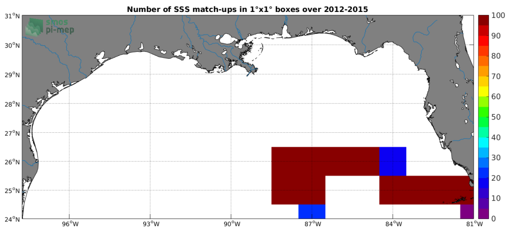
Figure 4: Number of SSS match-ups between TSG-GOSUD-Sailing-ship SSS and the CCI-L4-ESA-MERGED-OI-V1.8-30DAY-RUNNING SSS product for the Mississippi river plume Pi-MEP region over 1^\circ \times 1^\circ boxes and for the full satellite product period.
