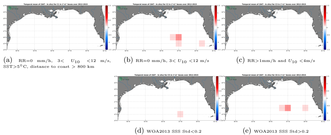
Figure 12: Temporal mean gridded over spatial boxes of size 1^\circ \times 1^\circ of \Delta SSS (CCI-L4-ESAMERGED-OI-V1.8-30DAY-RUNNING - TSG-GOSUD-Sailing-ship) for 5 different subdatasets corresponding to: RR=0 mm/h, 3 < U_{10} < 12 m/s, SST > 5°C, distance to coast > 800 km (a), RR=0 mm/h, 3 < U_{10} < 12 m/s (b), RR > 1mm/h and U_{10} < 4 m/s (c), WOA2013 SSS Std < 0.2 (d), WOA2013 SSS Std > 0.2 (e).
