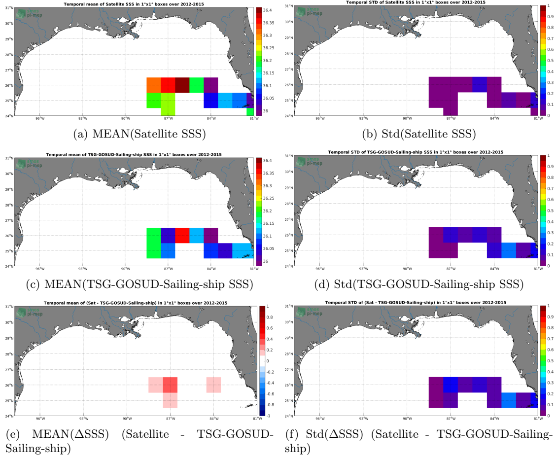
Figure 6: Temporal mean (left) and Std (right) of SSS from CCI-L4-ESA-MERGED-OI-V1.8-30DAY-RUNNING (top), TSG-GOSUD-Sailing-ship (middle), and of \Delta SSS (Satellite - TSG-GOSUD-Sailing-ship). Only match-up pairs are used to generate these maps.
