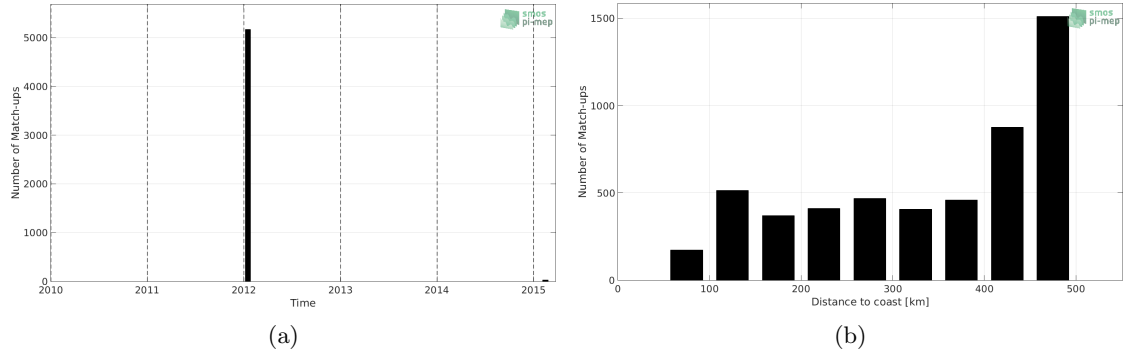
Figure 1: Number of match-ups between TSG-GOSUD-Sailing-ship and CCI-L4-ESA-MERGED-OI-V1.8-30DAY-RUNNING SSS as a function of time (a) and as function of the distance to coast (b) over the Mississippi river plume Pi-MEP region and for the full satellite product period.
