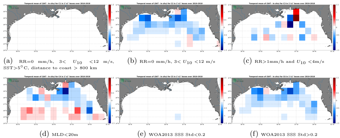
Figure 12: Temporal mean gridded over spatial boxes of size 1^{\circ}\times 1^{\circ} of \Delta\text{SSS} (CCI L4 Merged-OI v1.8 - 30-day running (ESA) - Argo) for 6 different subdatasets corresponding to: \text{RR}=0 mm/h, 3 < U_{10} < 12 m/s, \text{SST} > 5^{\circ}\text{C} , distance to coast > 800 km (a), \text{RR}=0 mm/h, 3 < U_{10} < 12 m/s (b), \text{RR} > 1 mm/h and U_{10} < 4 m/s (c), \text{MLD} < 20\text{m} (d), WOA2013 SSS Std < 0.2 (e), WOA2013 SSS Std > 0.2 (f).
