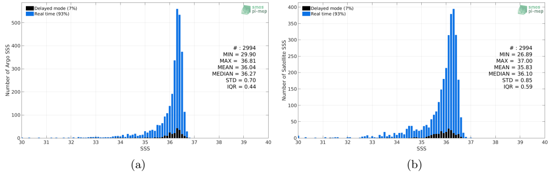
Figure 2: Histograms of SSS from Argo (a) and CCI L4 Merged-OI v1.8 - 30-day running (ESA) (b) considering all match-up pairs per bins of 0.1 over the Mississippi river plume Pi-MEP region and for the full satellite product period.
