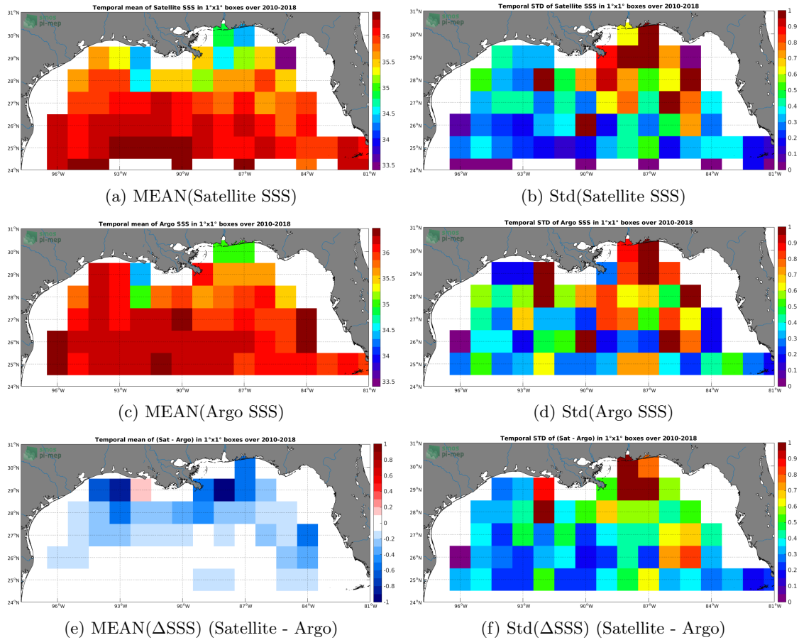
Figure 6: Temporal mean (left) and Std (right) of SSS from CCI L4 Merged-OI v1.8 - 30-day running (ESA) (top), Argo (middle), and of \Delta SSS (Satellite - Argo). Only match-up pairs are used to generate these maps.
