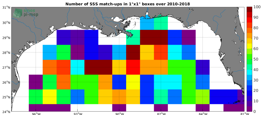
Figure 4: Number of SSS match-ups between Argo SSS and the CCI L4 Merged-OI v1.8 - 30-day running (ESA) SSS product for the Mississippi river plume Pi-MEP region over 1^\circ \times 1^\circ boxes and for the full satellite product period.
