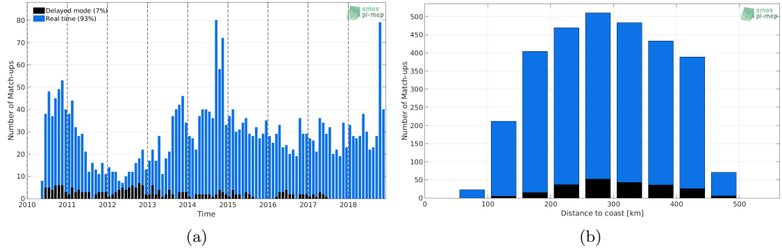
Figure 1: Number of match-ups between Argo and CCI L4 Merged-OI v1.8 - 30-day running (ESA) SSS as a function of time (a) and as function of the distance to coast (b) over the Mississippi river plume Pi-MEP region and for the full satellite product period.
