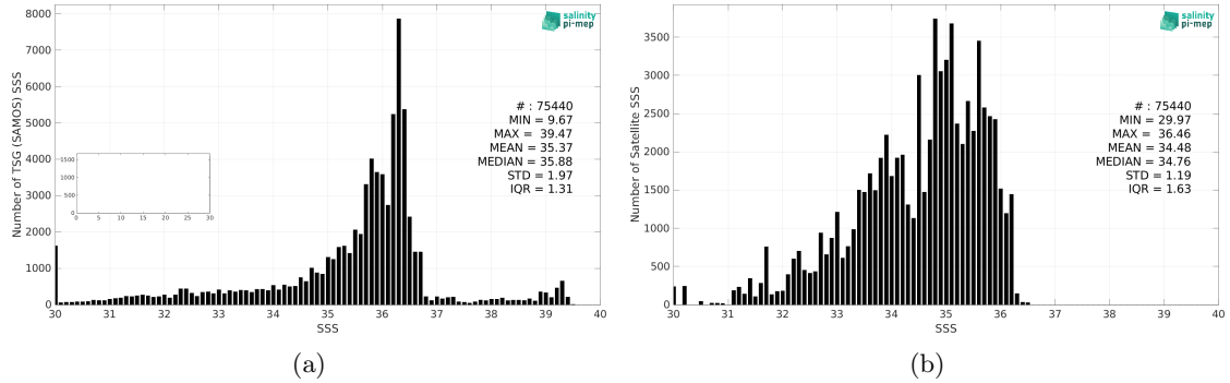
Figure 2: Histograms of SSS from TSG (SAMOS) (a) and Aquarius SSS L4 OI v5 - Weekly (IPRC) (b) considering all match-up pairs per bins of 0.1 over the Mississippi river plume Pi-MEP region and for the full satellite product period.
