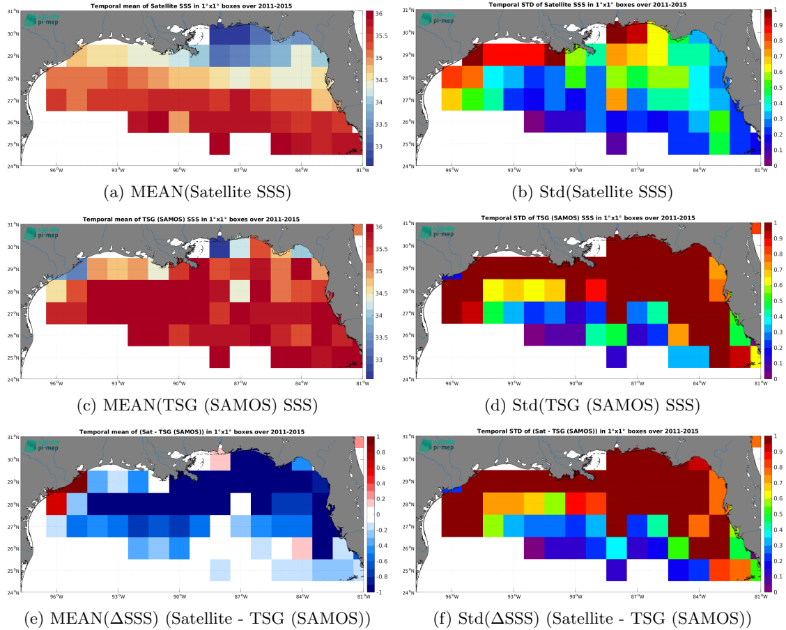
Figure 6: Temporal mean (left) and Std (right) of SSS from Aquarius SSS L4 OI v5 - Weekly (IPRC) (top), TSG (SAMOS) (middle), and of \Delta\text{SSS} (Satellite - TSG (SAMOS)). Only match-up pairs are used to generate these maps.
