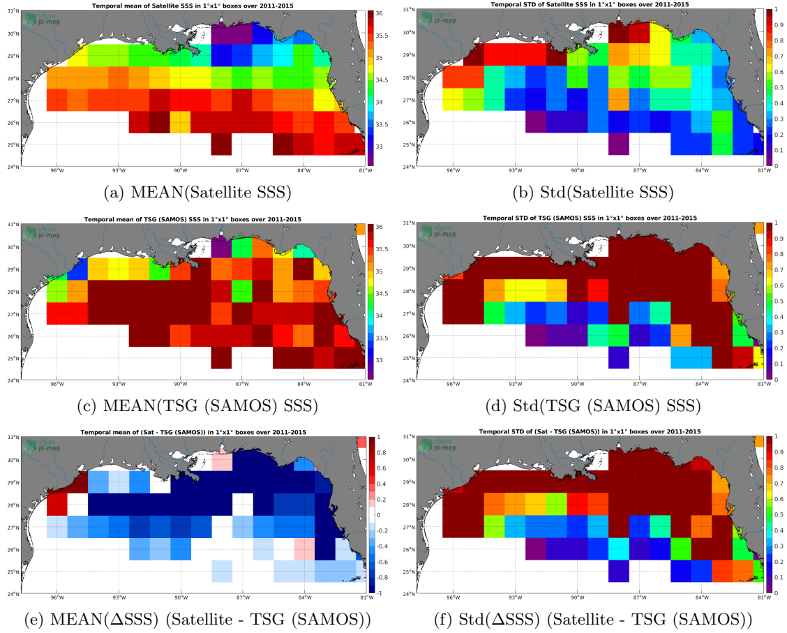
Figure 6: Temporal mean (left) and Std (right) of SSS from Aquarius SSS L4 OI v5 - Weekly (IPRC) (top), TSG (SAMOS) (middle), and of \Delta SSS (Satellite - TSG (SAMOS)). Only match-up pairs are used to generate these maps.
