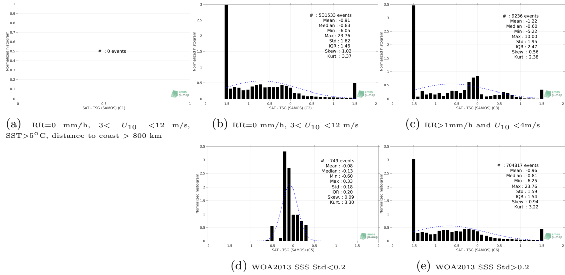
Figure 13: Normalized histogram of \Delta\text{SSS} (Aquarius SSS L4 OI v5 - Weekly (IPRC) - TSG (SAMOS)) for 5 different subdatasets corresponding to: RR=0 mm/h, 3 < U_{10} < 12 m/s, SST > 5^{\circ}\text{C} , distance to coast > 800 km (a), RR=0 mm/h, 3 < U_{10} < 12 m/s (b), RR > 1\text{mm/h} and U_{10} < 4\text{m/s} (c), WOA2013 SSS Std < 0.2 (d), WOA2013 SSS Std > 0.2 (e).
