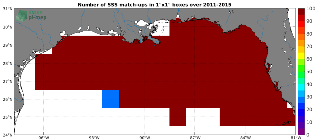
Figure 4: Number of SSS match-ups between TSG (SAMOS) SSS and the Aquarius SSS L4 OI v5 - Weekly (IPRC) SSS product for the Mississippi river plume Pi-MEP region over 1°x1° boxes and for the full satellite product period.
