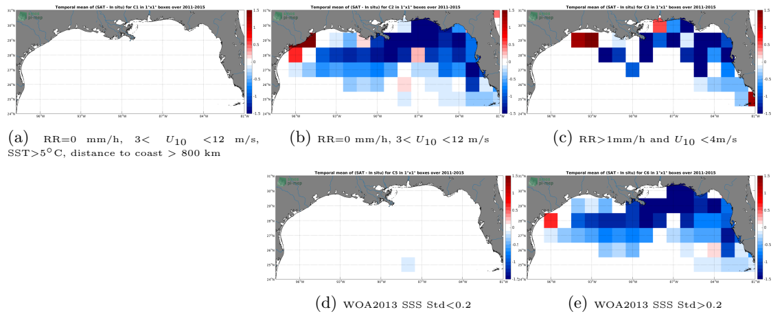
Figure 12: Temporal mean gridded over spatial boxes of size 1^{\circ}\times 1^{\circ} of \Delta\text{SSS} (Aquarius-L4-IPRC-V5-WEEKLY - TSG-SAMOS) for 5 different subdatasets corresponding to:RR=0 mm/h, 3 < U_{10} < 12 m/s, SST >5^{\circ}\text{C} , distance to coast > 800 km (a), RR=0 mm/h, 3 < U_{10} < 12 m/s (b), RR >1 mm/h and U_{10} < 4 m/s (c), WOA2013 SSS Std <0.2 (d), WOA2013 SSS Std >0.2 (e).
