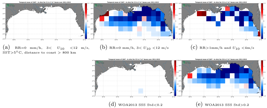
Figure 12: Temporal mean gridded over spatial boxes of size 1^\circ \times 1^\circ of \Delta SSS (Aquarius-L4-IPRC-V5-WEEKLY - TSG-SAMOS) for 5 different subdatasets corresponding to:RR=0 mm/h, 3 < U_{10} < 12 m/s, SST > 5^\circ\text{C} , distance to coast > 800 km (a), RR=0 mm/h, 3 < U_{10} < 12 m/s (b), RR > 1 mm/h and U_{10} < 4 m/s (c), WOA2013 SSS Std < 0.2 (d), WOA2013 SSS Std > 0.2 (e).
