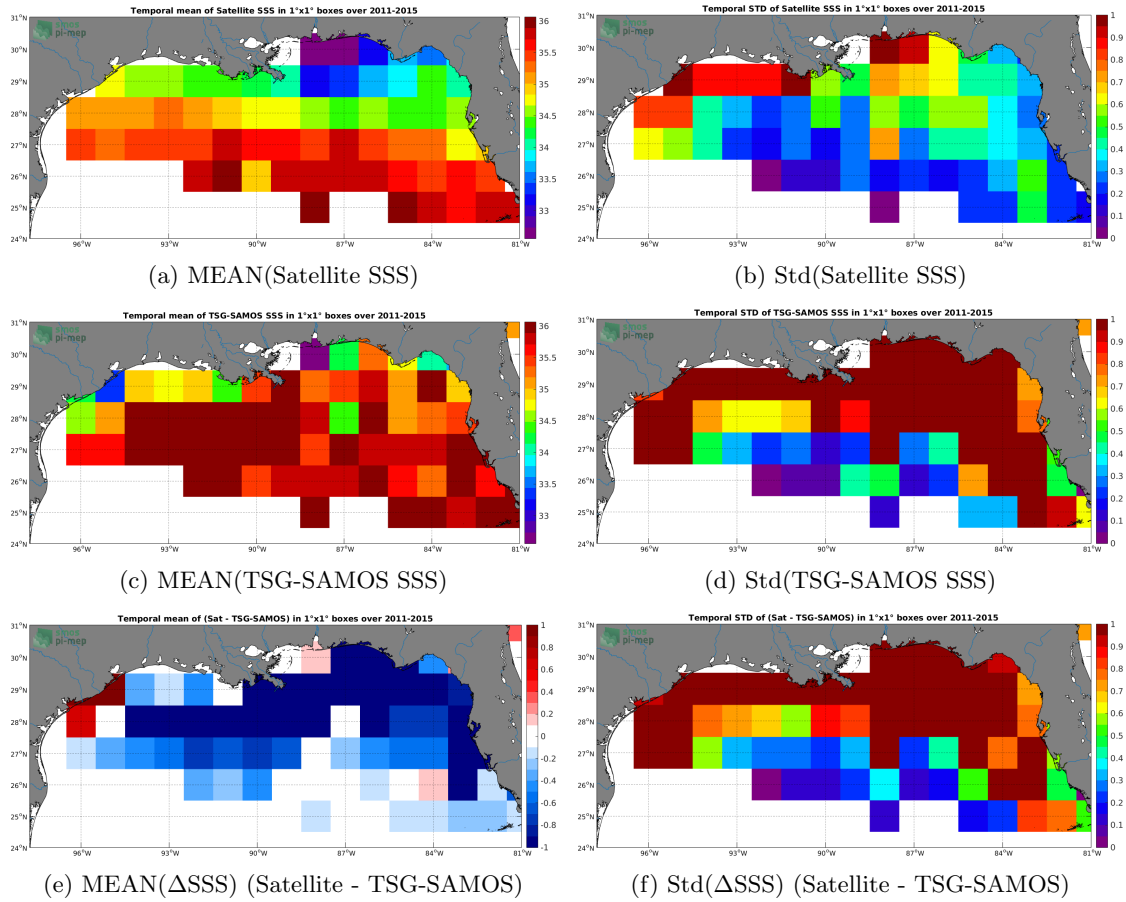
Figure 6: Temporal mean (left) and Std (right) of SSS from Aquarius-L4-IPRC-V5-WEEKLY (top), TSG-SAMOS (middle), and of \Delta SSS (Satellite - TSG-SAMOS). Only match-up pairs are used to generate these maps.
