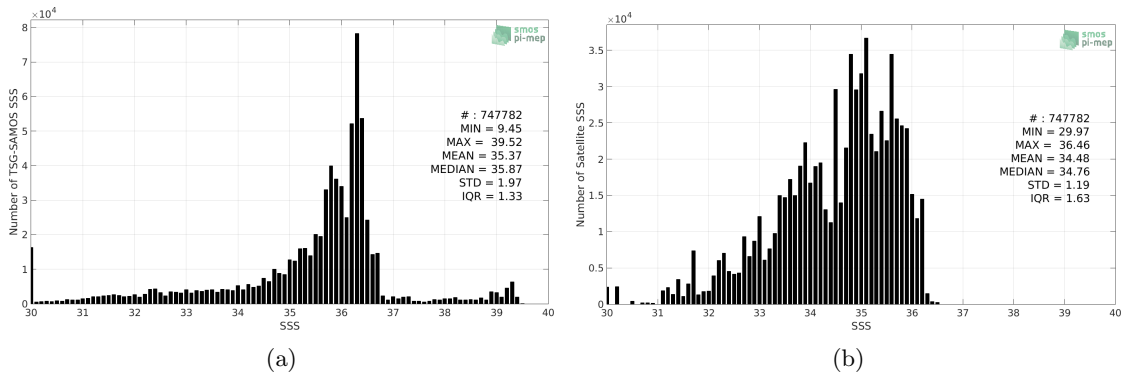
Figure 2: Histograms of SSS from TSG-SAMOS (a) and Aquarius-L4-IPRC-V5-WEEKLY (b) considering all match-up pairs per bins of 0.1 over the Mississippi river plume Pi-MEP region and for the full satellite product period.
