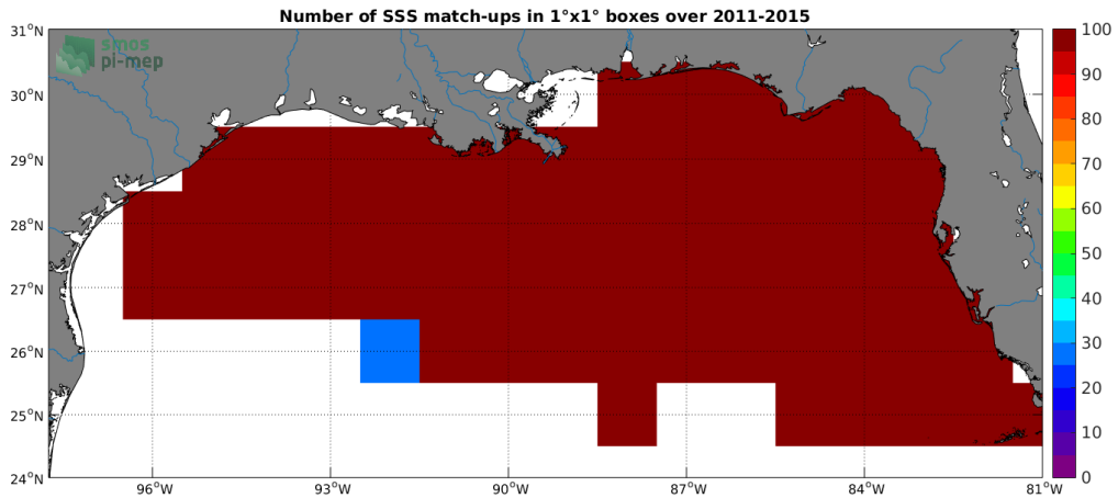
Figure 4: Number of SSS match-ups between TSG-SAMOS SSS and the Aquarius-L4-IPRC-V5-WEEKLY SSS product for the Mississippi river plume Pi-MEP region over 1°x1° boxes and for the full satellite product period.
