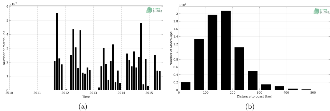
Figure 1: Number of match-ups between TSG-SAMOS and Aquarius-L4-IPRC-V5-WEEKLY SSS as a function of time (a) and as function of the distance to coast (b) over the Mississippi river plume Pi-MEP region and for the full satellite product period.
