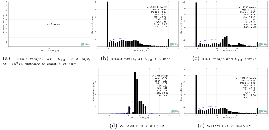
Figure 13: Normalized histogram of \Delta SSS (Aquarius-L4-IPRC-V5-WEEKLY - TSG-SAMOS) for 5 different subdatasets corresponding to: RR=0 mm/h, 3 < U_{10} < 12 m/s, SST > 5°C, distance to coast > 800 km (a), RR=0 mm/h, 3 < U_{10} < 12 m/s (b), RR > 1mm/h and U_{10} < 4 m/s (c), WOA2013 SSS Std < 0.2 (d), WOA2013 SSS Std > 0.2 (e).
