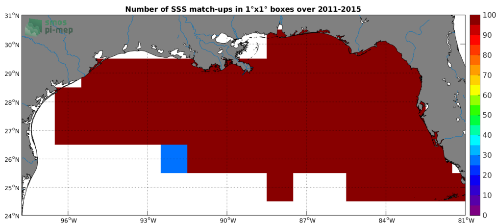
Figure 4: Number of SSS match-ups between TSG-SAMOS SSS and the Aquarius-L4-IPRC-V5-WEEKLY SSS product for the Mississippi river plume Pi-MEP region over 1^\circ \times 1^\circ boxes and for the full satellite product period.
