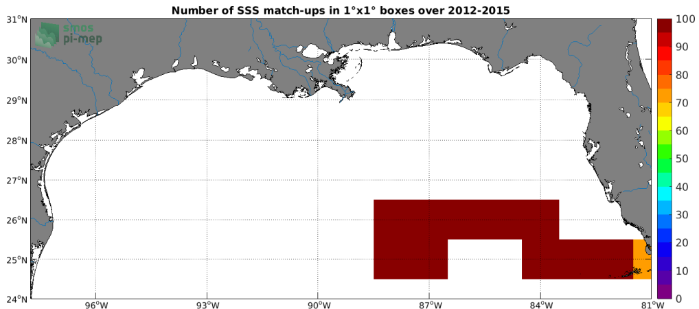
Figure 4: Number of SSS match-ups between TSG (GOSUD-Sailing-ship) SSS and the Aquarius SSS L4 OI v5 - Weekly (IPRC) SSS product for the Mississippi river plume Pi-MEP region over 1°x1° boxes and for the full satellite product period.
