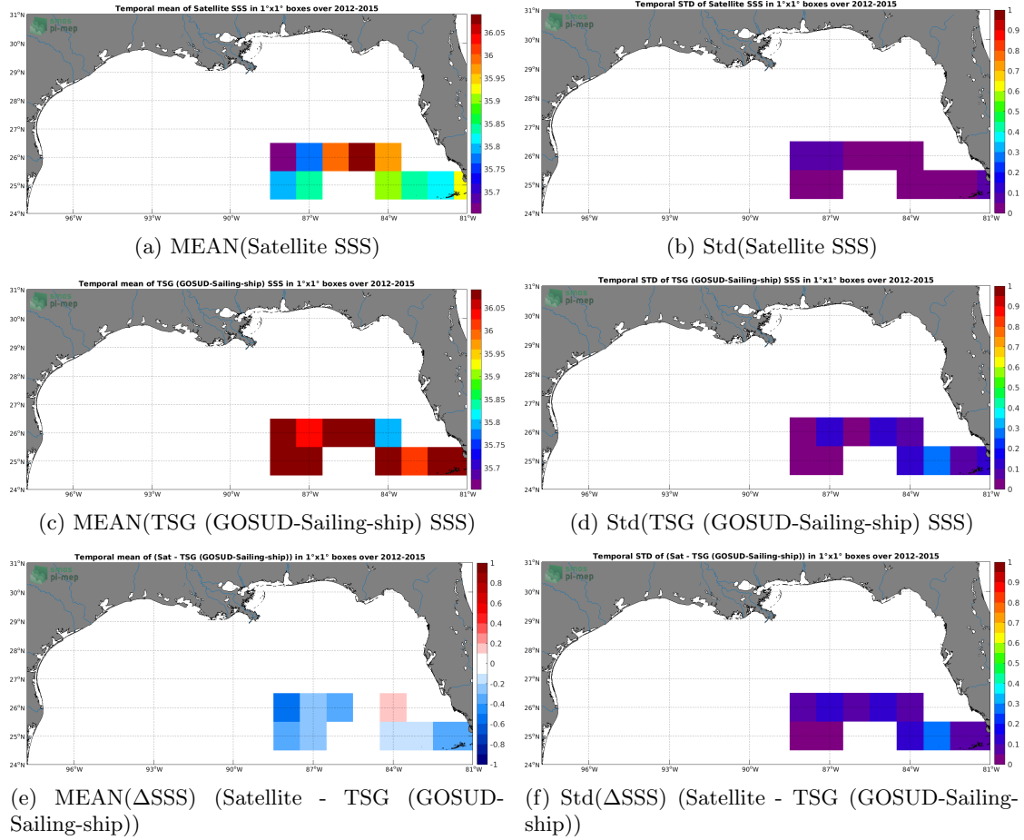
Figure 6: Temporal mean (left) and Std (right) of SSS from Aquarius SSS L4 OI v5 - Weekly (IPRC) (top), TSG (GOSUD-Sailing-ship) (middle), and of \Delta SSS (Satellite - TSG (GOSUD-Sailing-ship)). Only match-up pairs are used to generate these maps.
