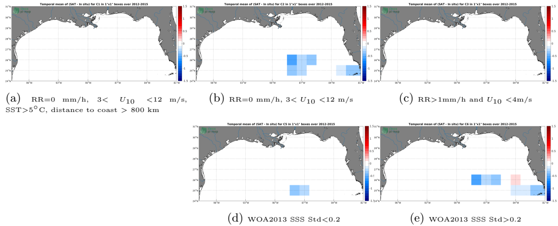
Figure 12: Temporal mean gridded over spatial boxes of size 1^{\circ}\times 1^{\circ} of \Delta SSS (Aquarius-L4-IPRC-V5-WEEKLY - TSG-GOSUD-Sailing-ship) for 5 different subdatasets corresponding to:RR=0 mm/h, 3 < U_{10} < 12 m/s, SST >5^{\circ}\text{C} , distance to coast > 800 km (a), RR=0 mm/h, 3 < U_{10} < 12 m/s (b), RR >1 mm/h and U_{10} < 4 m/s (c), WOA2013 SSS Std <0.2 (d), WOA2013 SSS Std >0.2 (e).
