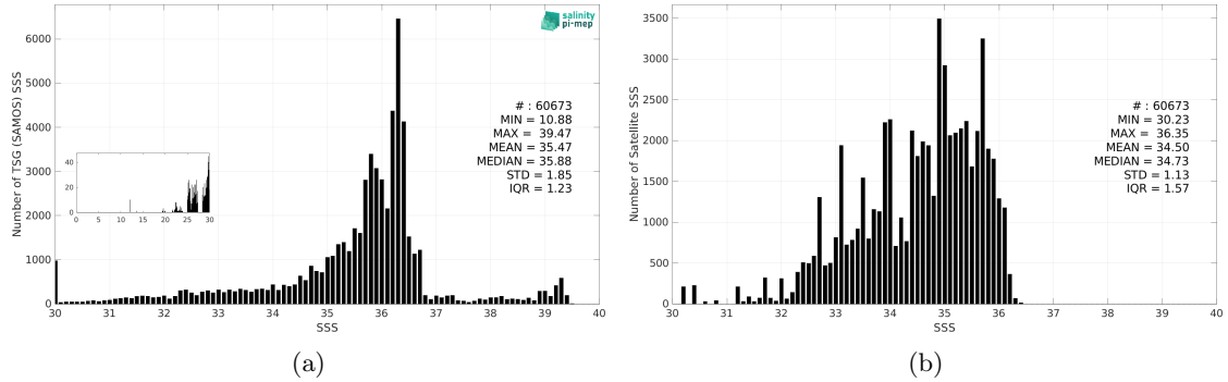
Figure 3: Histograms of SSS from TSG (SAMOS) (a) and Aquarius SSS L4 OI v5 - Monthly (IPRC) (b) considering all match-up pairs per bins of 0.1 over the Mississippi river plume Pi-MEP region and for the full satellite product period.
