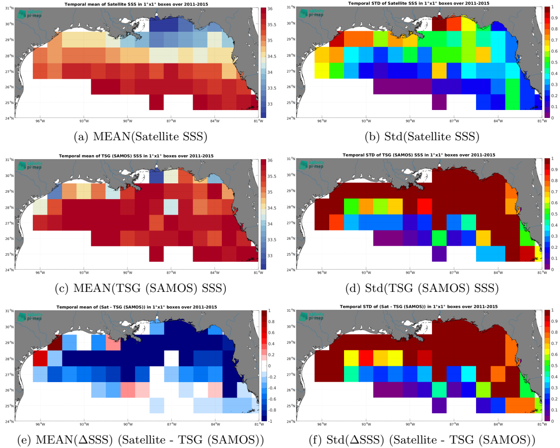
Figure 7: Temporal mean (left) and Std (right) of SSS from Aquarius SSS L4 OI v5 - Monthly (IPRC) (top), TSG (SAMOS) (middle), and of \Delta\text{SSS} (Satellite - TSG (SAMOS)). Only match-up pairs are used to generate these maps.
