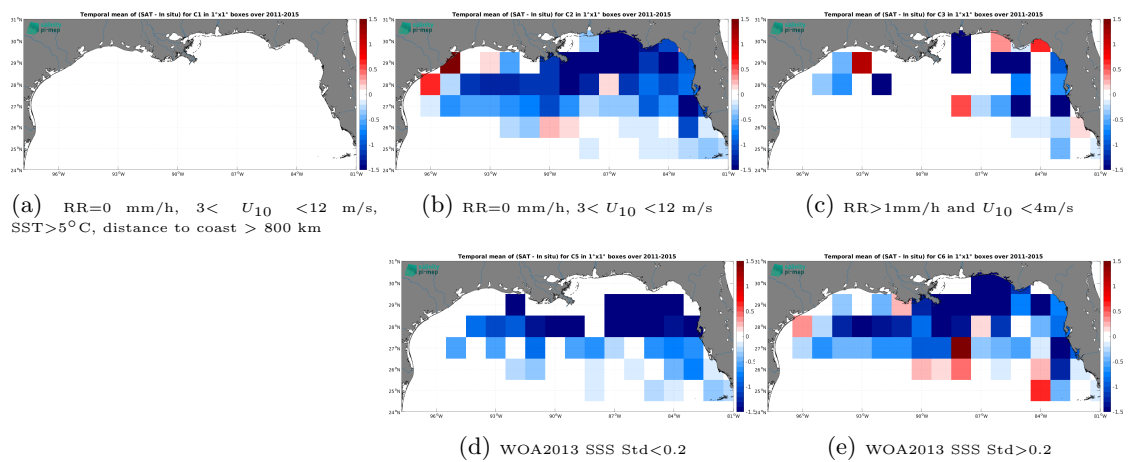
Figure 14: Temporal mean gridded over spatial boxes of size 1^\circ \times 1^\circ of \Delta SSS (Aquarius SSS L4 OI v5 - Monthly (IPRC) - TSG (SAMOS)) for 5 different subdatasets corresponding to:RR=0 mm/h, 3 < U_{10} < 12 m/s, SST > 5^\circ C , distance to coast > 800 km (a), RR=0 mm/h, 3 < U_{10} < 12 m/s (b), RR>1mm/h and U_{10} < 4m/s (c), WOA2013 SSS Std<0.2 (d), WOA2013 SSS Std>0.2 (e).
