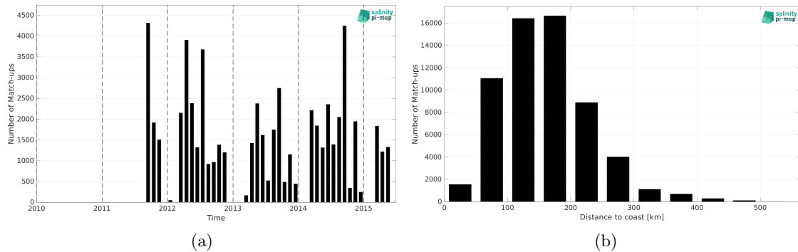
Figure 2: Number of match-ups between TSG (SAMOS) and Aquarius SSS L4 OI v5 - Monthly (IPRC) SSS as a function of time (a) and as function of the distance to coast (b) over the Mississippi river plume Pi-MEP region and for the full satellite product period.
