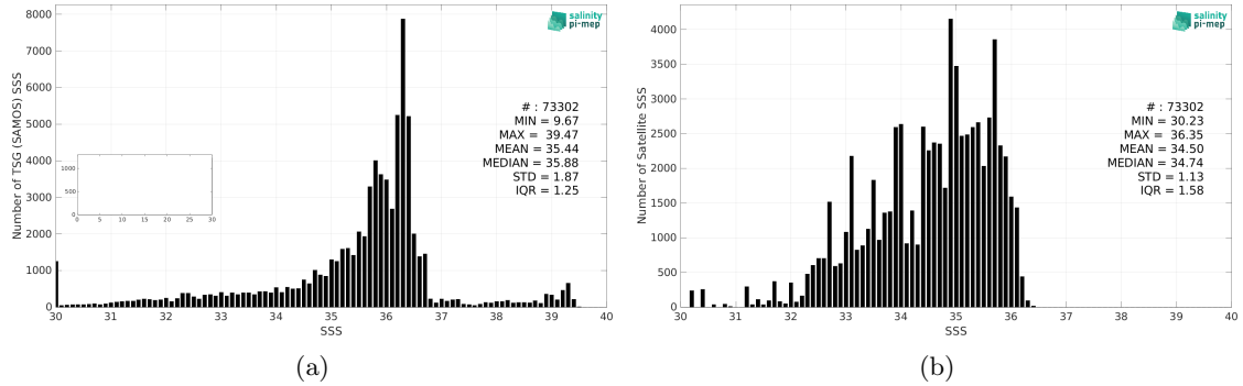
Figure 2: Histograms of SSS from TSG (SAMOS) (a) and Aquarius SSS L4 OI v5 - Monthly (IPRC) (b) considering all match-up pairs per bins of 0.1 over the Mississippi river plume Pi-MEP region and for the full satellite product period.
